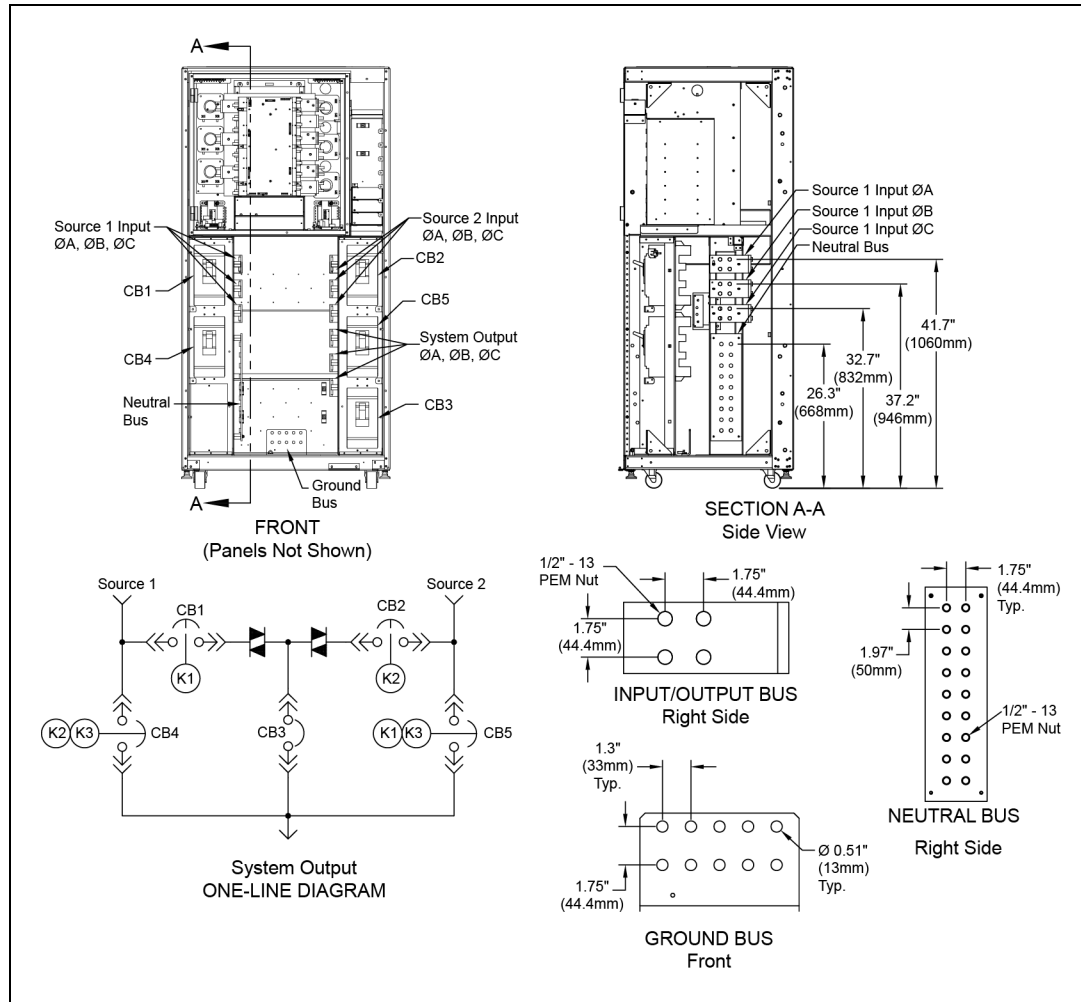
Figure 7.12 Electrical Field Connections Drawing: 400 – 600 Amp Vertiv™ Liebert® STS2 with Single Output Breaker
