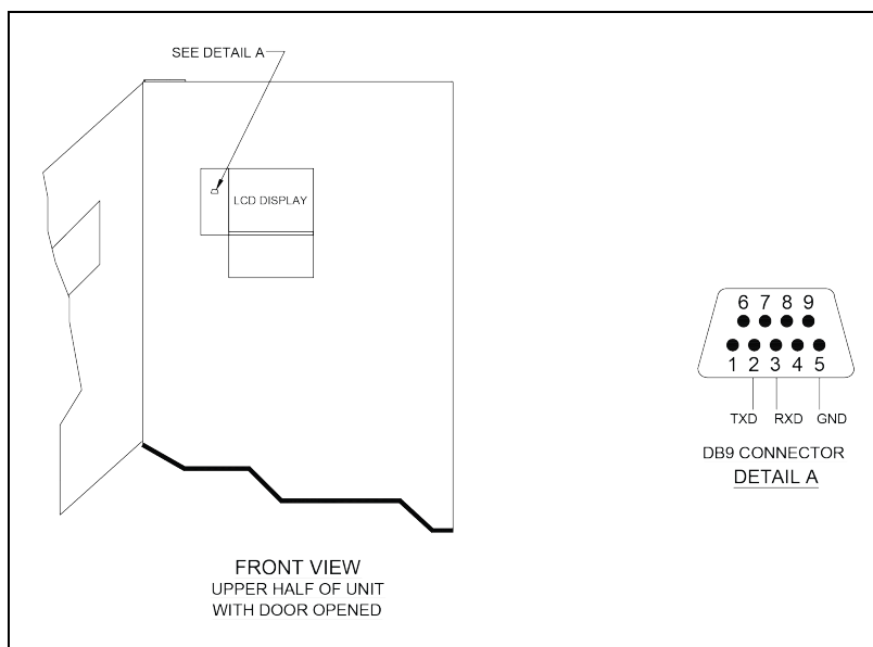
Figure 7.23 Control Wiring for the RS-232 Port
