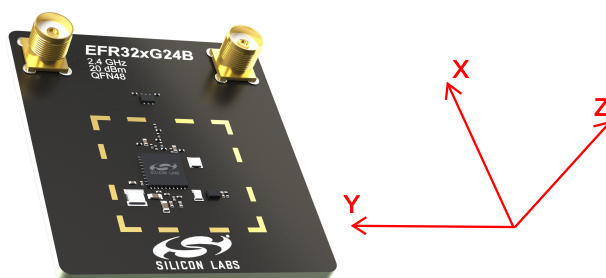
Figure 7.2. Illustration of Reference Planes with a Radio Board
