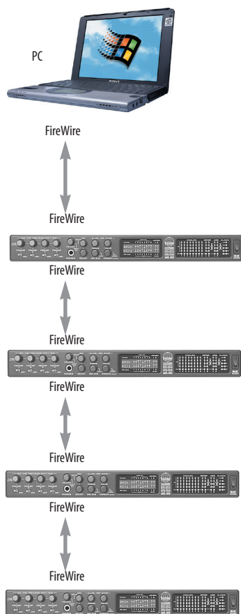
Figure 4-21: Connecting multiple Traveler's (or other MOTU FireWire audio interfaces) to a computer.
