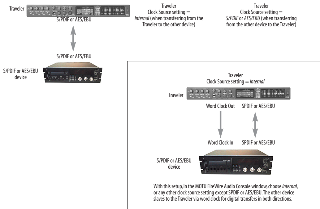
Figure 4-18: Two setups for synchronizing an S/PDIF device with the Traveler. In the top diagram, sync is achieved via the digital I/O connection itself. In this case, you have to choose S/PDIF or AES/EBU as the Traveler's clock source when recording from the other device. If you don't want to have to worry about switching the Clock Source setting depending on the direction of the digital transfer, you can slave the other device to word clock from the Traveler or vice versa (not shown). The Word Clock connection maintains sync, regardless of the direction of the transfer.
