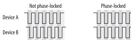
Figure 4-10: When transferring audio, two devices must have phase-locked audio clocks to prevent clicks, pops or other artifacts.
