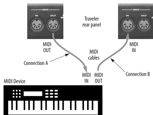
Figure 4-3: Connecting a MIDI device to the Traveler.
