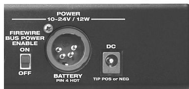
Figure 4-5: The Traveler's battery and power supply options.
