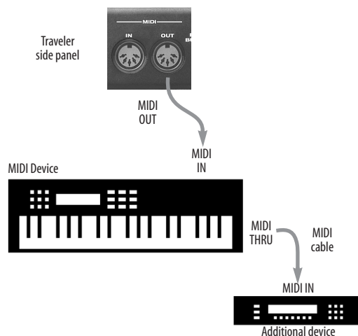
Figure 4-4: Connecting additional devices with MIDI THRU ports.
