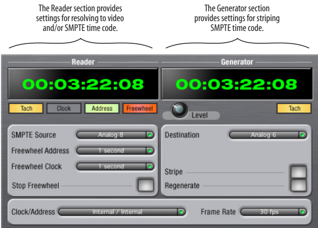
Figure 11-1: SMPTE Console gives you access to your Traveler’s on-board SMPTE time code synchronization features.
