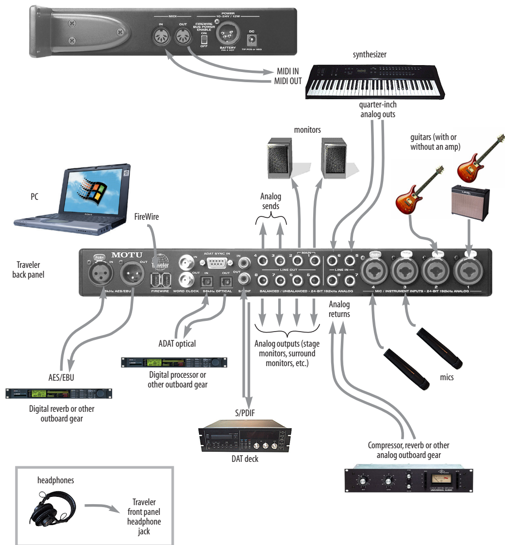
Figure 4-7: A typical Traveler studio setup.
