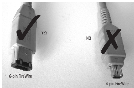
Figure 4-6: 4-pin FireWire connectors cannot be used for bus power.
