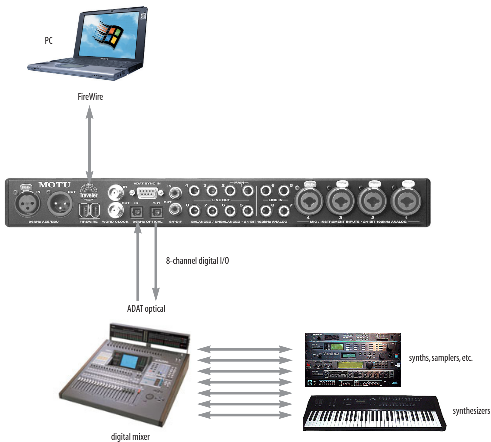
Figure 4-8: Using the Traveler with a digital mixer.
