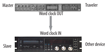
Figure 4-19: Slaving another digital audio device to the Traveler via word clock. For the Traveler clock source, choose any source besides word clock, as it is not advisable to chain word clock.
