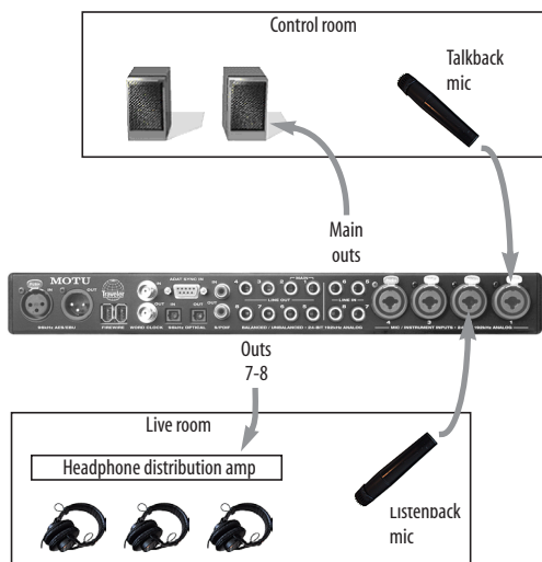
Figure 10-2: Typical hardware setup for Talkback and Listenback.
