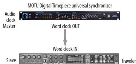
Figure 4-20: Slaving the Traveler to word clock. For the Traveler clock source, choose 'Word Clock In'.
