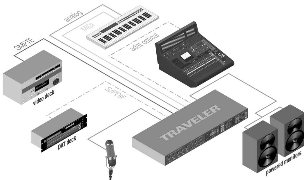
Figure 10-7: An example setup of a system that takes full advantage of CueMix DSP.
