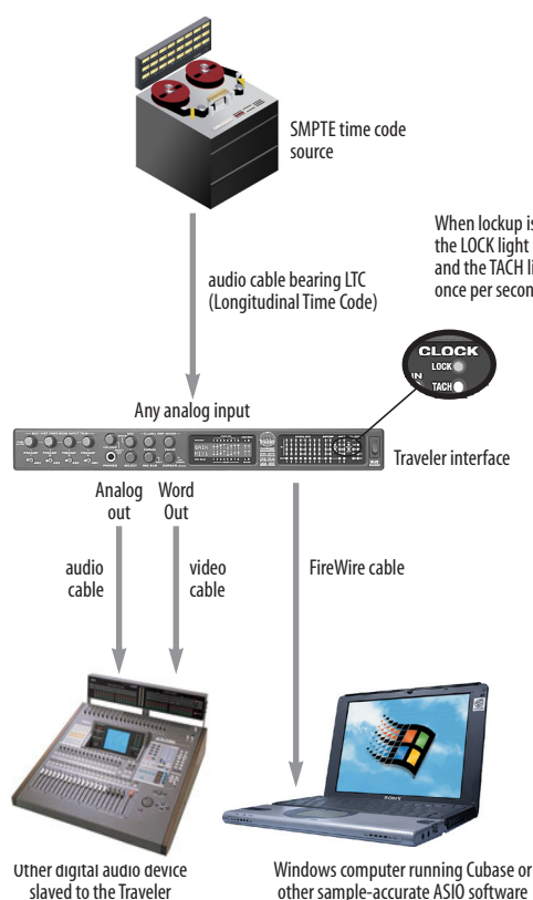
Figure 4-15: Connections for synchronizing the Traveler directly to SMPTE time code.
