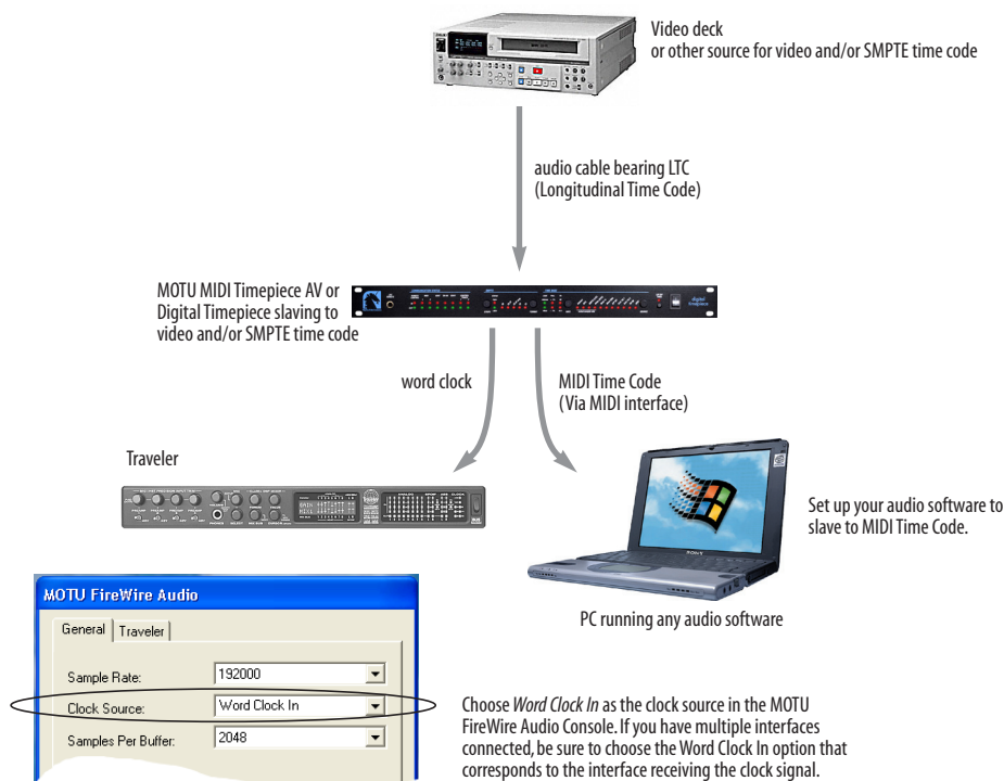
Figure 4-16: If your host audio software does not support sample-accurate sync and the Traveler's built-in SMPTE sync features, use a universal synchronizer such as the MOTU MIDI Timepiece AV or Digital Timepiece.
