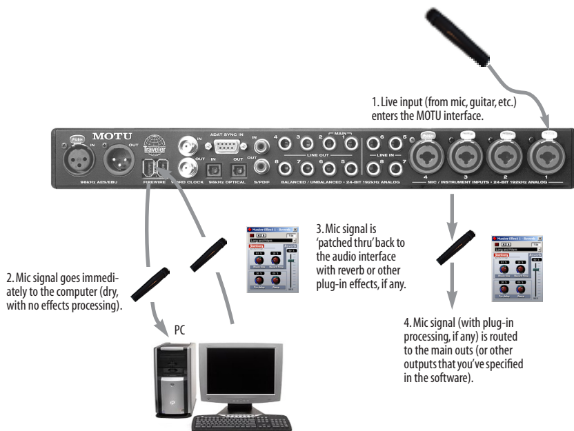
Figure 9-1: There are two ways to monitor live audio inputs with a Traveler: 1) through the computer or 2) via CueMix™ DSP hardware monitoring. This diagram shows method 1 (through the computer). When using this method, use your host software's buffer setting to reduce the slight delay you hear when monitoring the live input, but don't lower it too much, or your computer might get sluggish.
