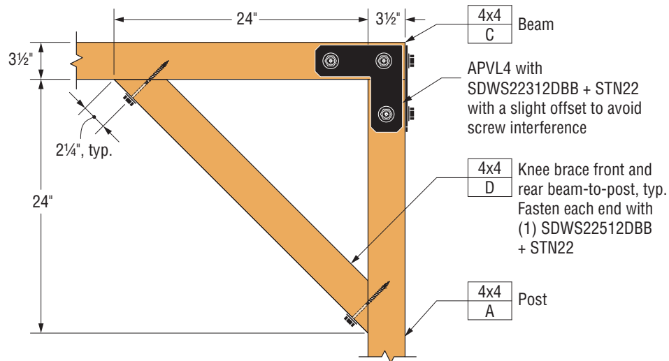
Post-to-Beam Connection
