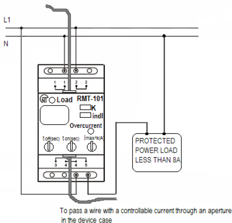
Figure 2 - Wiring diagram
