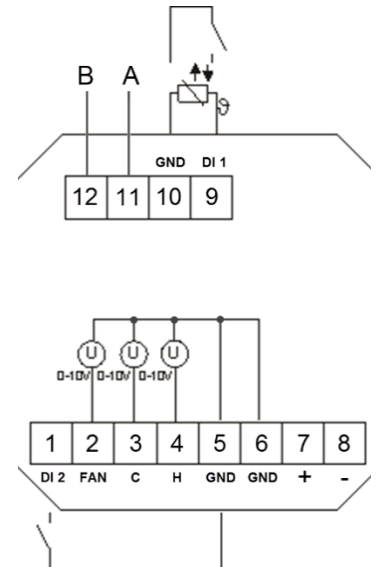
JOY Fancoil EC 3AO (24 V ~/=)
