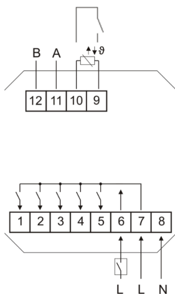
JOY Fancoil 5DO (85..260 V ~)
