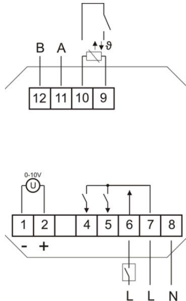
JOY Fancoil EC AO2DO (85..260 V ~)
