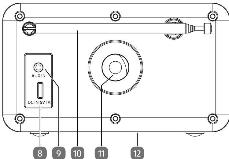
Fig. 2 – BACK VIEW
