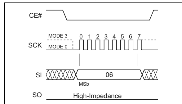
FIGURE 4-15: WRITE ENABLE ( \overline{\text{WREN}} ) SEQUENCE
