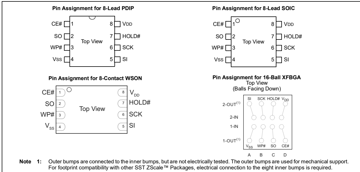
FIGURE 2-1: PIN ASSIGNMENTS
