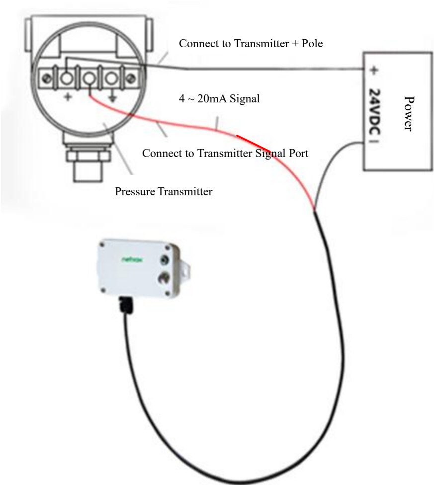
Figure1 2-wire System Example Diagram (for wiring reference)
