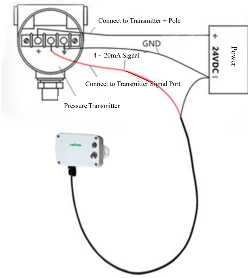
Figure2 3-wire System Example Diagram (for wiring reference)
