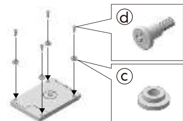
2.5" SSD Installation
