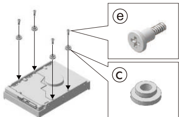
3.5" HDD Installation
