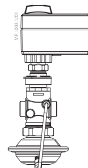
AME 10, AME 11 + AVQM (see data sheet)
