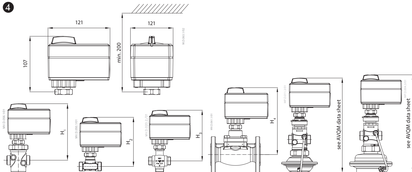
AME 10, AME 11 + VM 2 (DN 15-32)
