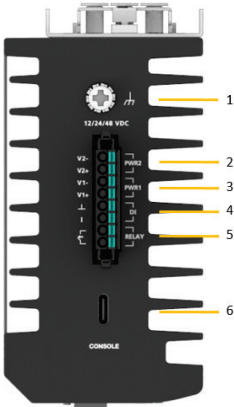
Top Panel
