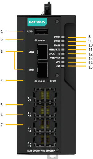
Front Panel
