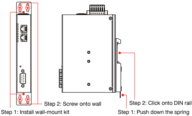
Wall-Mount Installation
