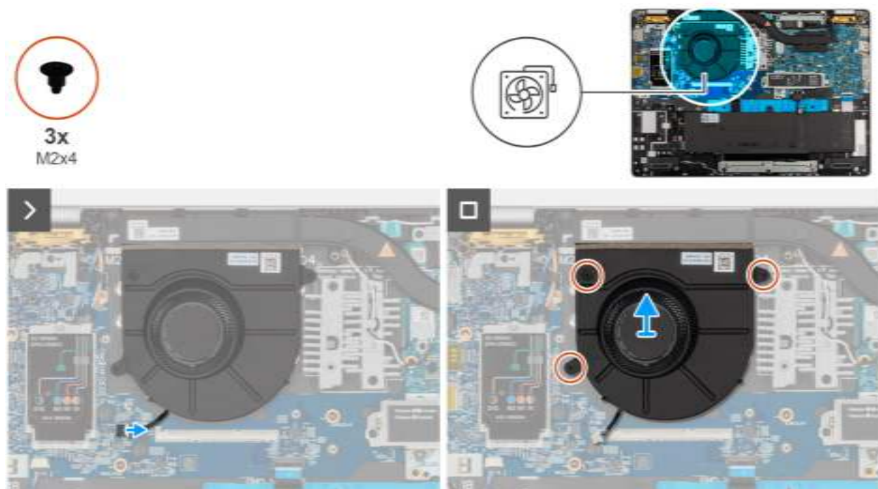
Figure 19. Removing the fan
