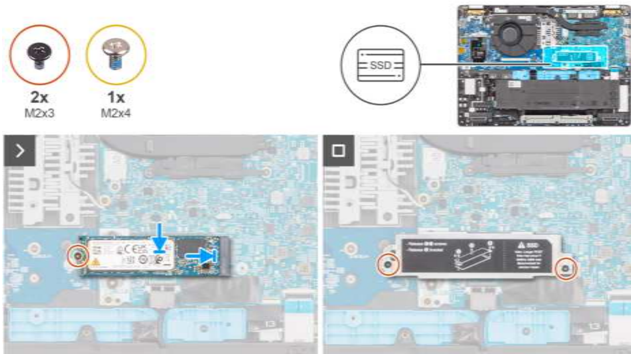
Figure 15. Installing the M.2 2280 SSD
