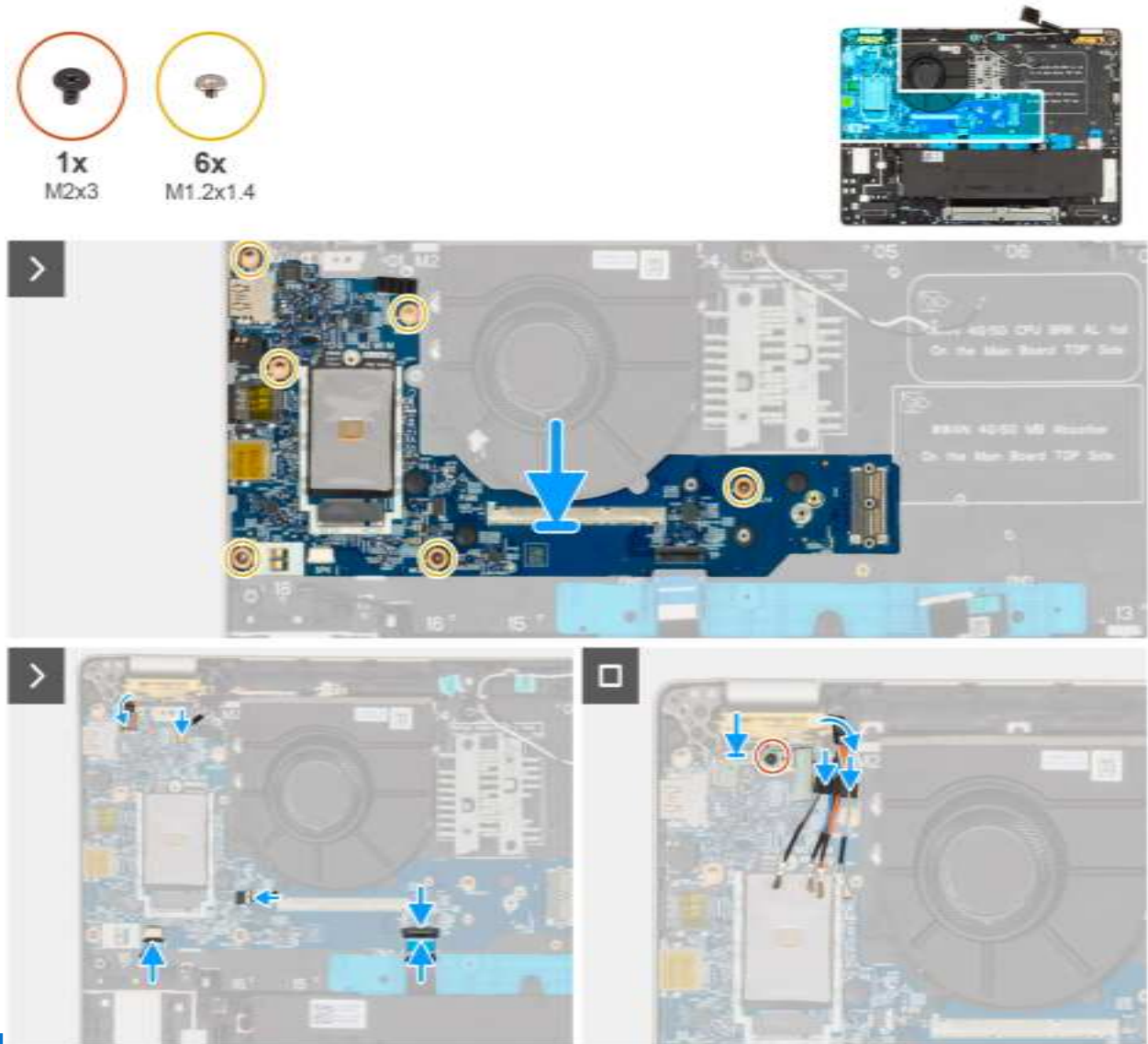
Figure 57. Installing the I/O daughter
