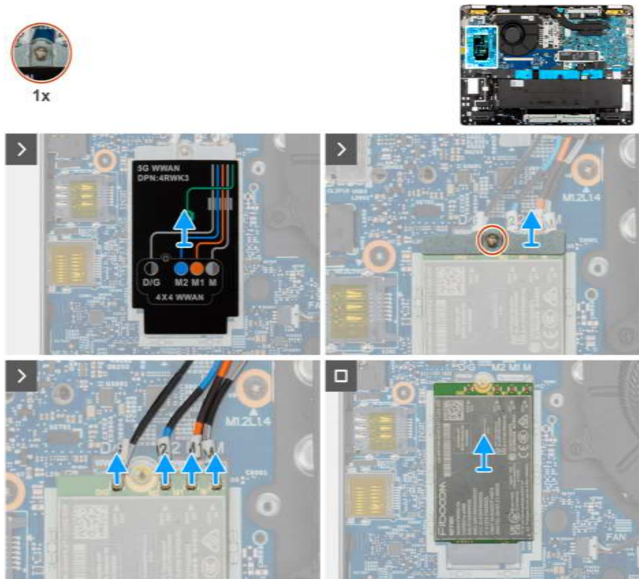
Figure 10. Removing the 5G WWAN card
