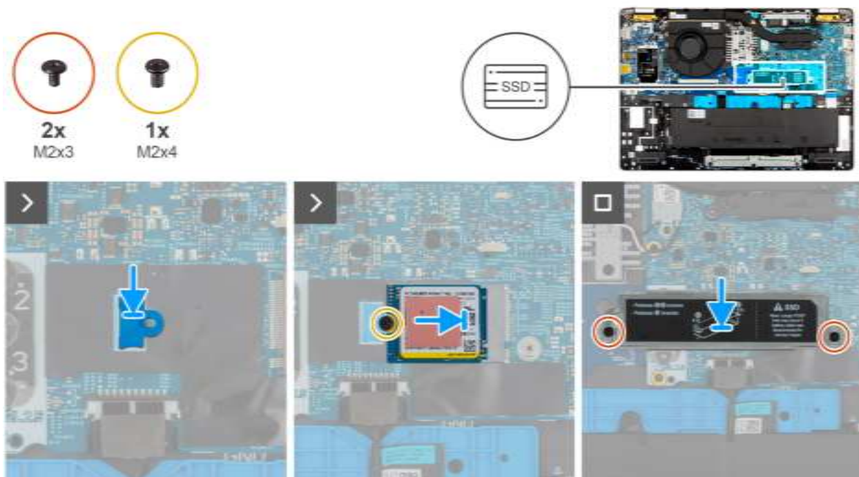
Figure 13. Installing the M.2 2230 SSD
