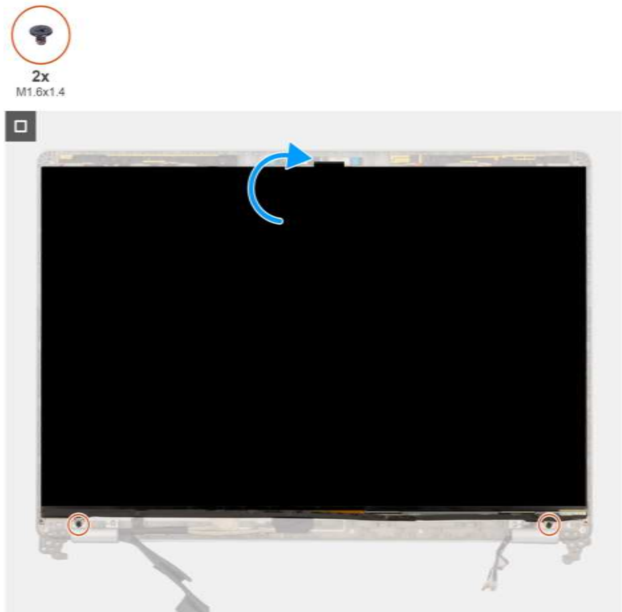
Figure 33. Installing the display panel
