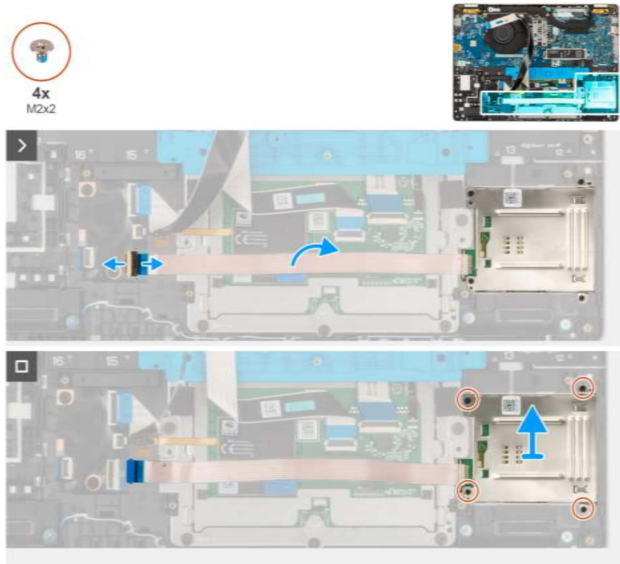
Figure 42. Removing the smart-card reader
