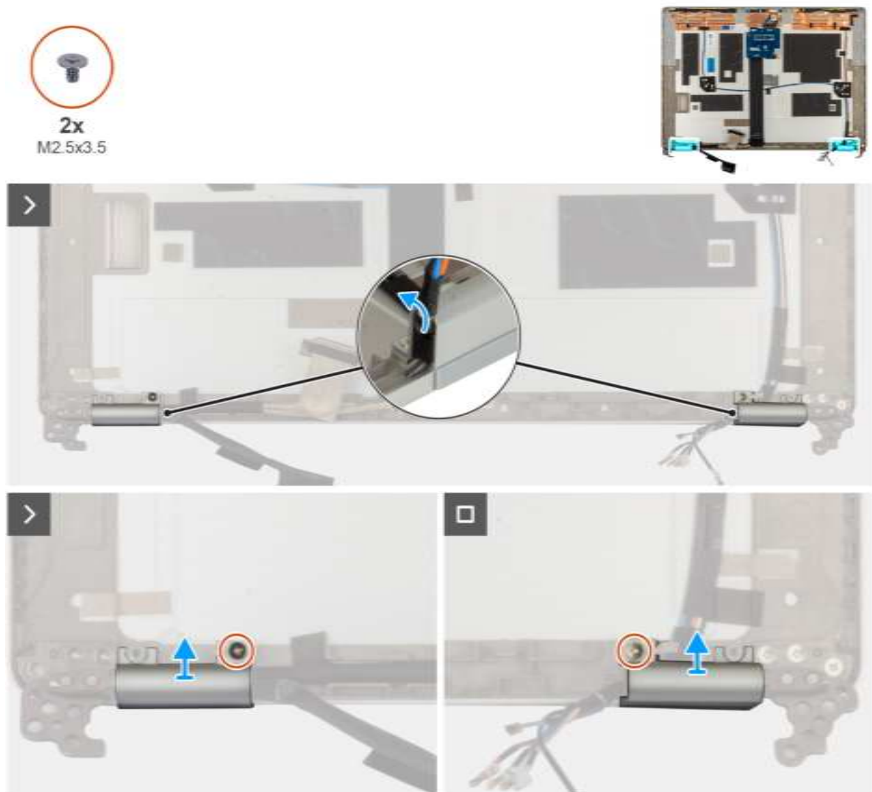
Figure 34. Removing the display hinges
