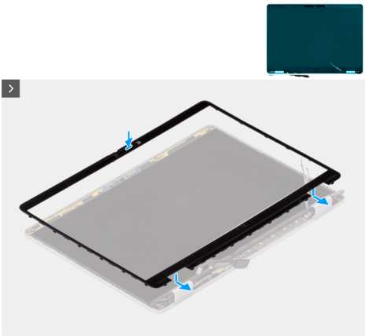
Figure 29. Installing the display bezel
