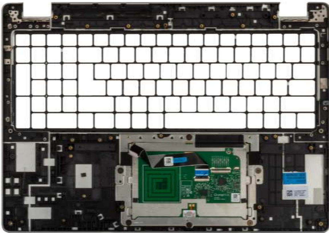
Figure 62. Installing the palm-rest assembly
