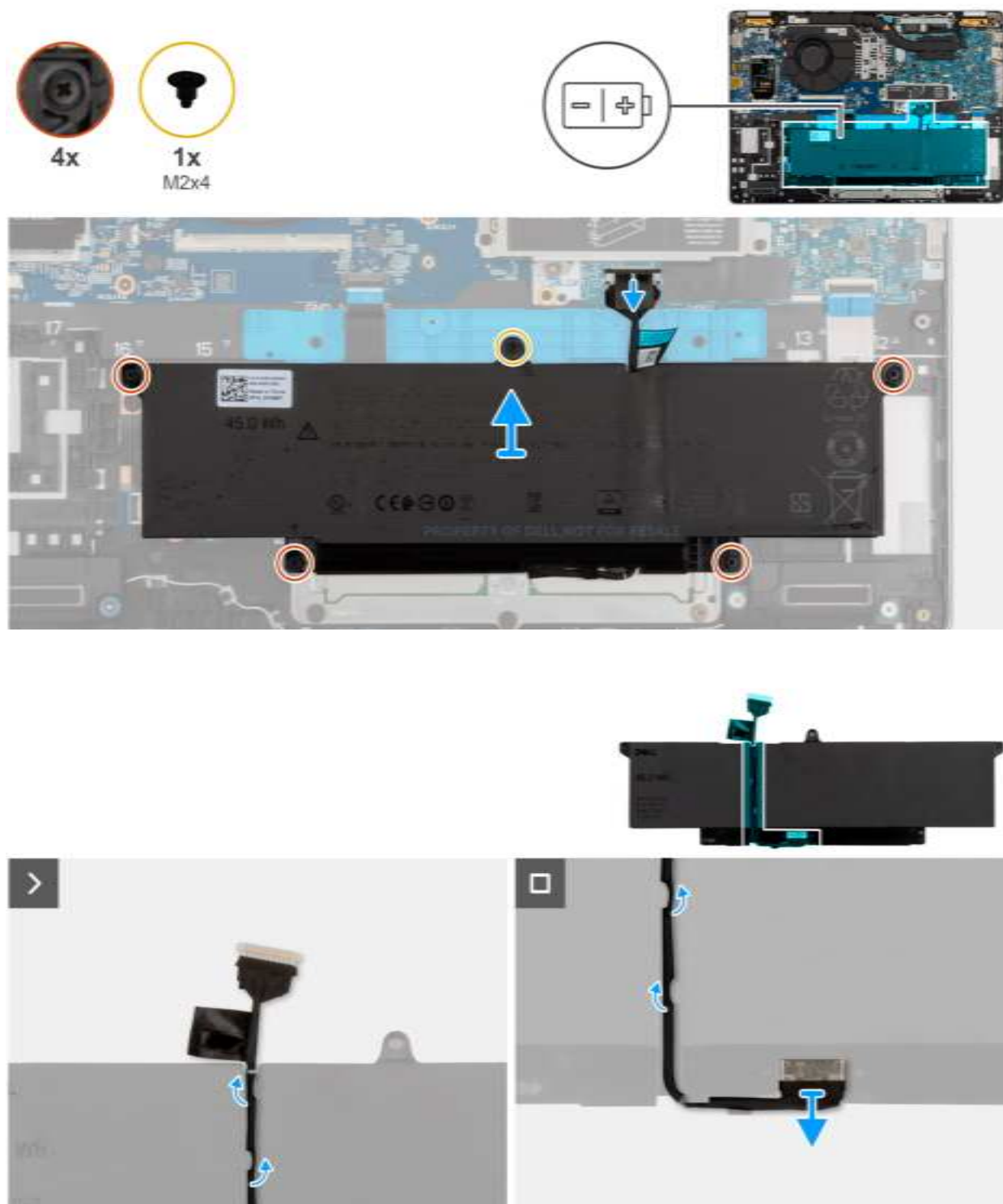
Figure 8. Removing the battery
