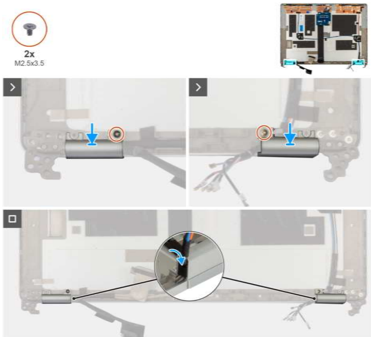
Figure 35. Installing the display hinge cap
