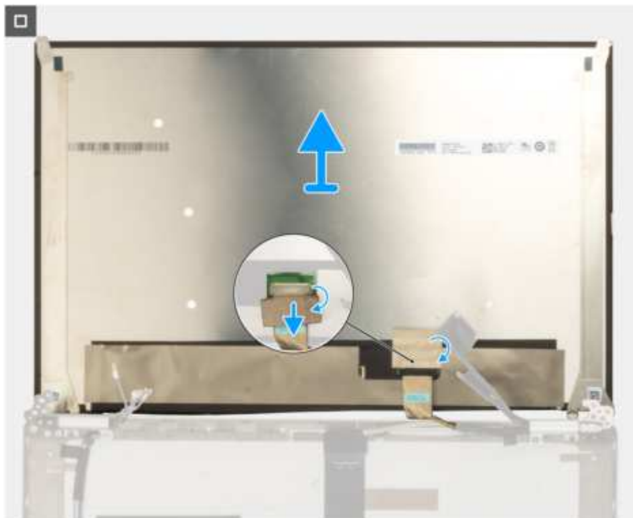
Figure 31. Removing the display panel
