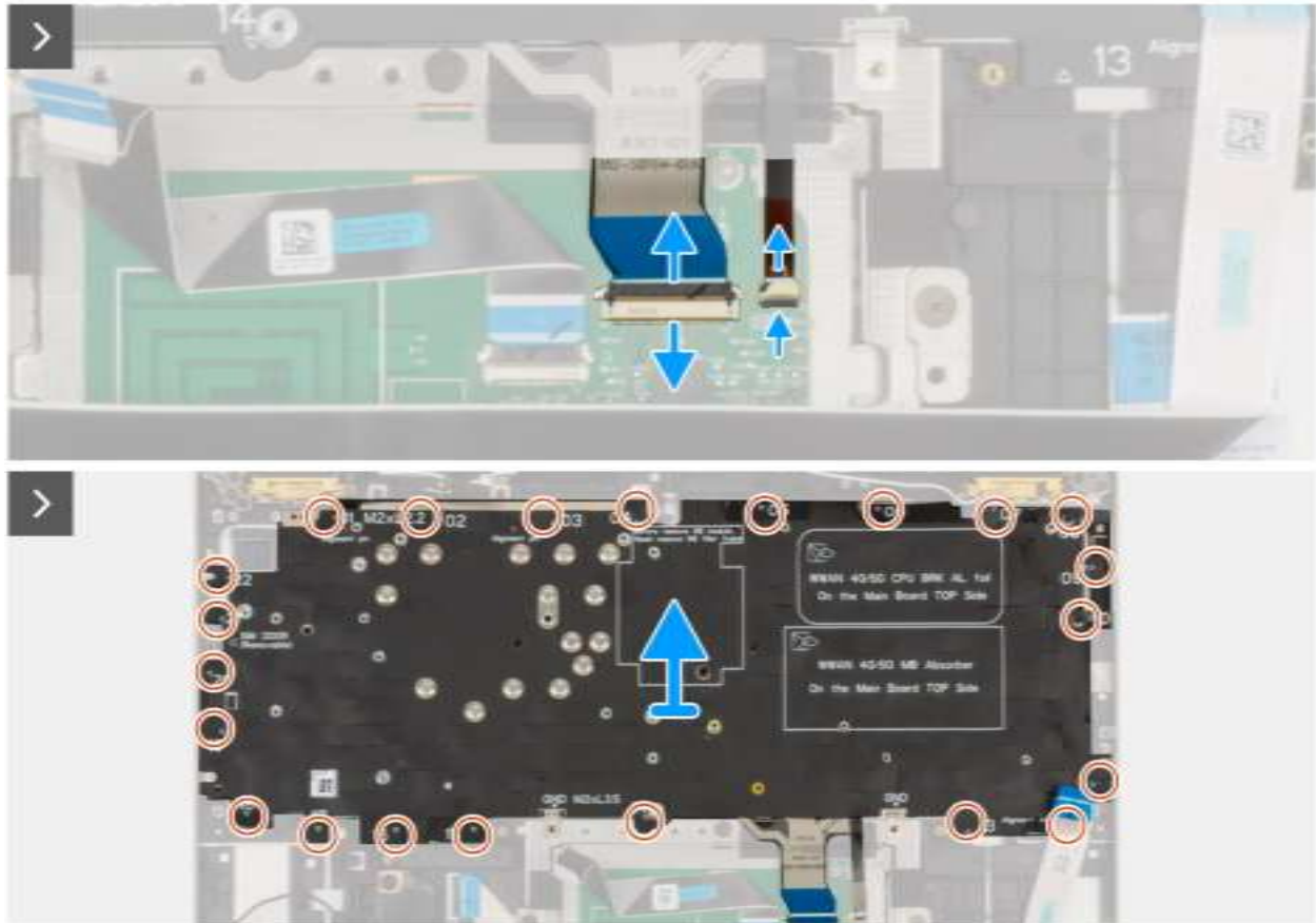
Figure 58. Removing the keyboard
