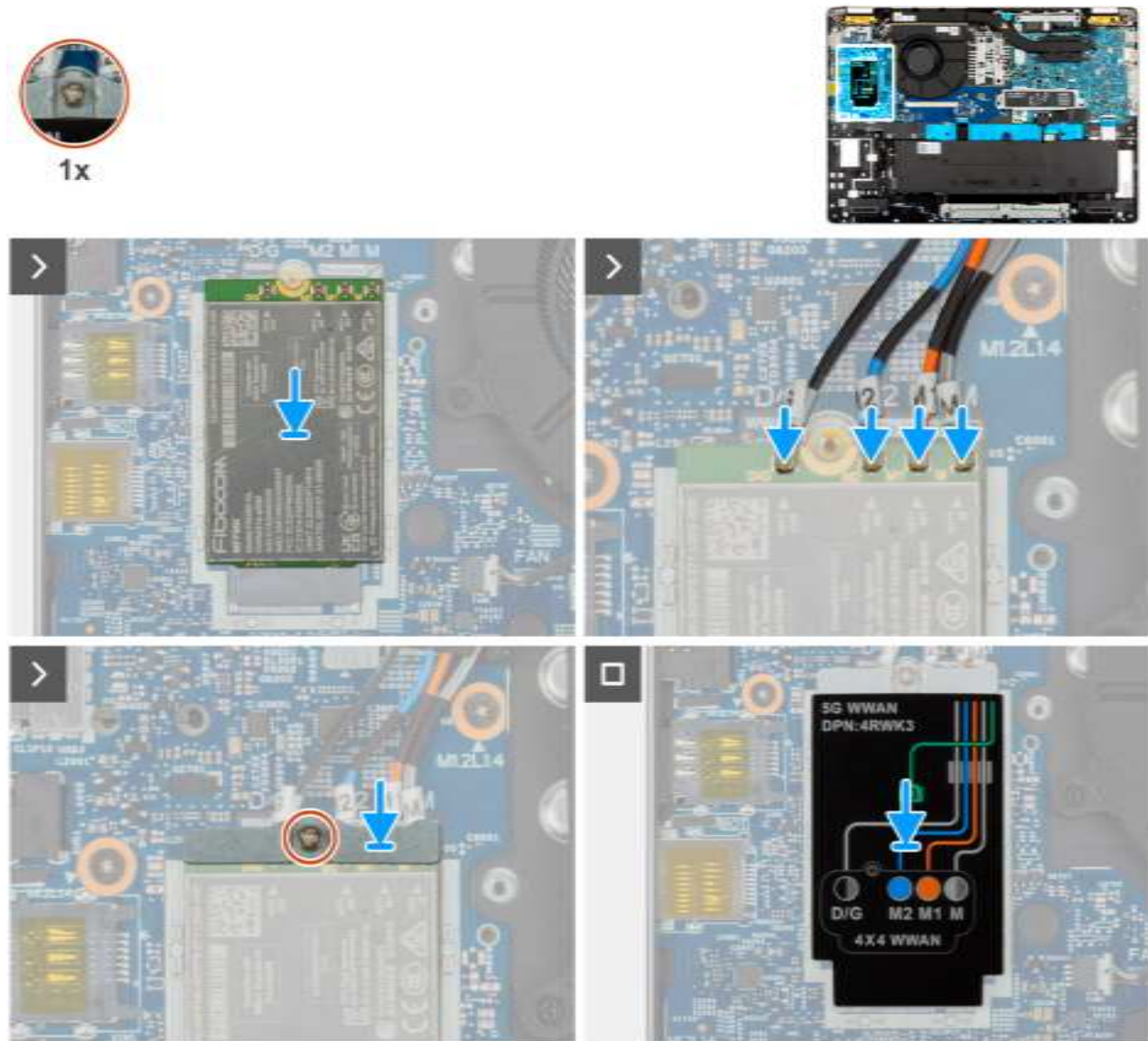
Figure 11. Installing the 5G WWAN card
