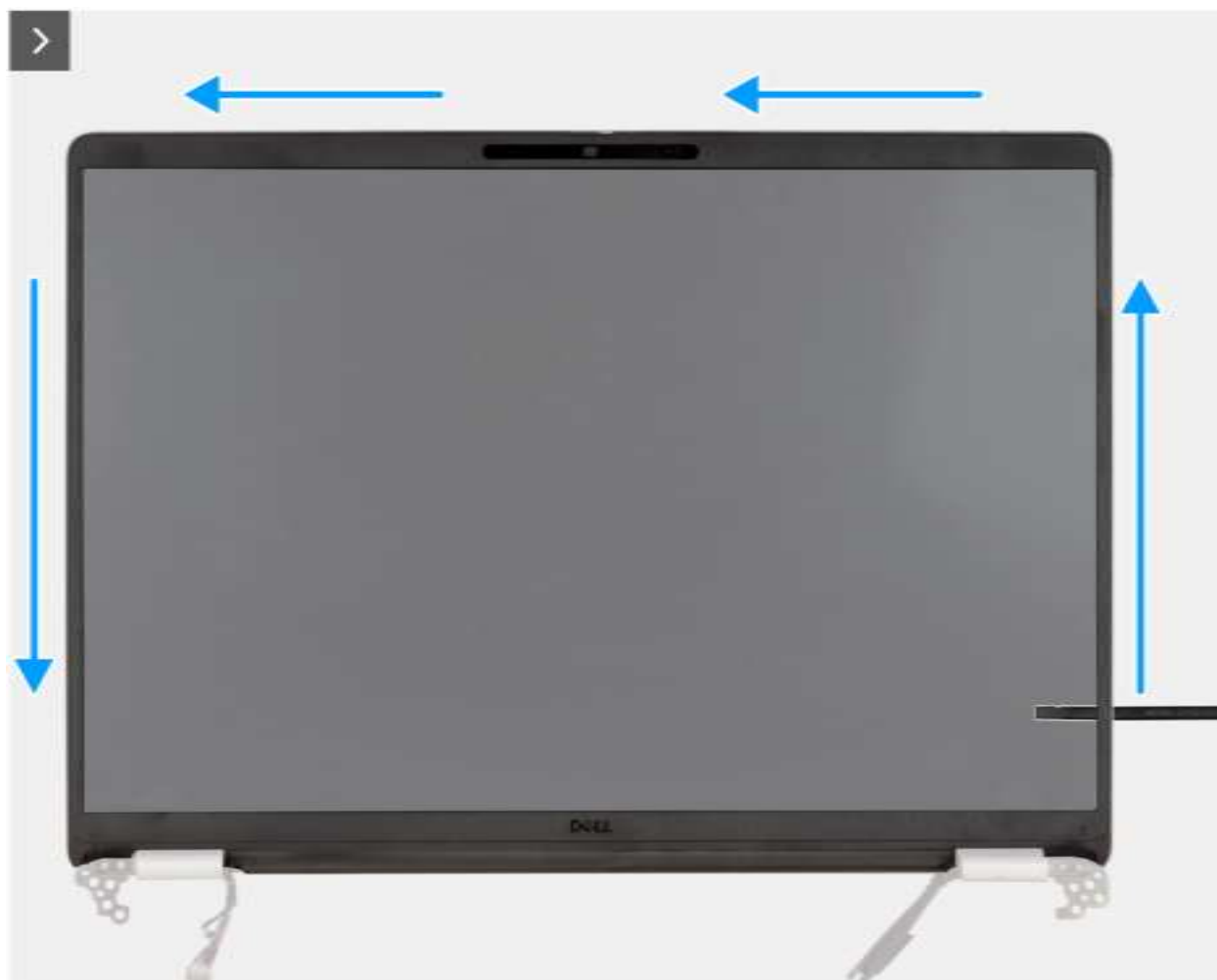
Figure 27. Removing the display bezel
