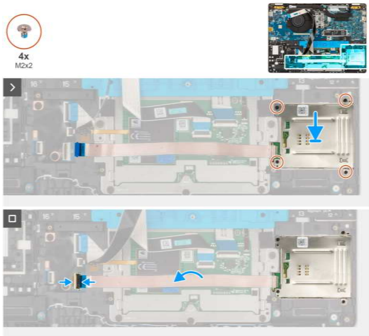
Figure 43. Installing the smart-card reader
