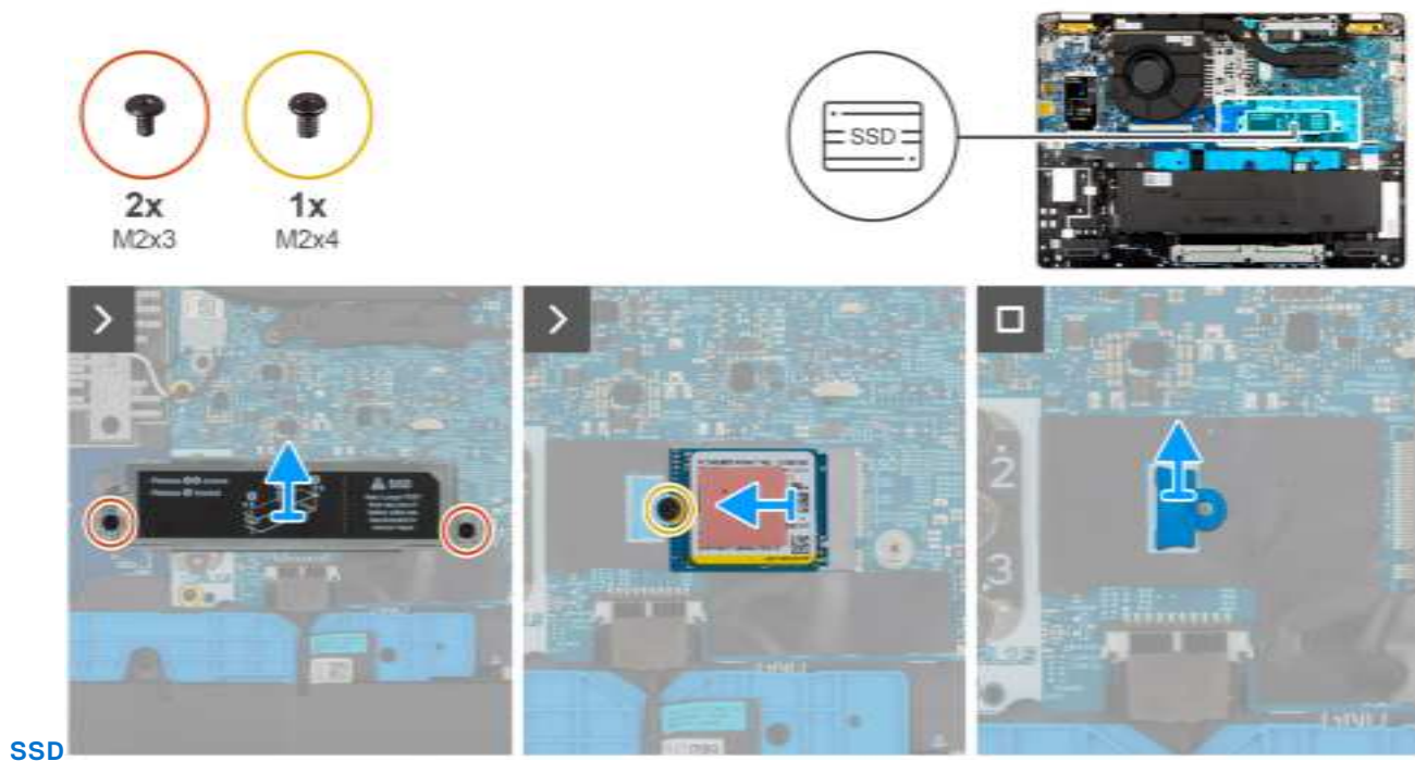
Figure 12. Removing the M.2 2230
