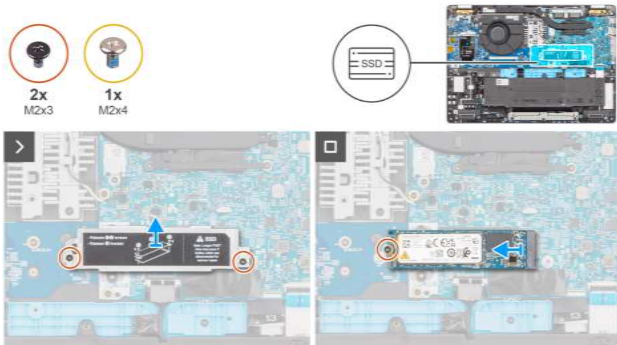
Figure 14. Removing the M.2 2280 SSD
