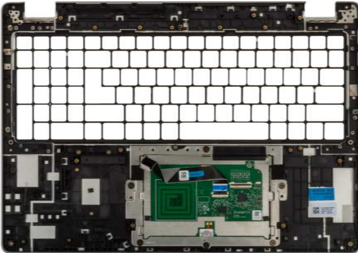
Figure 61. Removing the palm-rest assembly
