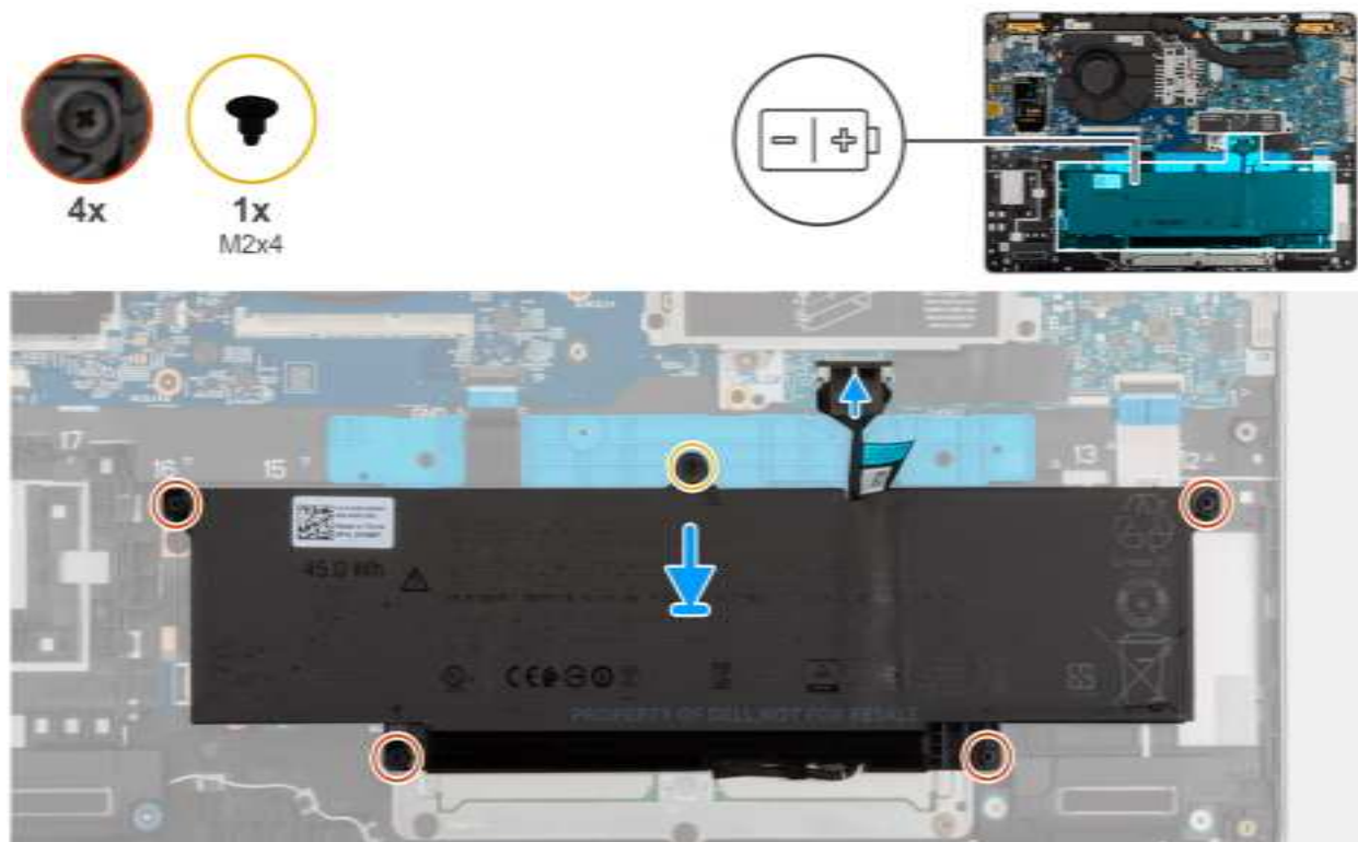
Figure 9. Installing the battery
