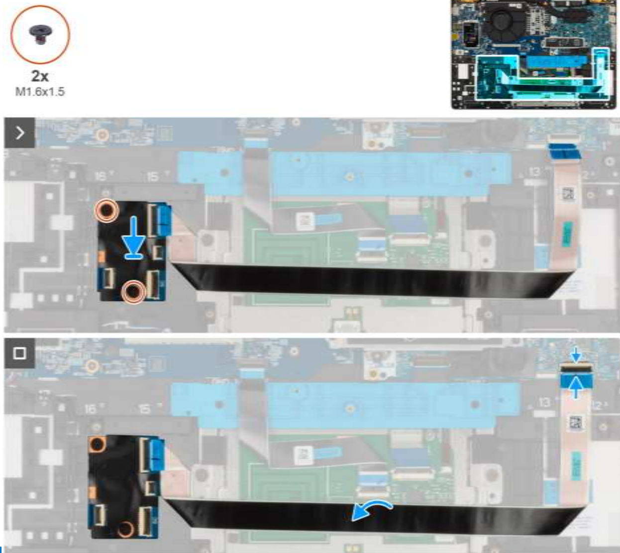
Figure 45. Installing the USH daughter
