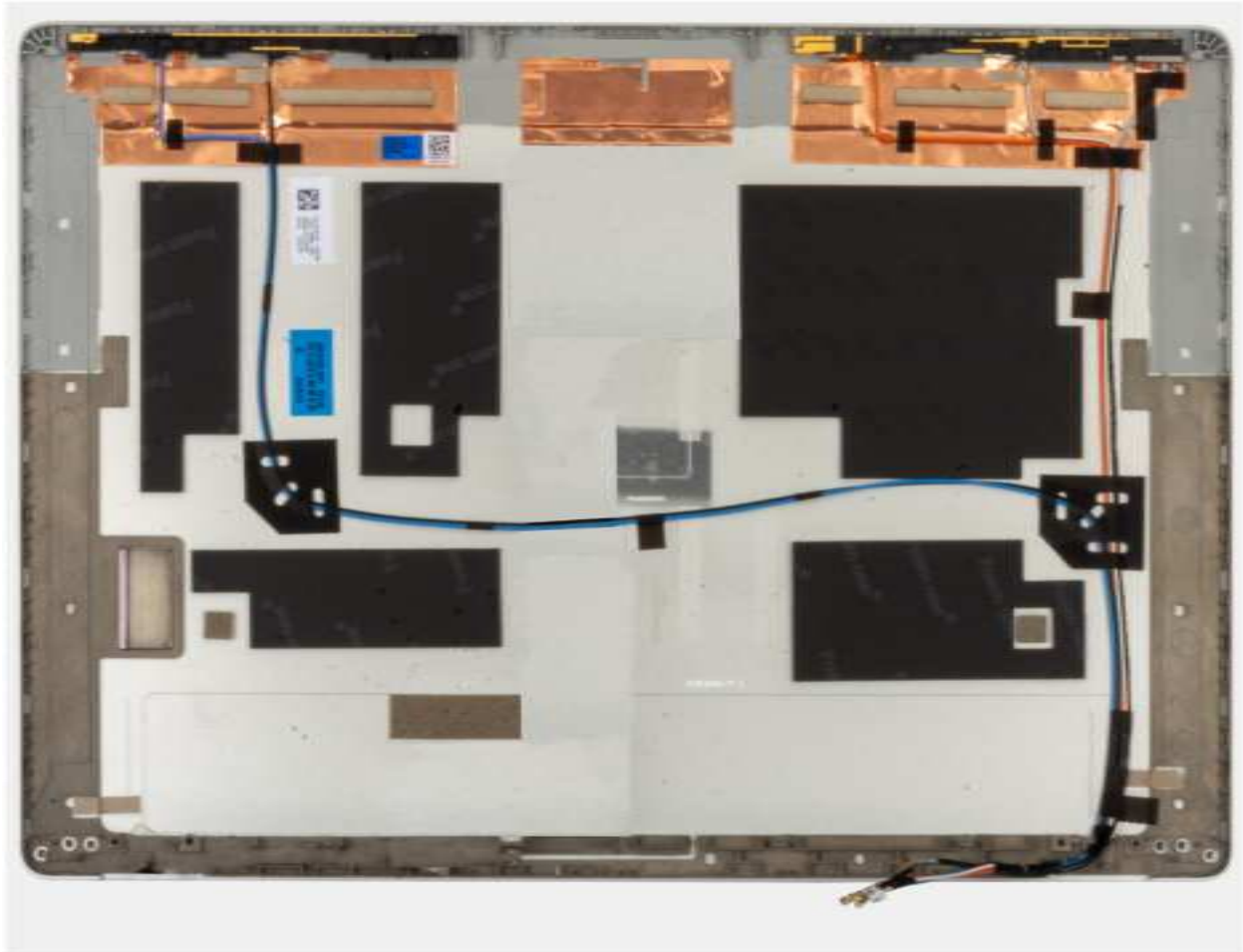
Figure 40. Removing the display back cover
