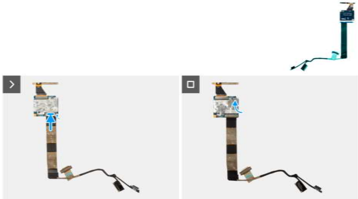
Figure 37. Installing the display cable
