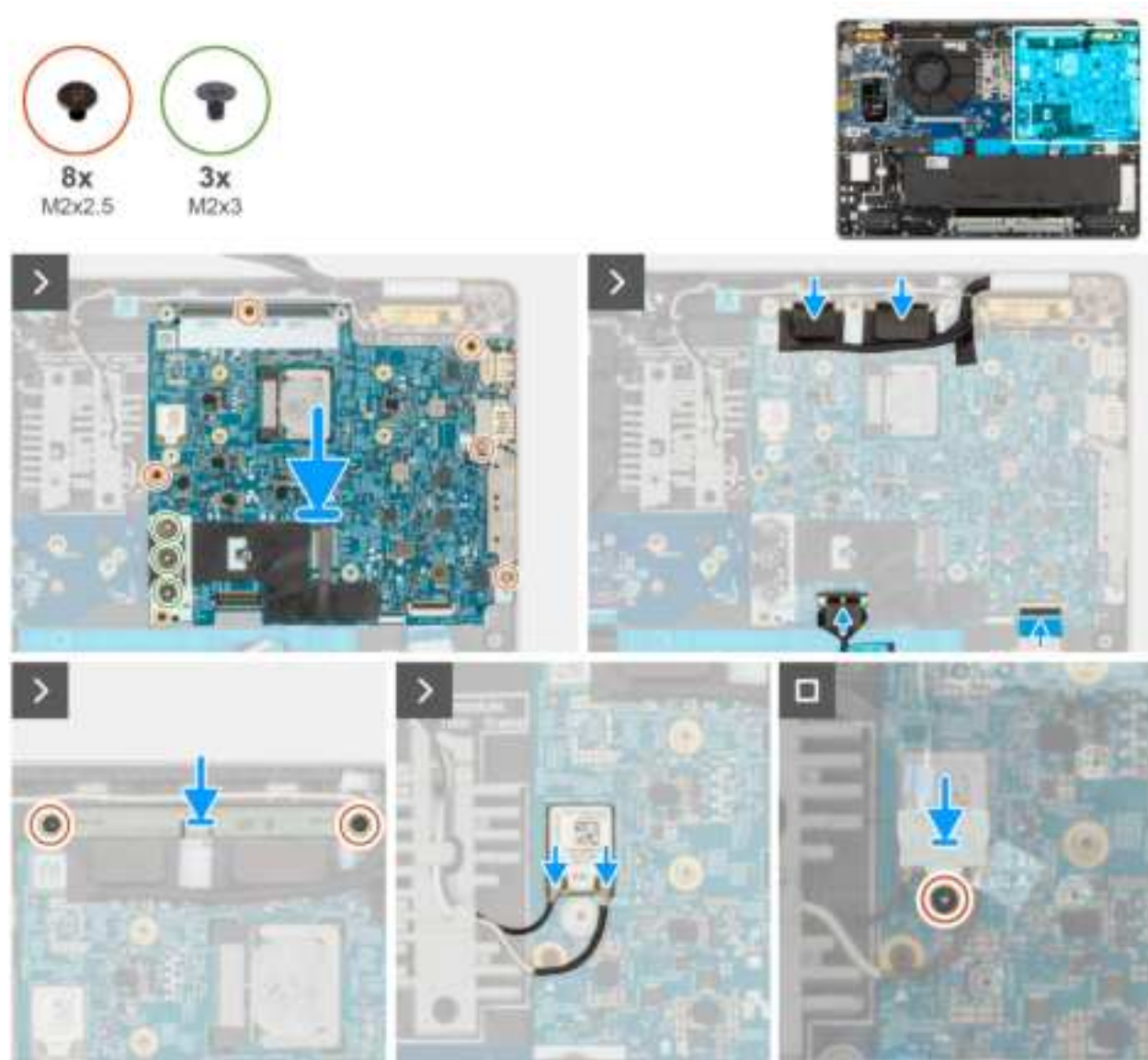
Figure 51. Installing the system board
