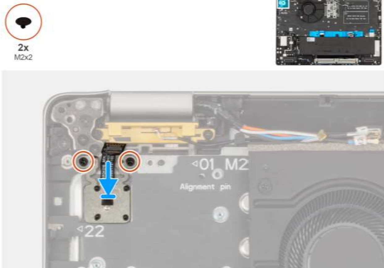
Figure 55. Installing the power button with an optional fingerprint reader
