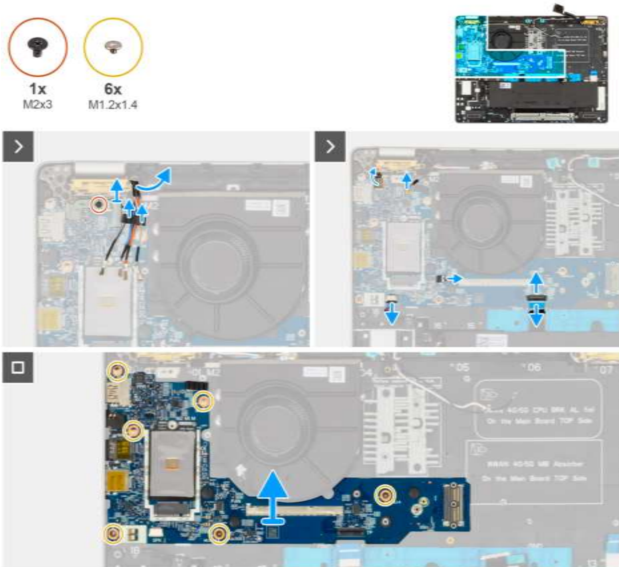
Figure 56. Removing the I/O board
