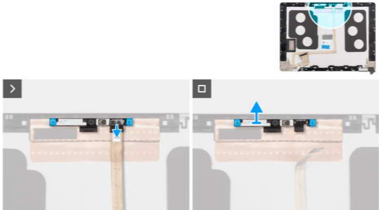
Figure 38. Removing the camera module
