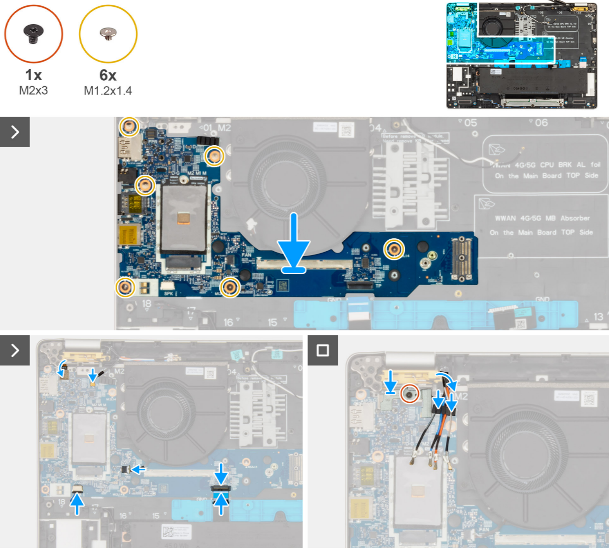
Figure 57. Installing the I/O daughter
