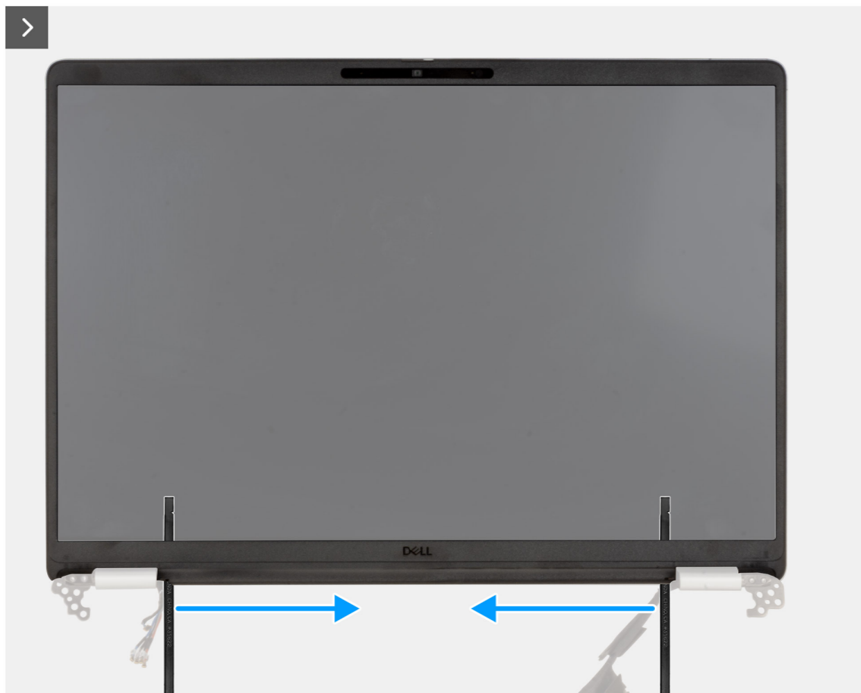
Figure 25. Prying the bezel along the sides
