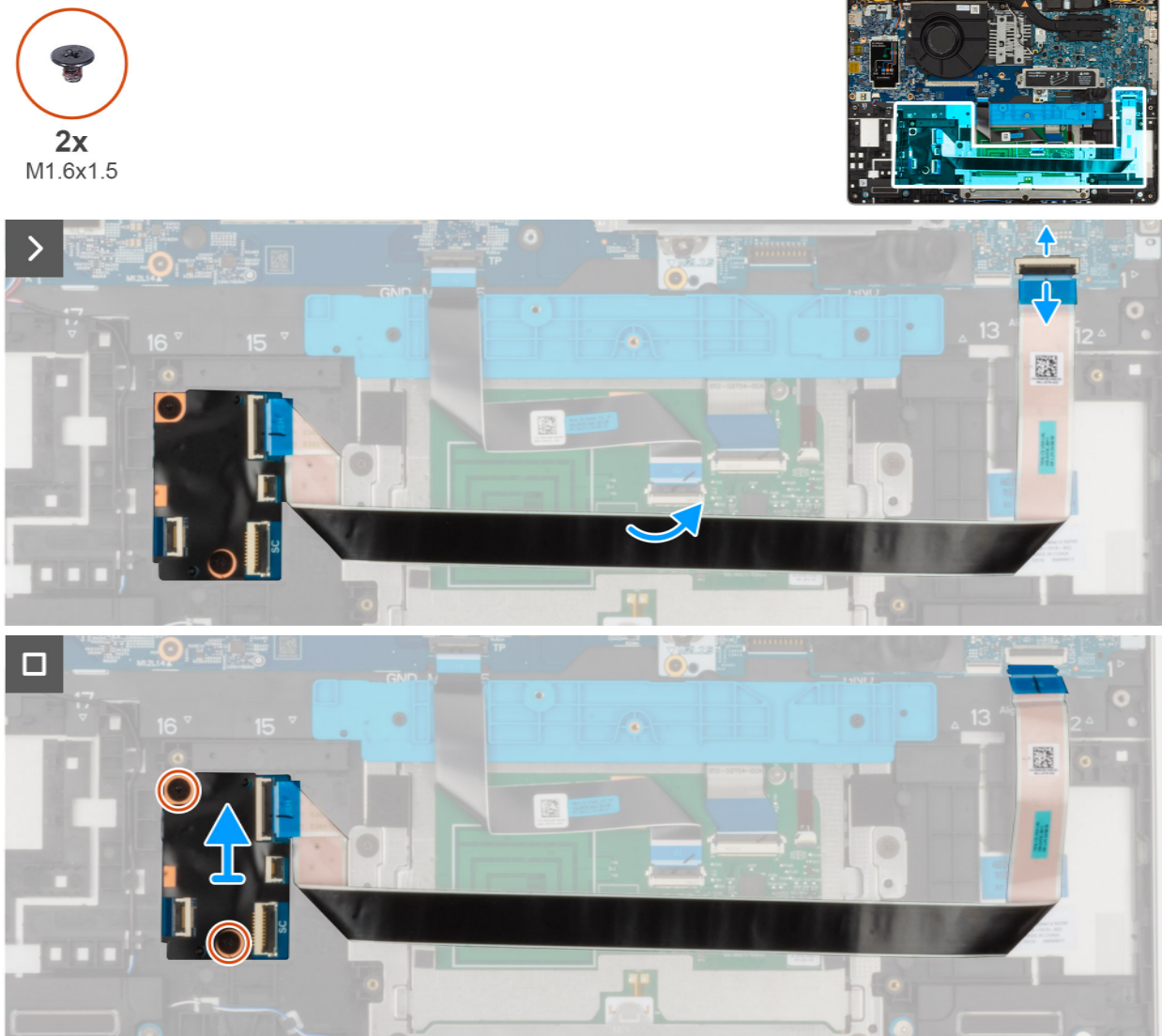
Figure 44. Removing the USH daughter board
