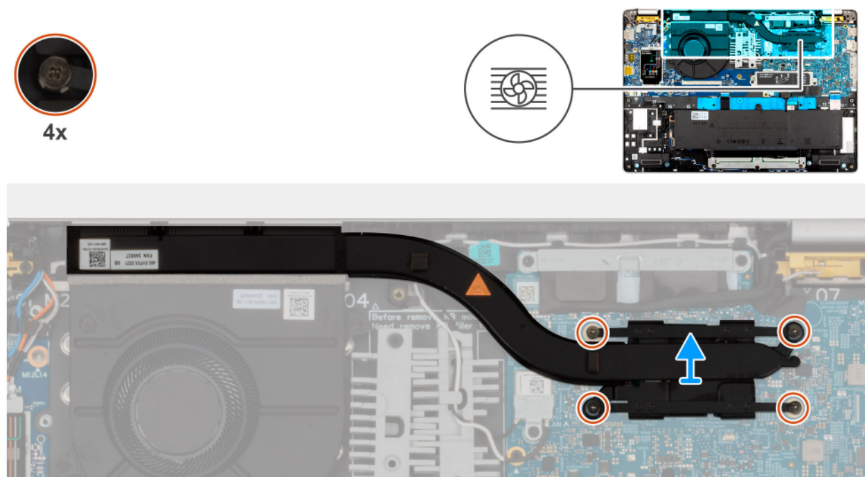
Figure 46. Removing the heat sink
