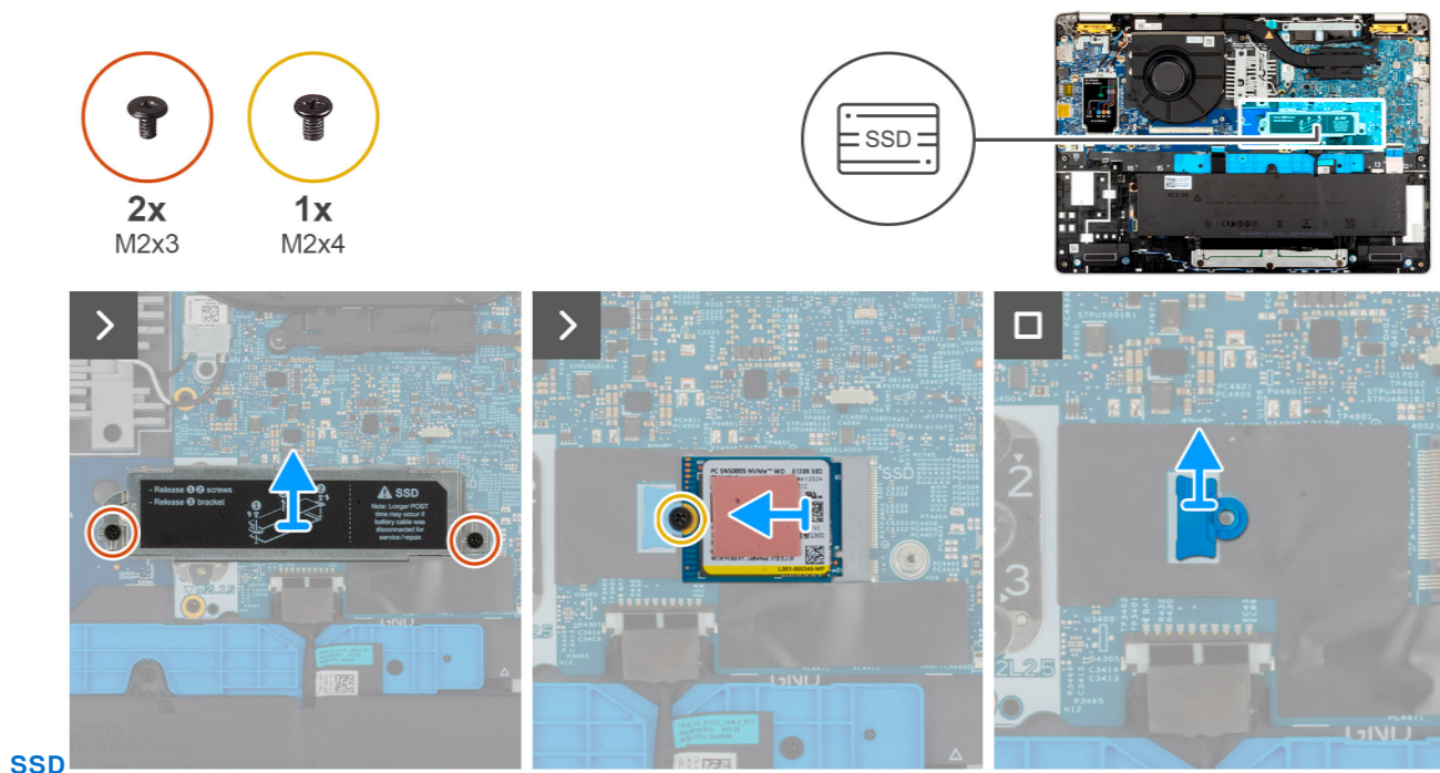
Figure 12. Removing the M.2 2230
