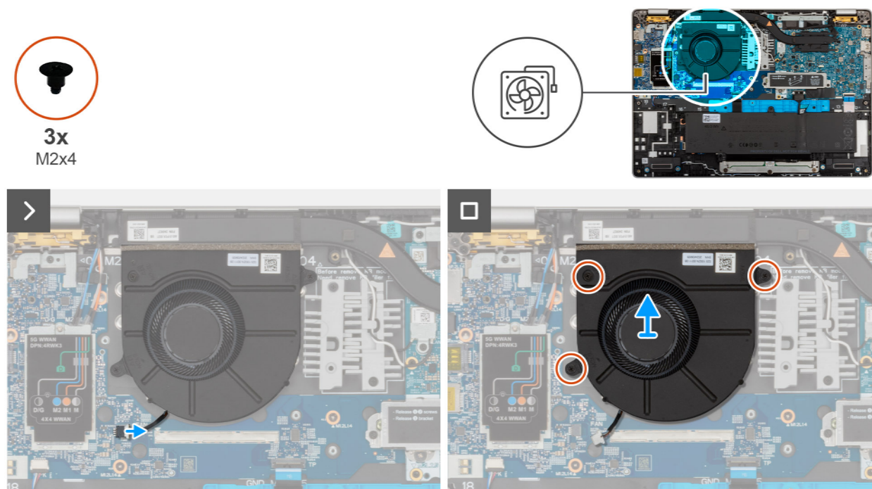
Figure 19. Removing the fan
