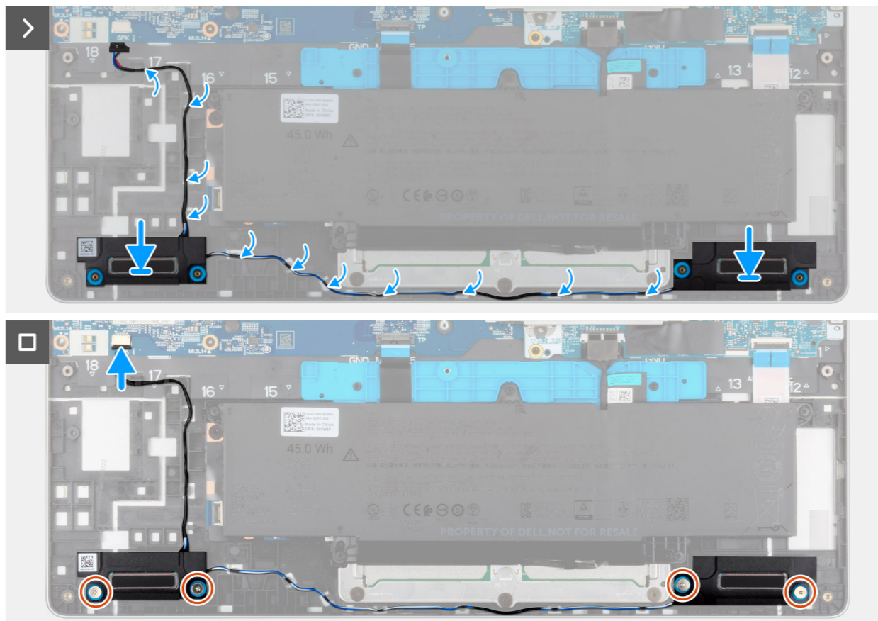
Figure 17. Installing the speakers
