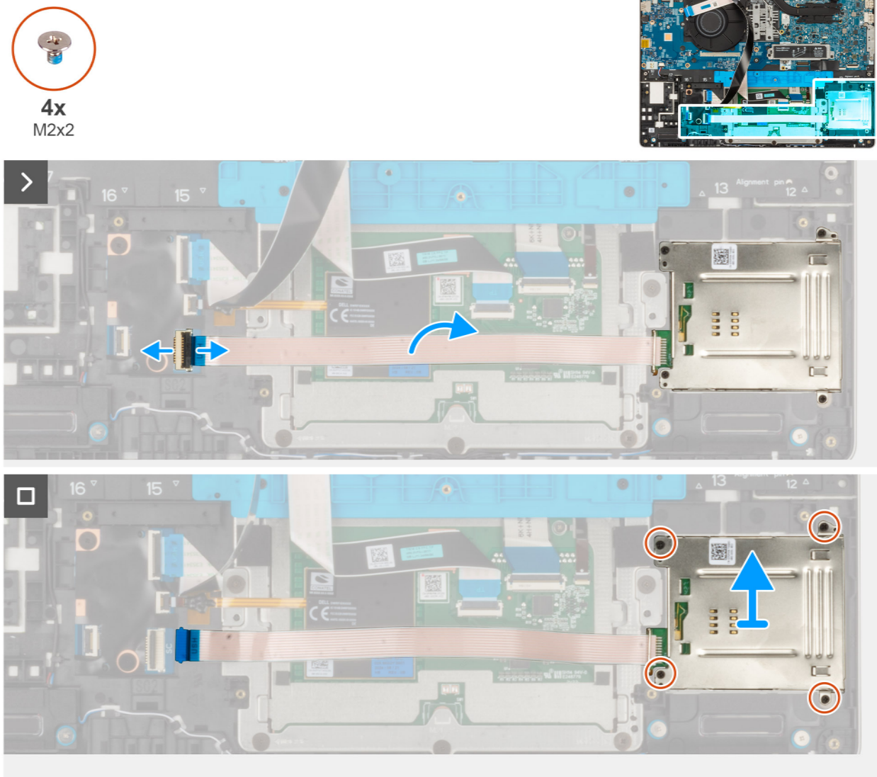
Figure 42. Removing the smart-card reader
