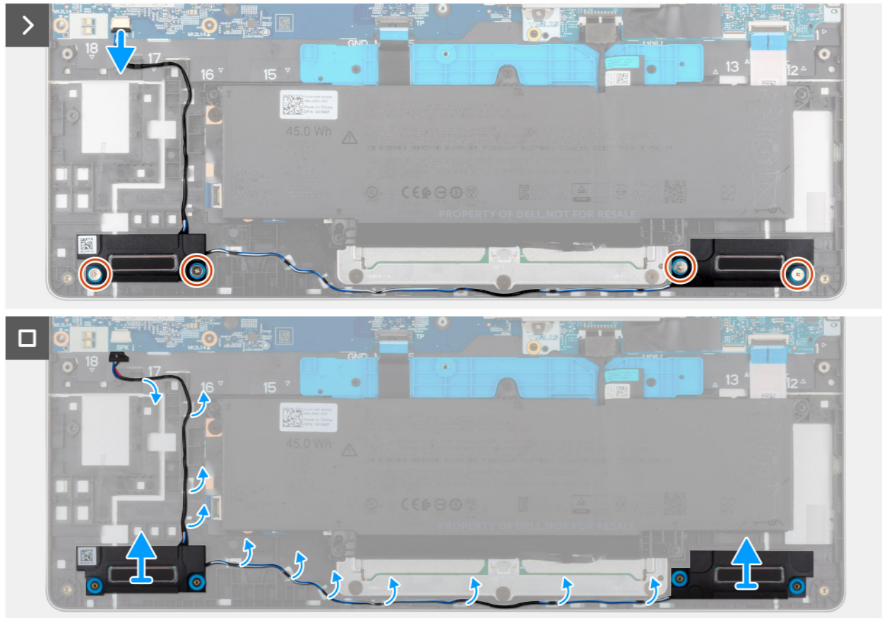
Figure 16. Removing the speakers
