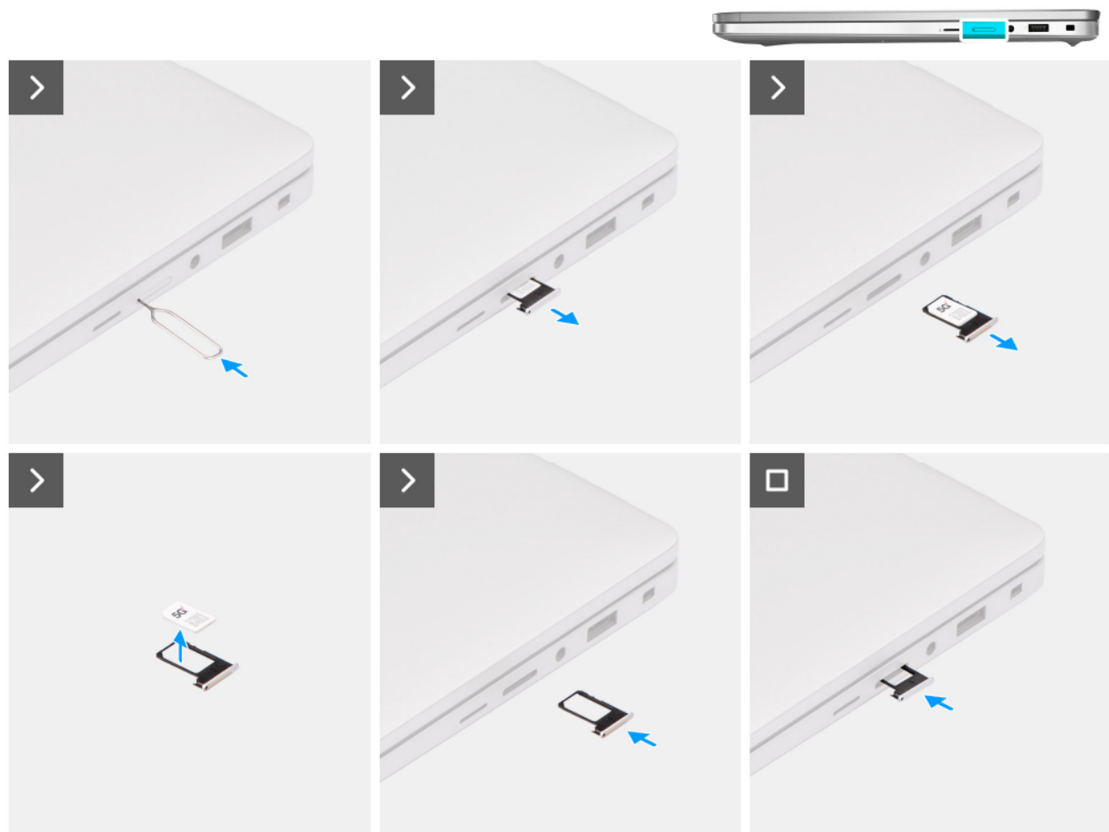
Figure 4. Removing the SIM card tray
