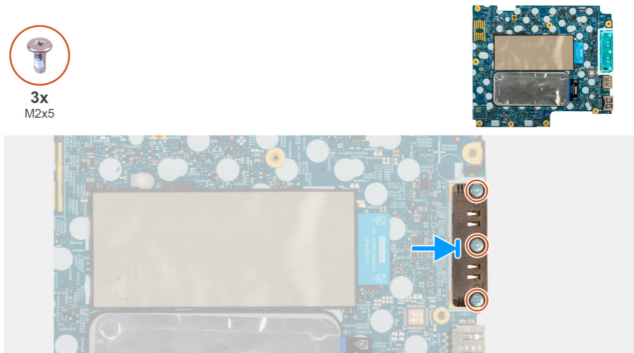
Figure 53. Installing the USB-C Connector Module
