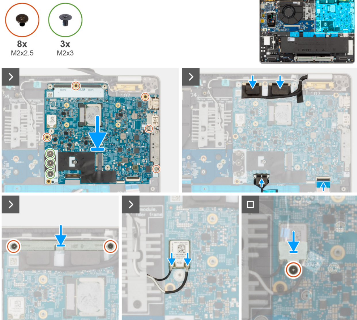
Figure 51. Installing the system board
