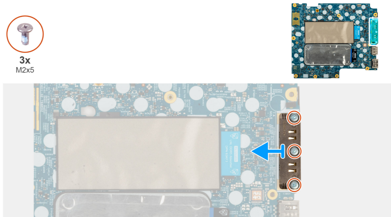
Figure 52. Removing the USB-C Connector Module
