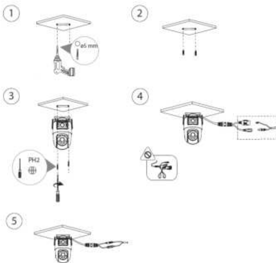
Figure 4-4 Ceiling mount
