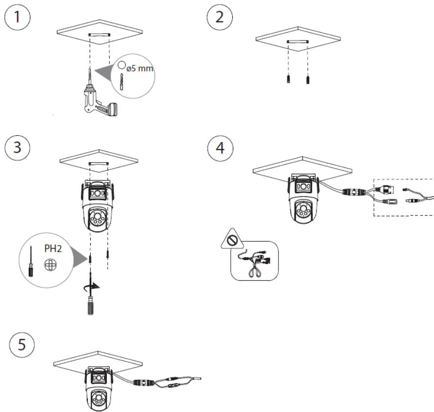
Figure 4-4 Ceiling mount
