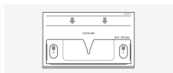
Wall-mounting Guide (AH85-01091A)
