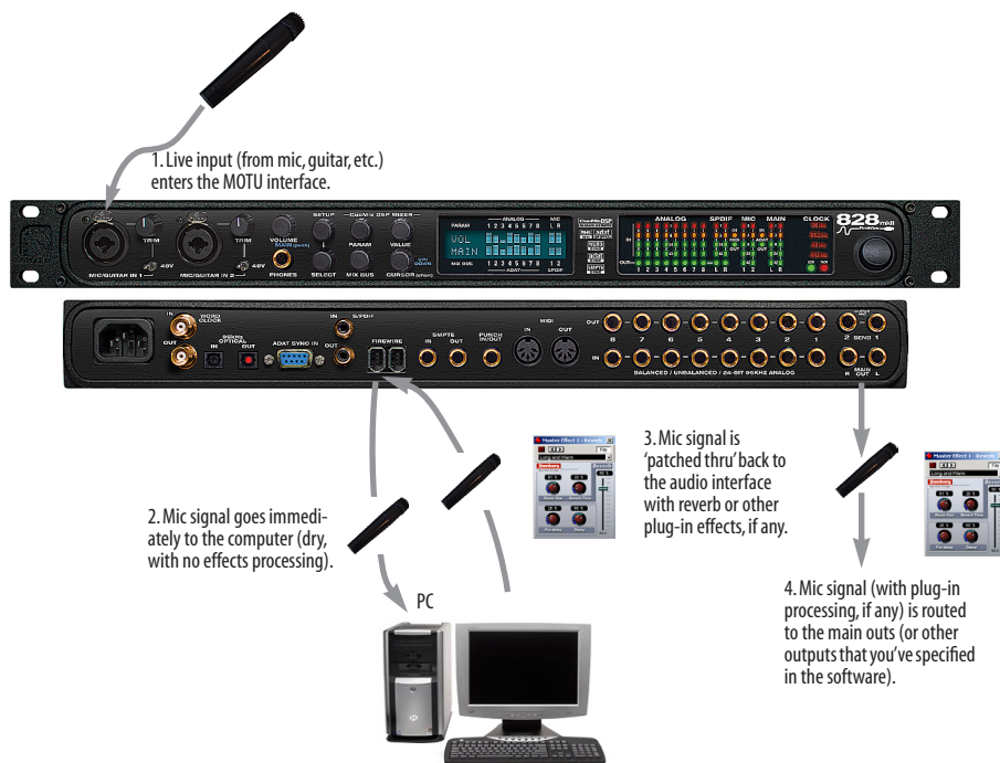
Figure 9-1: There are two ways to monitor live audio inputs with an 828mkII: 1) through the computer or 2) via CueMix™ DSP hardware monitoring. This diagram shows method 1 (through the computer). When using this method, use your host software's buffer setting to reduce the slight delay you hear when monitoring the live input, but don't lower it too much, or your computer might get sluggish.
