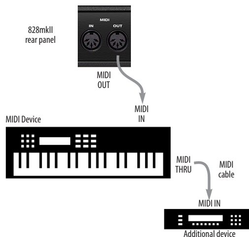
Figure 4-4: Connecting additional devices with MIDI THRU ports.
