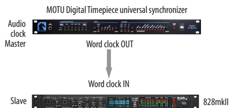
Figure 4-18: Slaving the 828mkII to word clock. For the 828mkII clock source, choose 'Word Clock In'.
