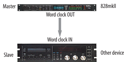
Figure 4-17: Slaving another digital audio device to the 828mkII via word clock. For the 828mkII clock source, choose any source besides word clock, as it is not advisable to chain word clock.
