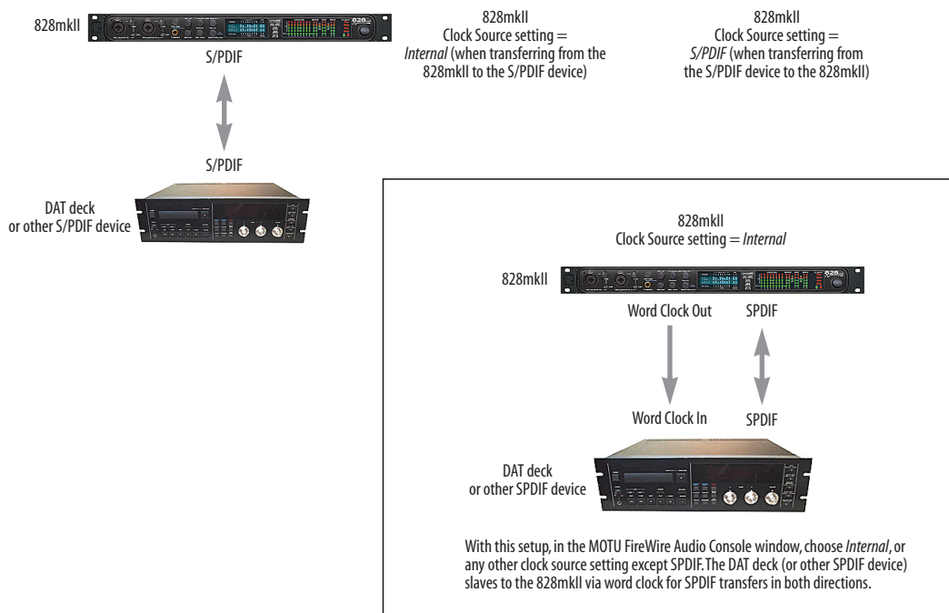
Figure 4-16: Two setups for synchronizing an S/PDIF device with the 828mkII. In the top diagram, sync is achieved via the S/PDIF connection itself. In this case, you have to choose S/PDIF as the 828mkII's clock source when recording from the S/PDIF device. If you don't want to have to worry about switching the Clock Source setting depending on the direction of the S/PDIF transfer, you can slave the S/PDIF device to word clock from the 828mkII or vice versa (not shown). The Word Clock connection maintains sync, regardless of the direction of the transfer.
