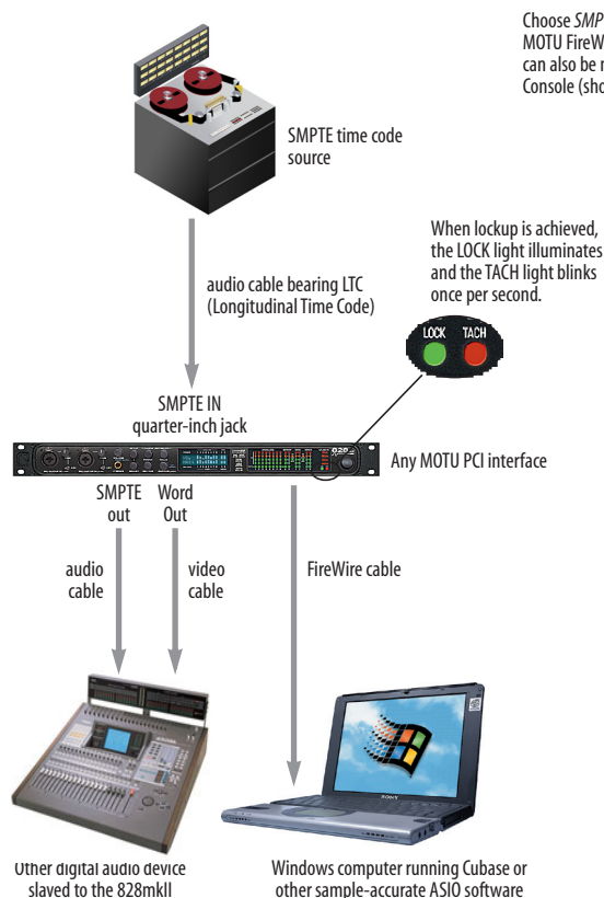
Figure 4-13: Connections for synchronizing the 828mkII directly to SMPTE time code.
