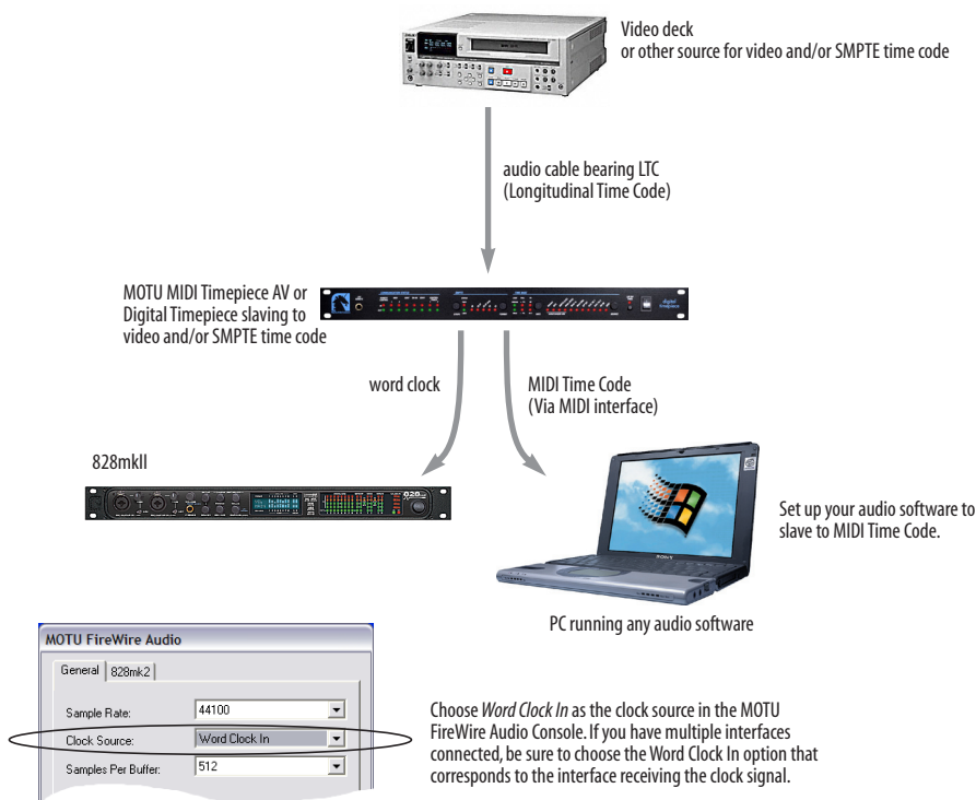
Figure 4-14: If your host audio software does not support sample-accurate sync and the 828mkII's built-in SMPTE sync features, use a universal synchronizer such as the MOTU MIDI Timepiece AV or Digital Timepiece.
