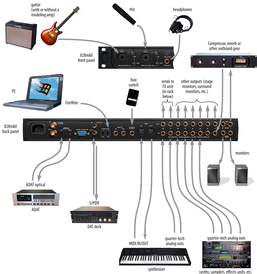
Figure 4-5: A typical 828mkII studio setup.
