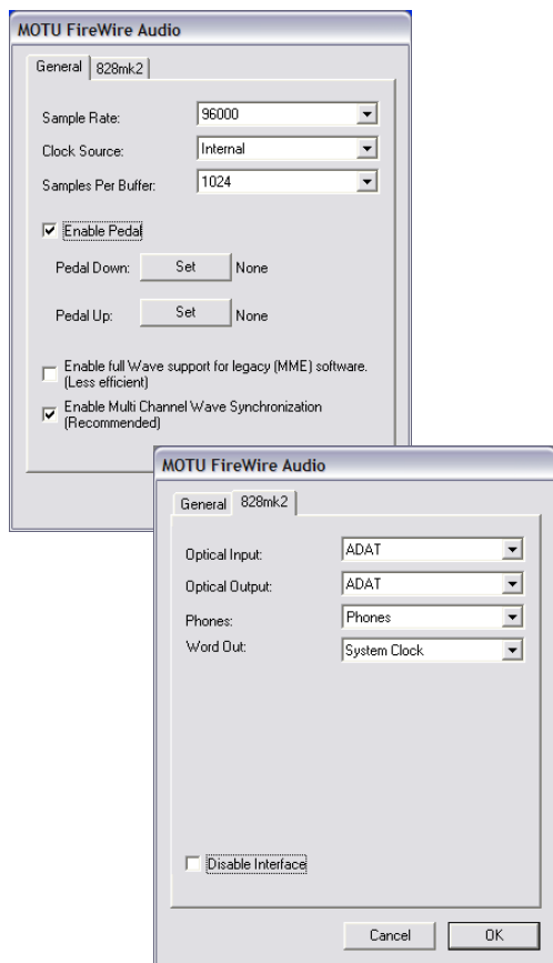
Figure 7-1: The MOTU FireWire Audio Console gives you access to all of the settings in the 828mkII hardware, including the clock source, sample rate and optical I/O enable/disable.
