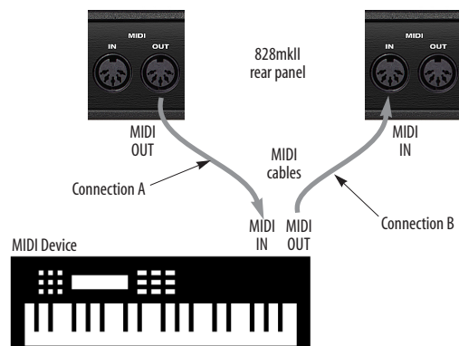
Figure 4-3: Connecting a MIDI device to the 828mkII.
