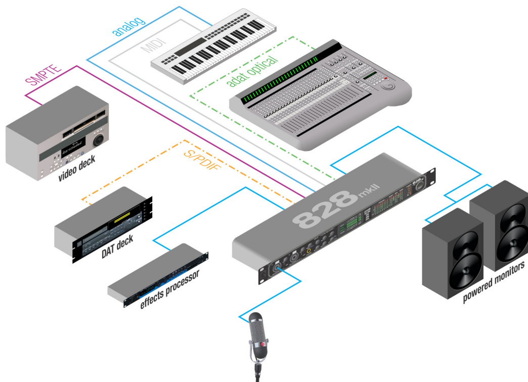
Figure 10-2: An example setup of a system that takes full advantage of CueMix DSP.
