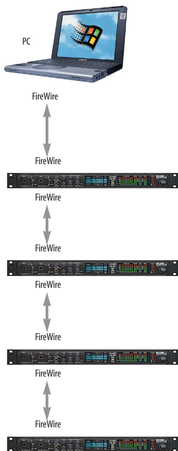
Figure 4-19: Connecting multiple 828mkII's (or other MOTU FireWire audio interfaces) to a computer.
