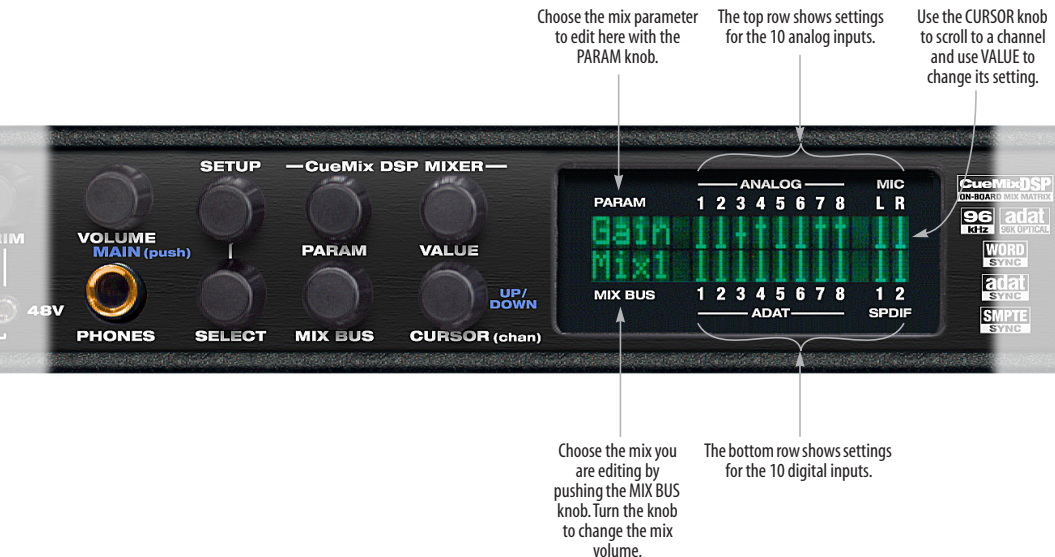
Figure 6-1: The 828mkII front panel controls.
