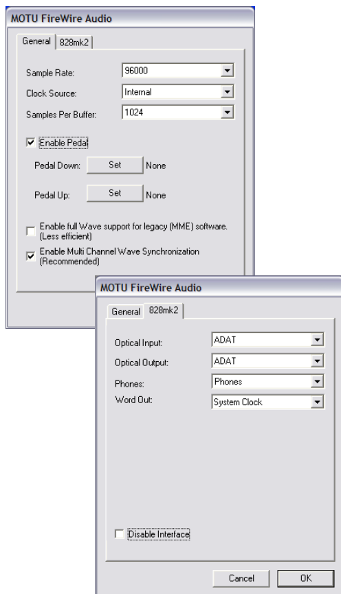
Figure 8-1: The MOTU FireWire Audio Console gives you access to all of the settings in the 828mkII hardware, including the clock source, sample rate and optical I/O enable/disable.
