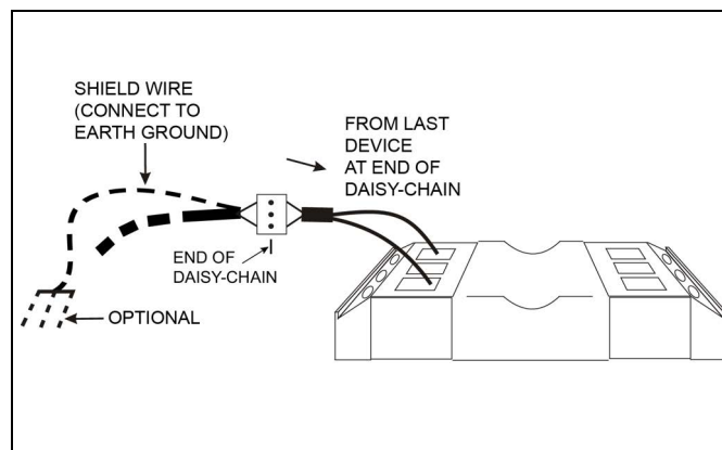
Figure 2 - Termination Block After Last Device on Daisy Chain
