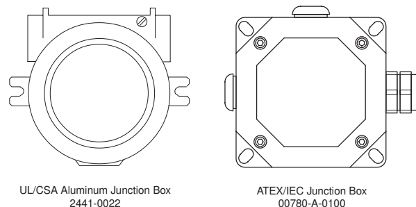
Figure 45. Remote terminal housings
