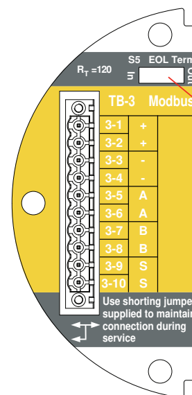
Figure 58. Modbus option board terminal block/jumper switch
