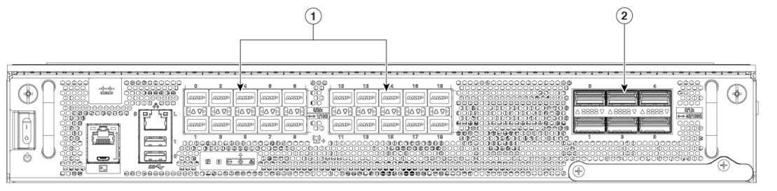
Figure 12: Bay Configuration - C8500 - 20X6C
