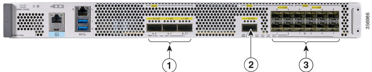
Figure 10: Bay Configuration - C8500-12X4QC
