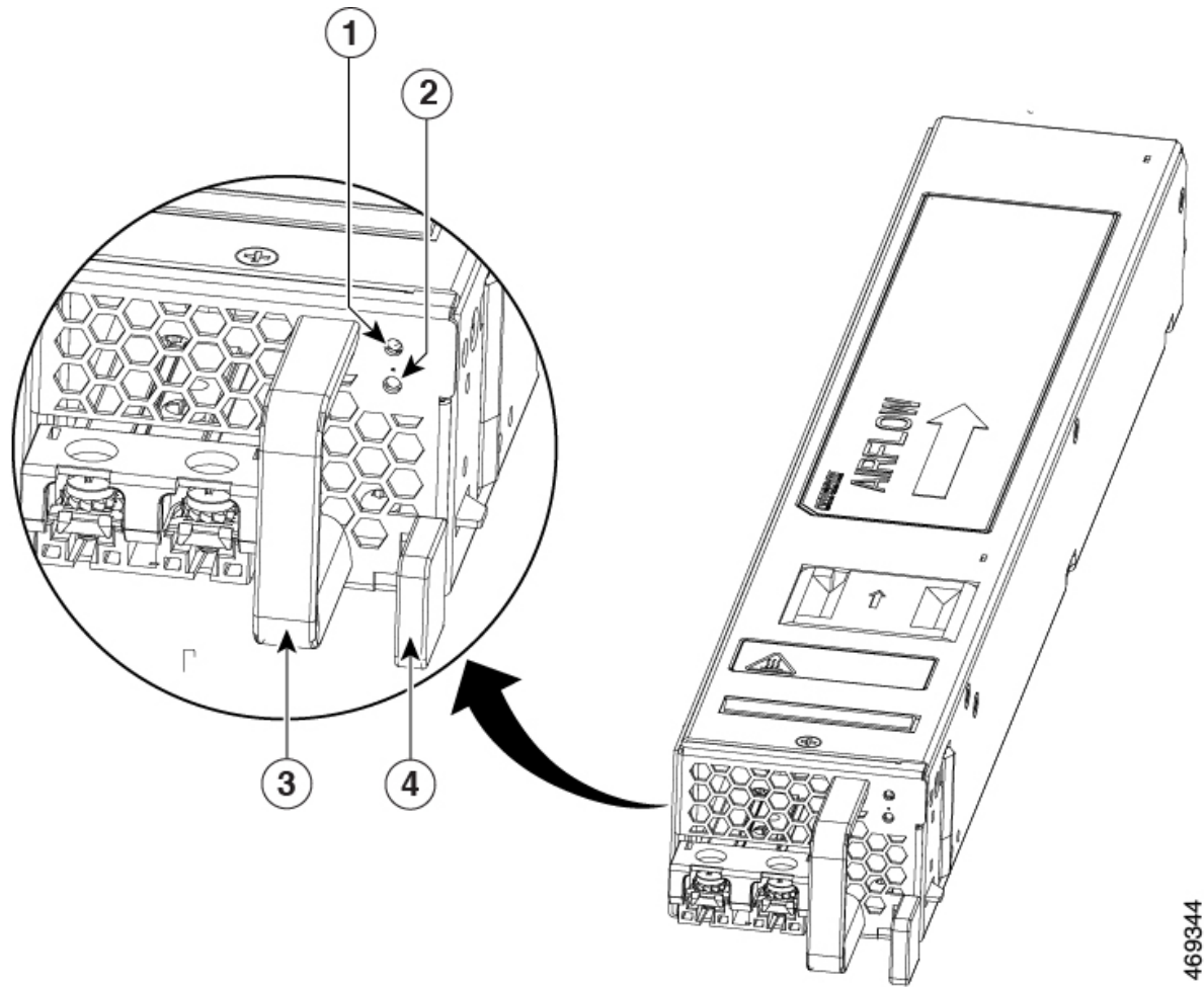
Figure 16: DC Power Supply for C8500-20X6C
