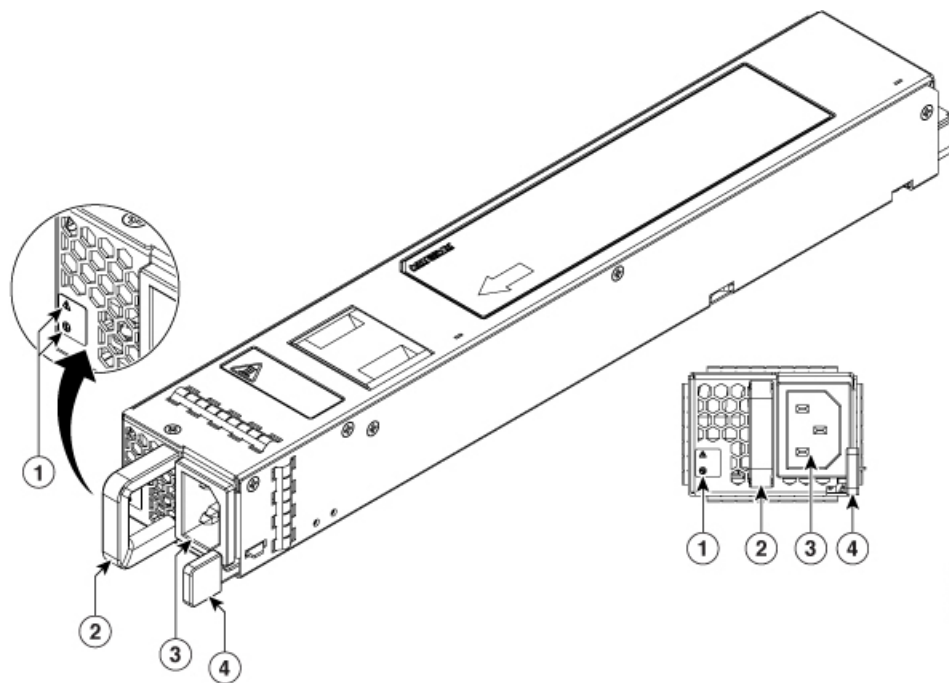
Figure 13: AC Power Supply Used in the Cisco C8500-12X4QC Router
