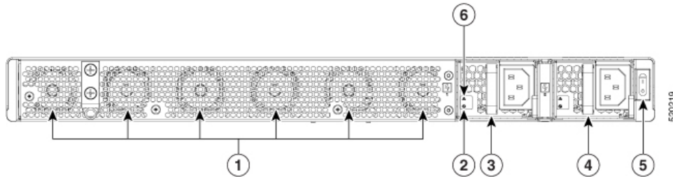
Figure 2: Cisco C8500-12X4QC Rear View
