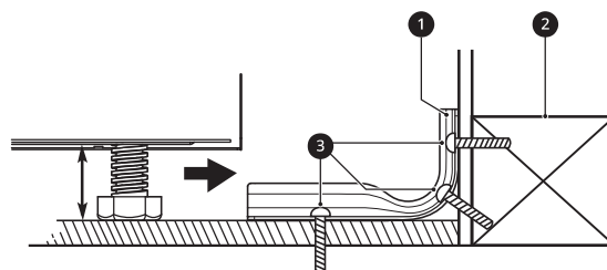
① Anti-tip Bracket
