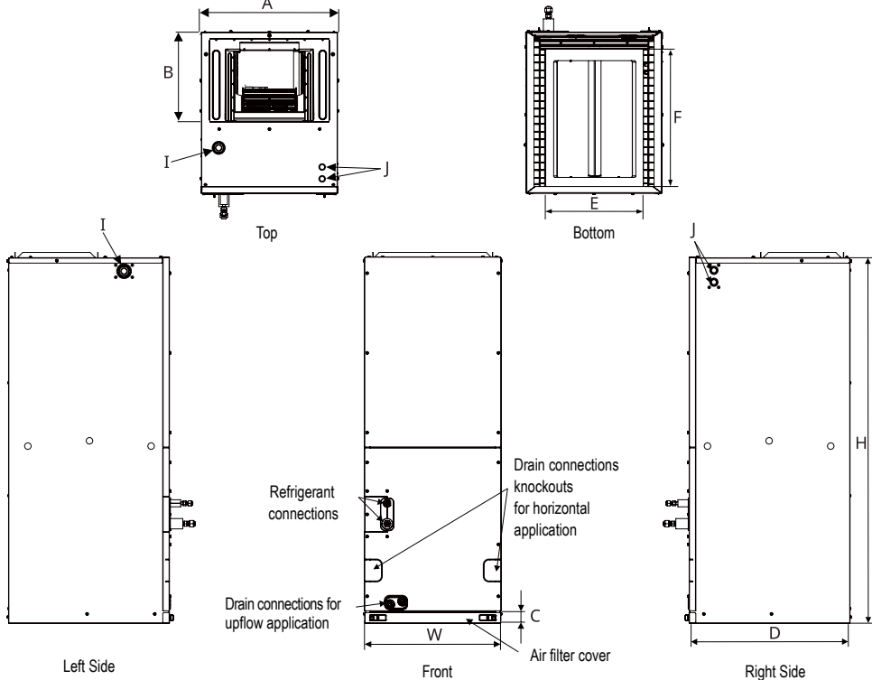
Figure 229: Location of Access Holes and Piping Connections.
