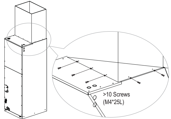
Figure 234: Securing the Ducts to the Unit.
