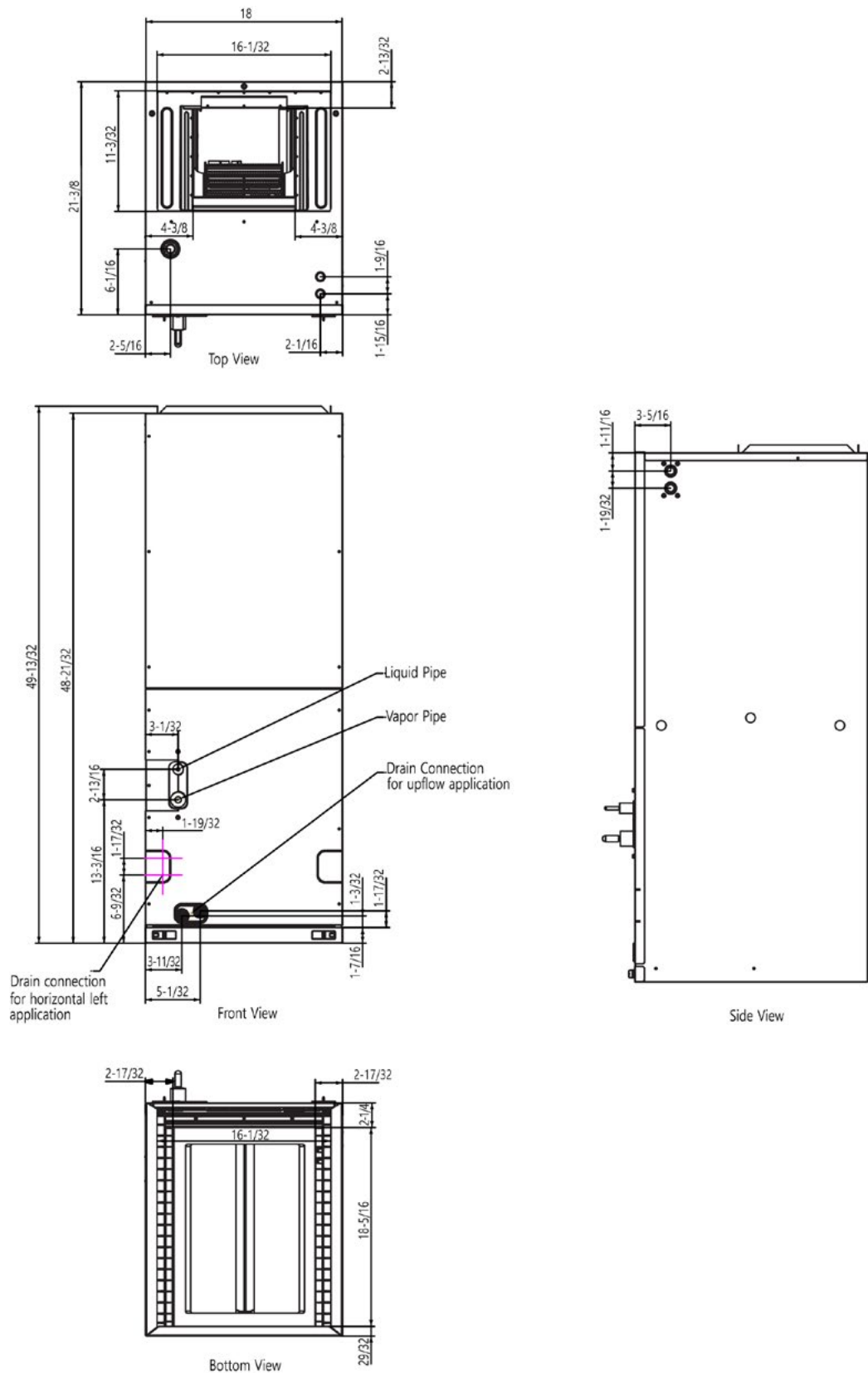
Figure 218: Multi Position Air Handling Unit Dimensions KNMLB121A, KNMLB181A, KNMLB241A.
