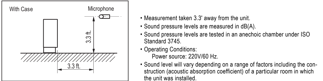
Figure 221: Sound Pressure Level Measurement Location.
