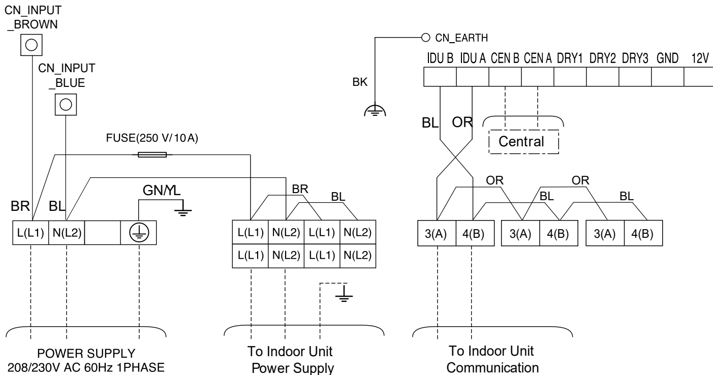
Figure 270: Multi F with LGRED KUMXA181A, KUMXA241A, and KUMXA301A System Power Wiring and Communications Cable.
