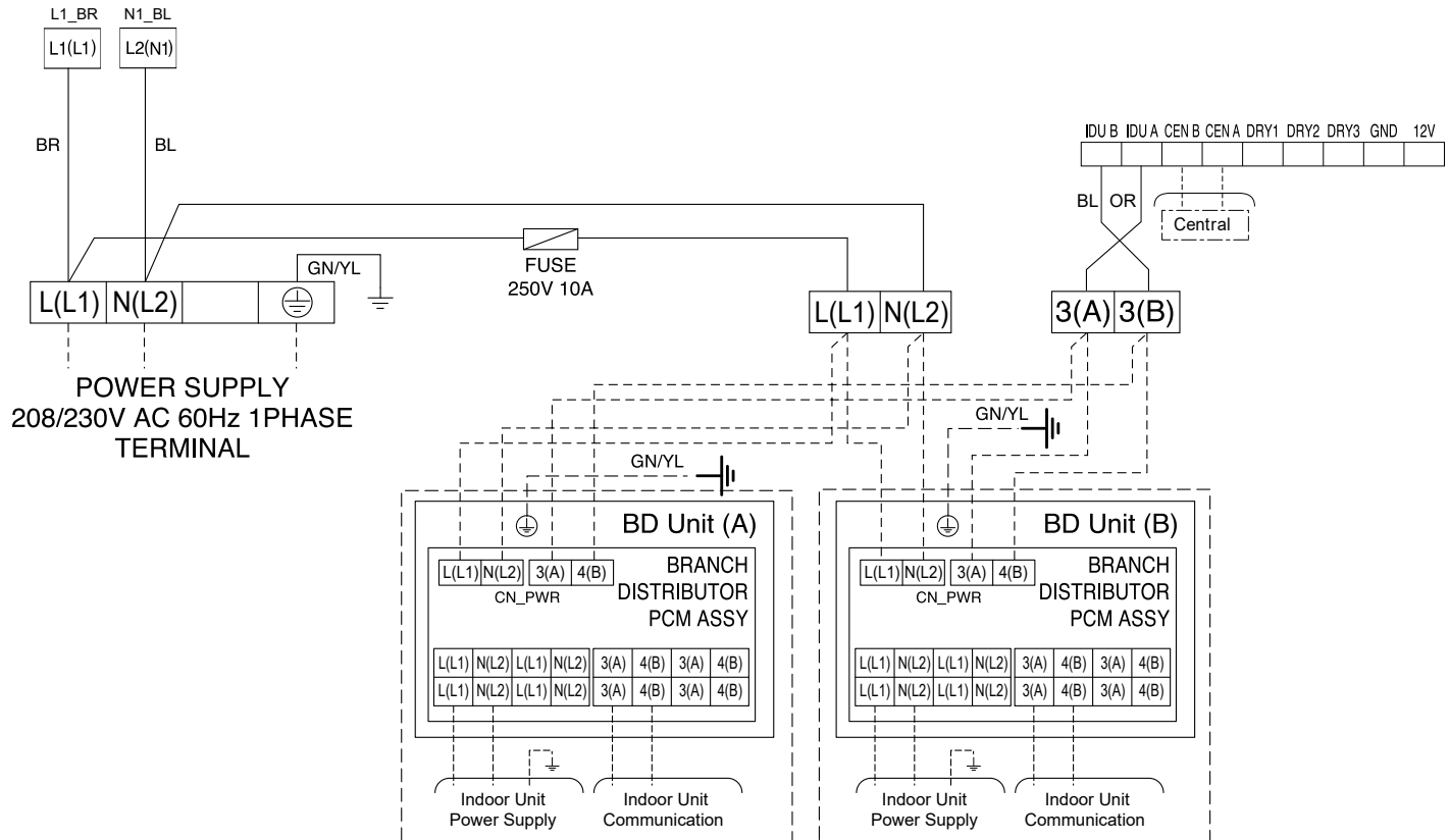
Figure 271: Multi F MAX with LGRED KUMXA361A, KUMXA421A, and KUMXA481A System Power Wiring and Communications Cable.
