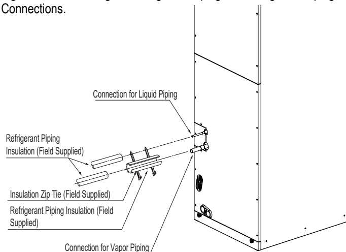
Figure 242: Insulating the Refrigerant Piping and Refrigerant Piping Connections.
