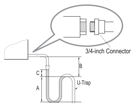
Figure 238: Installing the U-Trap.
