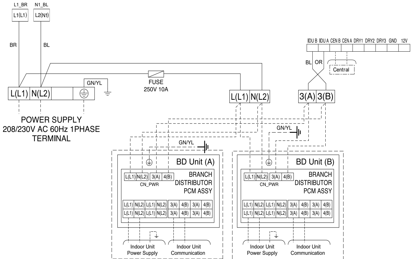
Figure 269: Multi F MAX KUMXB481A, KUMXB541A, and KUMXB601A System Power Wiring and Communications Wiring.
