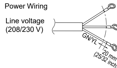
Figure 260: Multi F / Multi F MAX Outdoor Unit Power Wiring.
