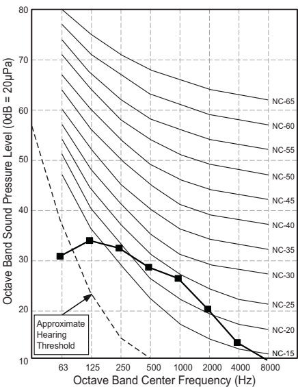
Figure 91: Sound Pressure Level Diagrams. KNMKB091A
