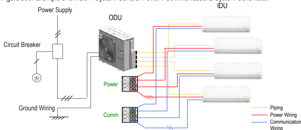
Figure 263: Example of a Multi F System General Power / Communications System Schematic.
