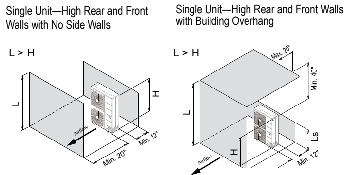
Figure 257: Proper Outdoor Unit Placement and Clearances When There Are Obstacles on the Suction and the Discharge Sides.
