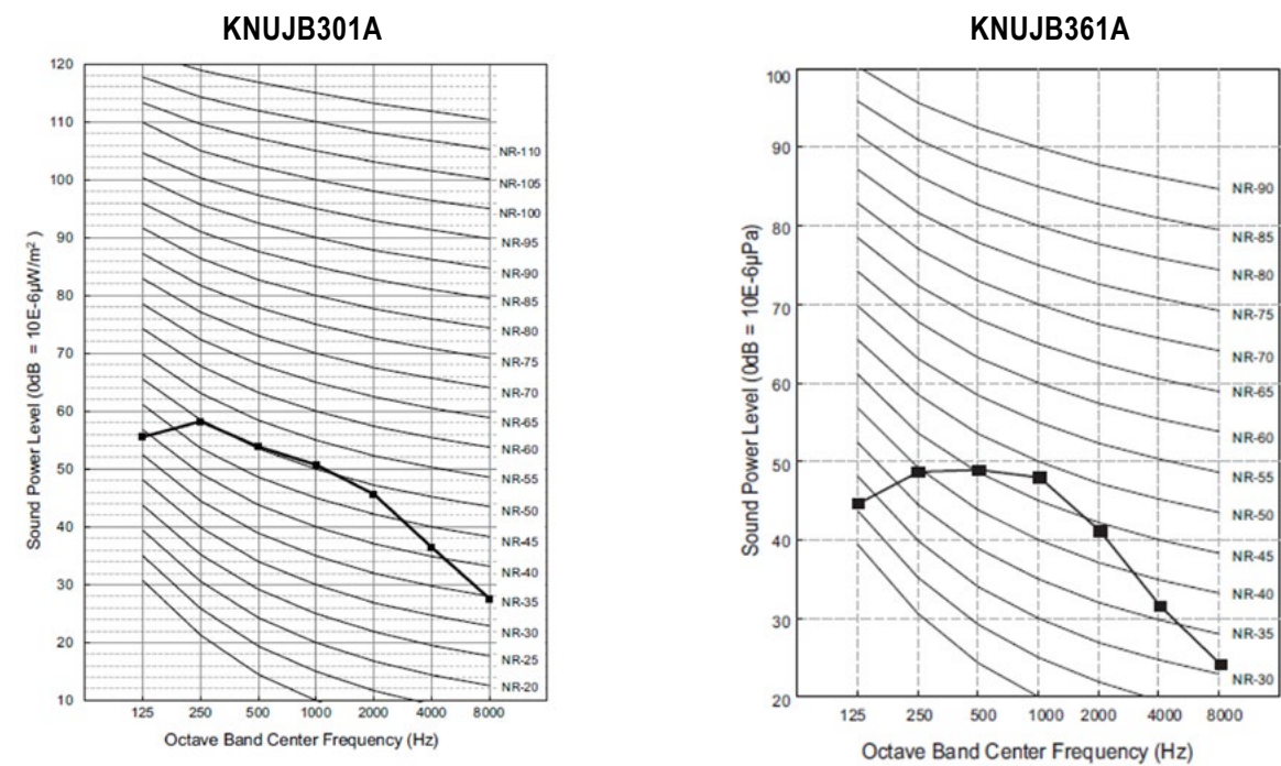
Figure 158: Sound Power Level Diagrams.
