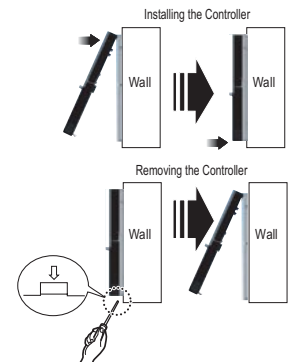
Figure 250: Installing / Removing the Controller.
