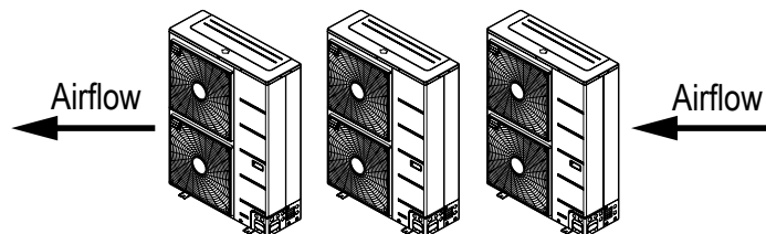
Figure 255: Proper Outdoor Unit Placement and Clearances When There Are Obstacles on the Suction Side.
