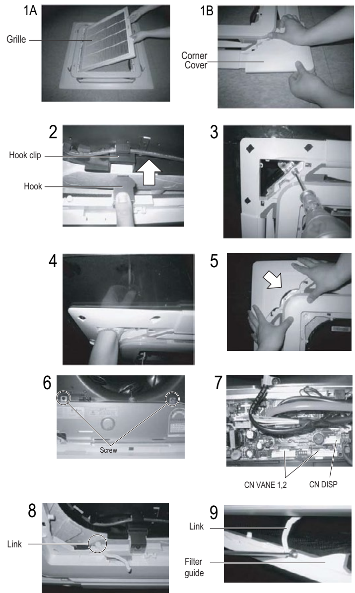
Figure 215: Installing the Decoration Panel.
