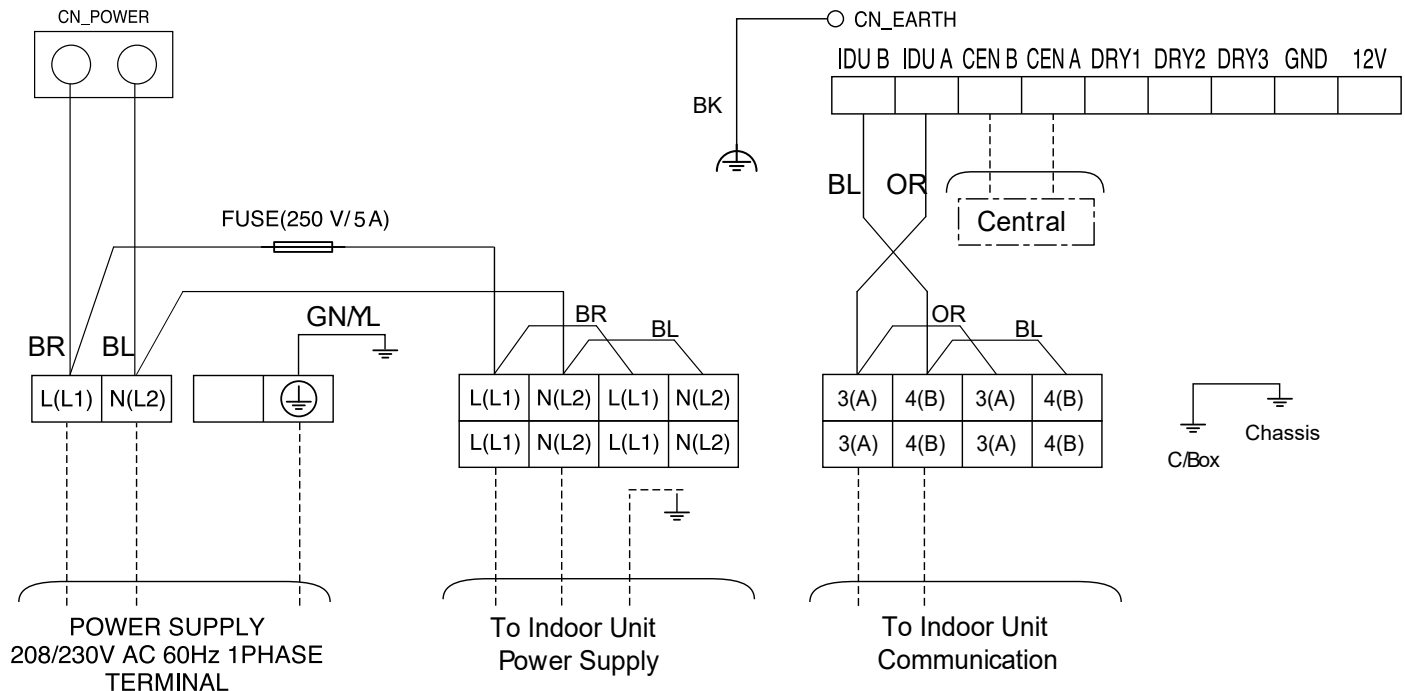
Figure 267: Multi F KUMXB181A and KUMXB241A System Power Wiring and Communications Cable.
