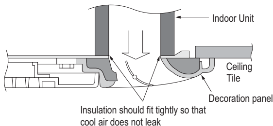
Figure 216: Ensure that no gaps are present between the indoor unit frame and the decoration panel.
