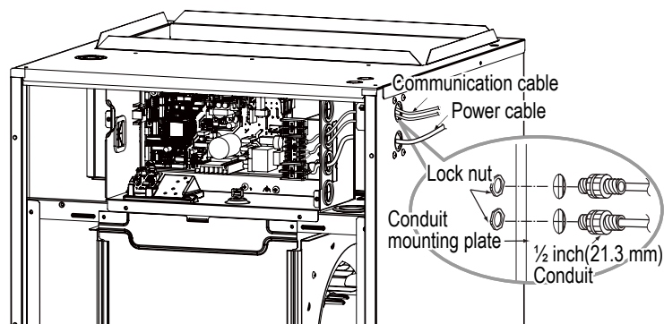
Figure 243: Connecting the Power Wiring and Communications Cable.
