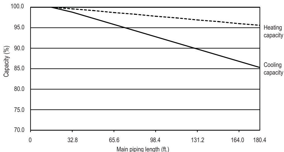
Figure 251: Multi F MAX / Multi F MAX with LGRED Outdoor Unit to Branch Distribution Unit Refrigerant Line Length Derate Chart.
