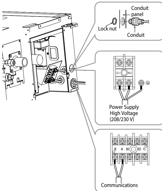
Figure 144: Using a Conduit.
