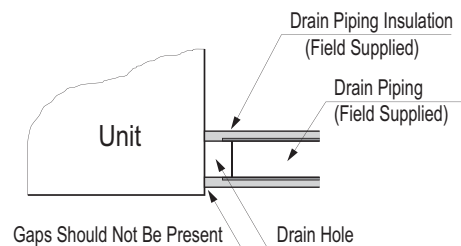
Figure 237: Close up of Drain Piping Connection.
