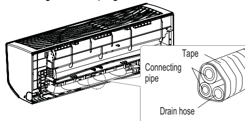
Figure 18: Piping Installed to the Left.
