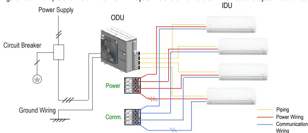
Figure 266: Example of a Multi F MAX with LGRED System General Power / Communications System Schematic.
