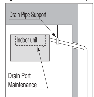
Figure 134: Indoor Unit Drain Piping.
