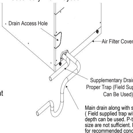
Figure 239: Vertical Primary and Secondary Drain Layout.
