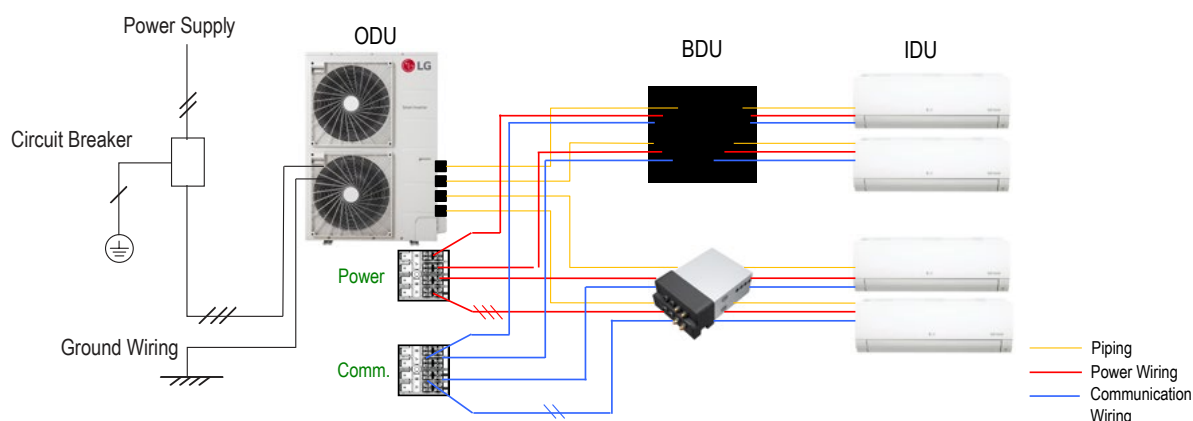
Figure 266: Example of a Multi F MAX with LGRED System General Power / Communications System Schematic.
