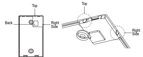
Figure 250: Installing / Removing the Controller.
