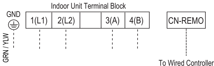
Figure 246: Wired Controller Connection on the Indoor Unit Terminal Block.
