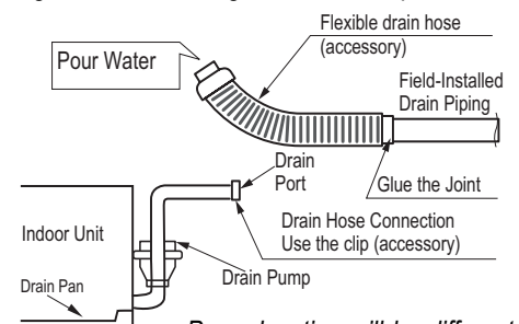
Figure 106: Checking the Drain Pump.
