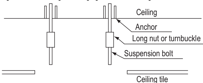
Figure 199: Installing the Hanging Bolt in the Ceiling.
