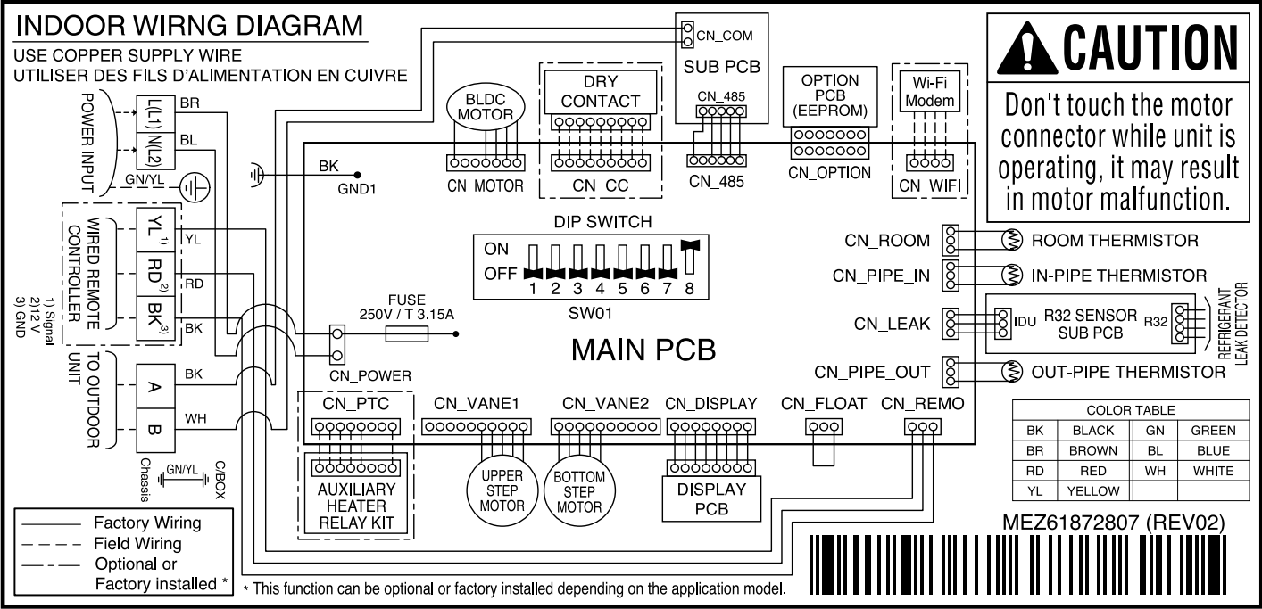
Figure 72: Multi F Low Wall Console KNUQB091A, KNUQB121A, and KNMQB151A Indoor Units Wiring Diagram.
