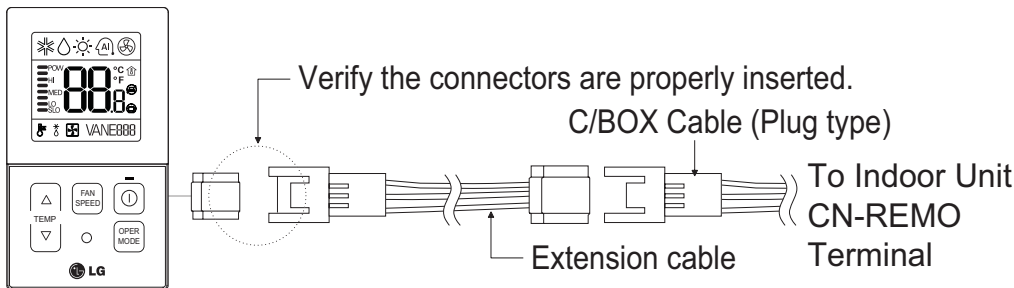
Figure 245: PZCWRC1 LG Wired Remote Extension Cable.
