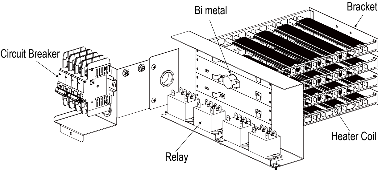
Figure 220: Typical Multi Position Air Handling Unit Optional Electric Heater Accessory.
