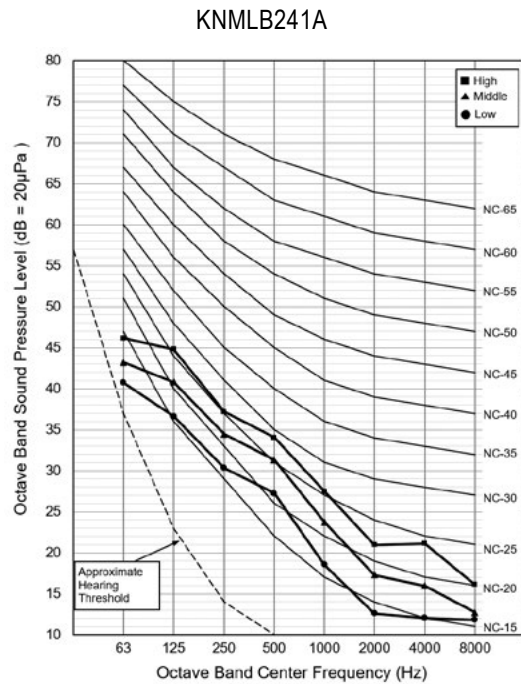
Figure 223: Sound Pressure Level Diagrams - continued.
