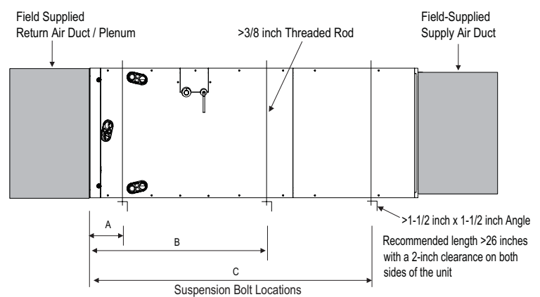
Figure 233: Typical Horizontal Right Installation.
