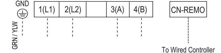
Figure 210: Wired Controller Connections on the Indoor Unit Terminal Block.
