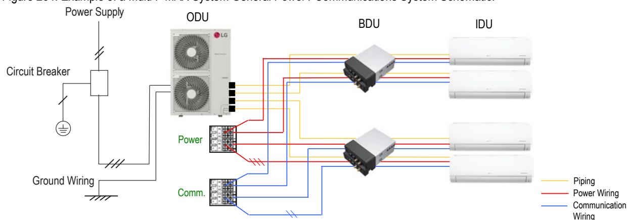
Figure 264: Example of a Multi F MAX System General Power / Communications System Schematic.
