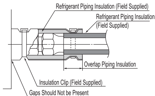
Figure 241: Close Up of Refrigerant Piping Connection Insulation.
