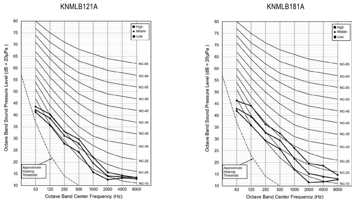
Figure 222: Sound Pressure Level Diagrams.
