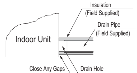
Figure 103: Drain Connection.
