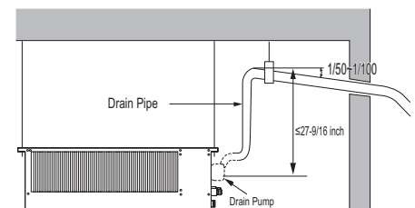
Figure 104: Indoor Unit Using Drain Pump.
