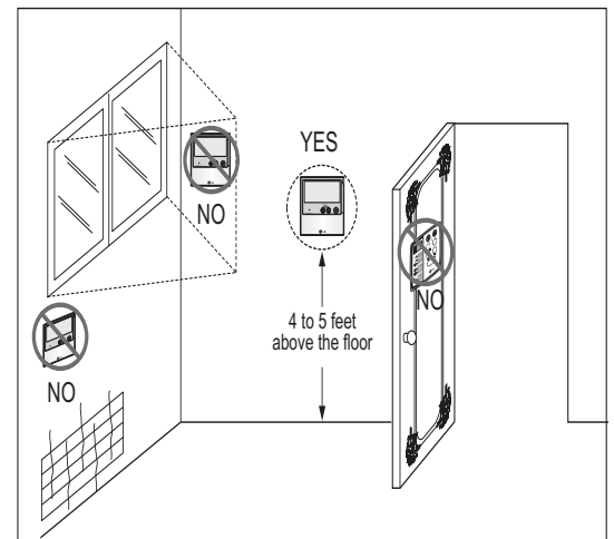
Figure 25: Proper Location for the Wired Controller.
