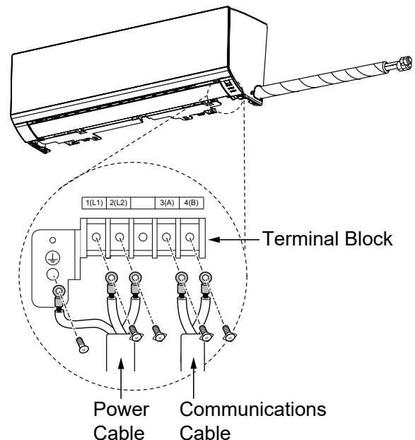
Figure 54: Connecting Power Wiring / Communications Cable.
