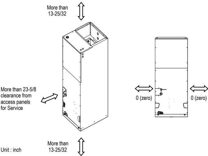
Figure 227: Clearance Requirements.
