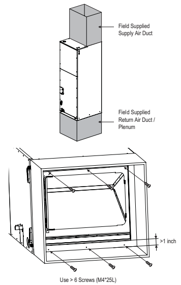
Figure 230: Vertical Installation / Attaching the Bottom Duct.
