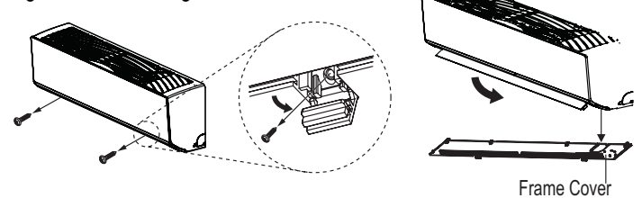
Figure 16: Removing the Frame Cover.
