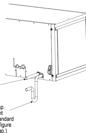
Figure 240: Horizontal Primary and Secondary Drain Layout.
