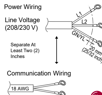
Figure 262: Power Wiring and Communication Wiring from ODU to IDU / BDU (Multi F MAX Only), and from the BDU to the IDU (Multi F MAX Only) GREATER THAN 130 feet
