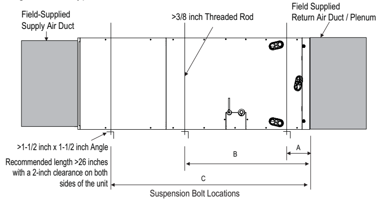
Figure 232: Typical Horizontal Left Installation.
