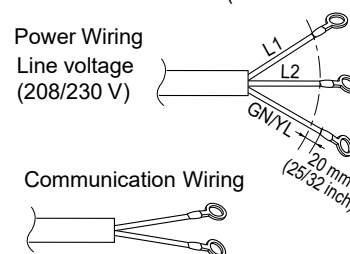
Figure 262: Power Wiring and Communication Wiring from ODU to IDU / BDU (Multi F MAX Only), and from the BDU to the IDU (Multi F MAX Only) GREATER THAN 130 feet
