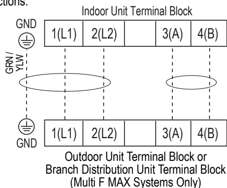
Figure 244: Indoor Unit to Outdoor Unit / Branch Distribution Unit (Multi F MAX systems only) Power Wiring / Communications Cable Connections.
