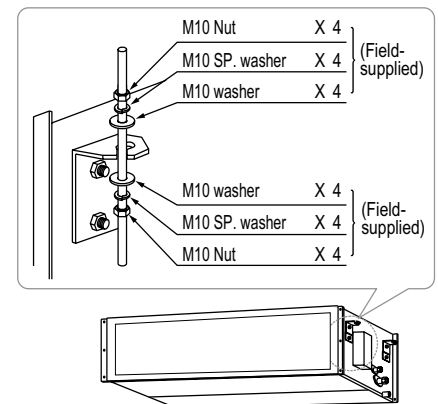
Figure 133: Hanging the Indoor Unit.
