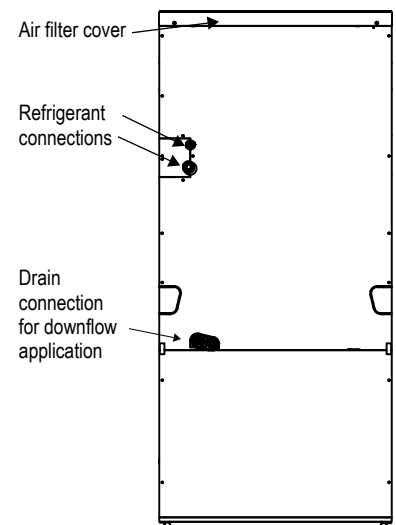
Figure 231: Chassis after Downflow Field Conversion.
