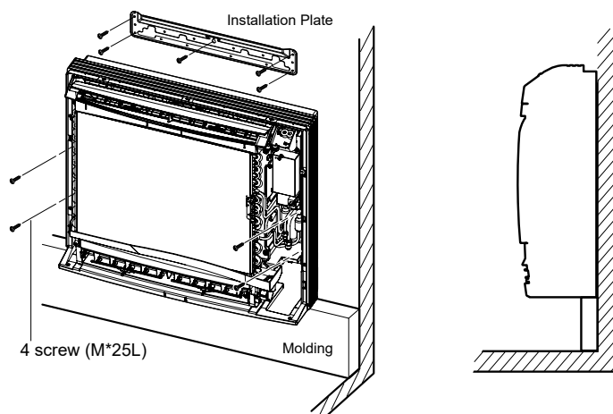
Figure 75: Wall Installation.
