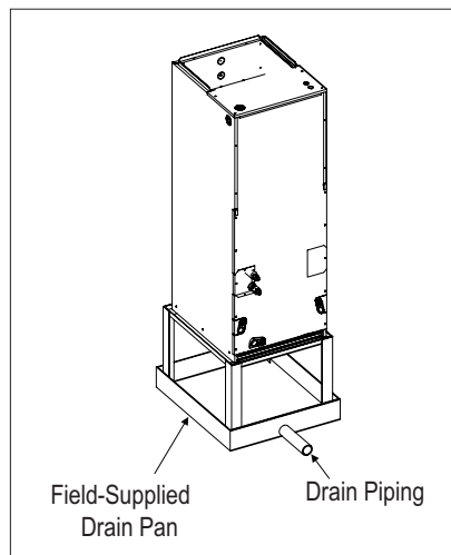
Figure 235: Typical Vertical Up/Down Installation Drain System.
