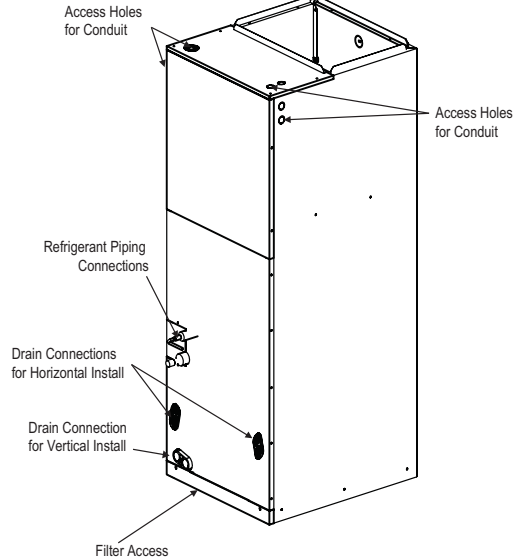
Figure 228: General and Duct Connection Dimensions.
