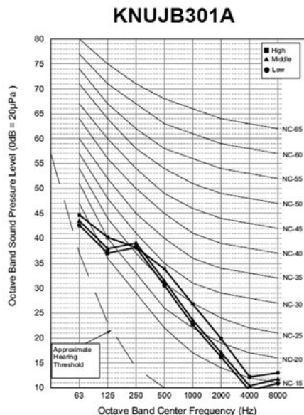
Figure 157: Sound Pressure Level Diagrams.
