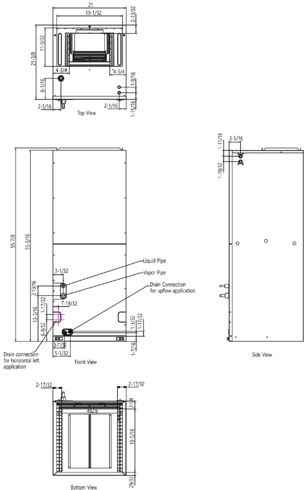
Figure 219: Multi Position Air Handling Unit Dimensions, KNMLB301A, KNMLB361A.
