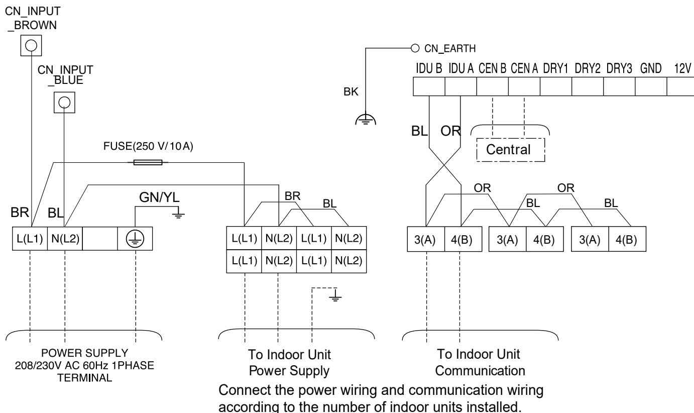
Figure 268: Multi F KUMXB301A and KUMXB361A System Power Wiring and Communications Wiring.
