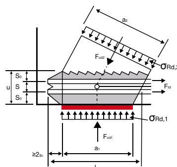
Fig. 6.4: Strut-and-tie model for moment resisting connctions (red = tension, green = compression) according to EC2-1-1 [1]
