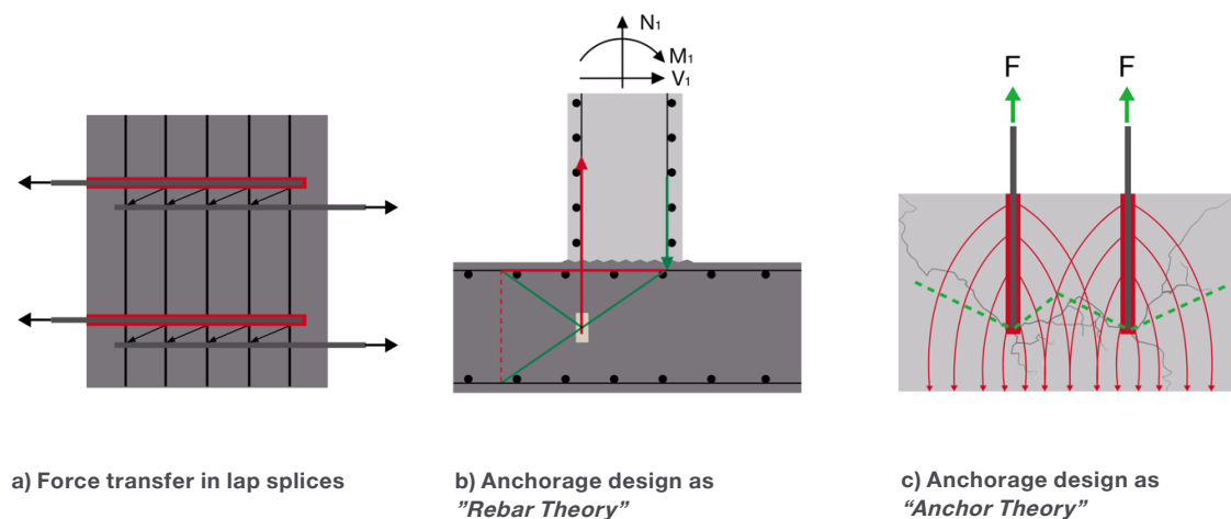
Fig. 2.12: Load-bearing mechanisms
