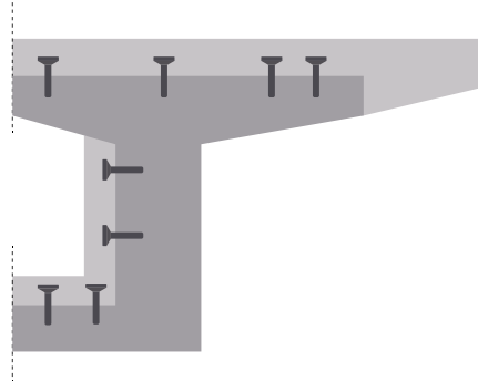
d) Foundations strengthening
