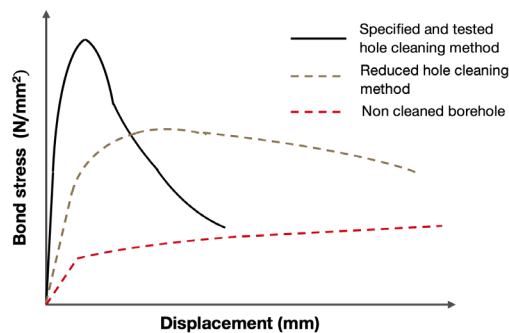
b) Influence of cleaning methods on bond stress Vs displacement
