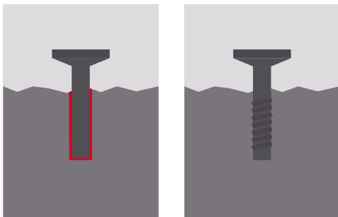
a) Existing concrete-bonded fastener &amp; concrete screw
