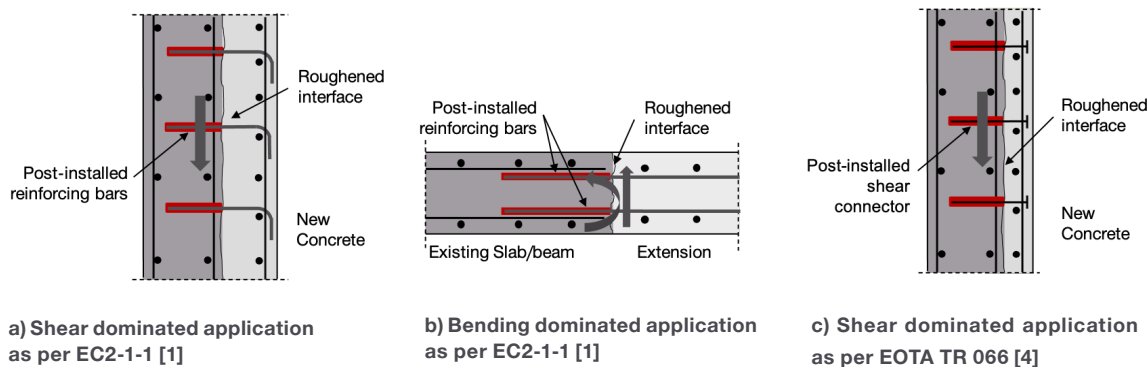
Fig. 7.1: Interface shear transfer in different applications
