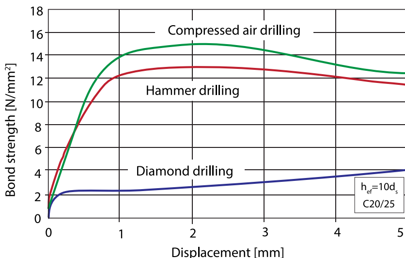
Fig. 9.6: Influence of drilling method on the bond-displacement behavior of a post-installed rebar with embedment of 10Φ in low-strength concrete and cleaned hole [5]
