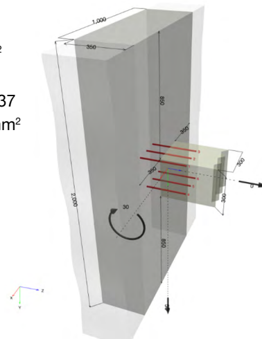
Fig. 6.19: Beam to Wall connection
