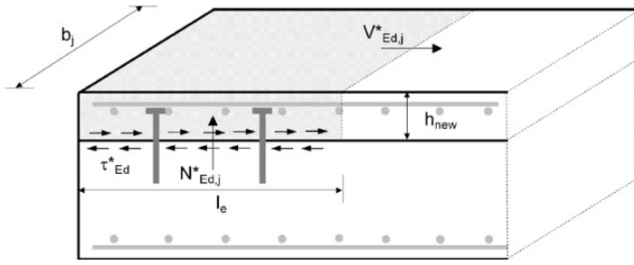
Fig. 7.4: Schematic representation of connectors to resist restraint forces along the perimeters (ref. EOTA TR 066 [4])
