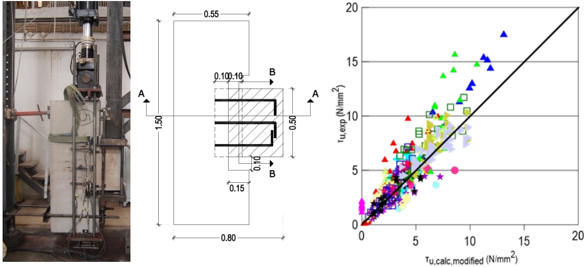
a) Typical test specimen and setup used to derive the shear-friction model (dimensions are in m)
