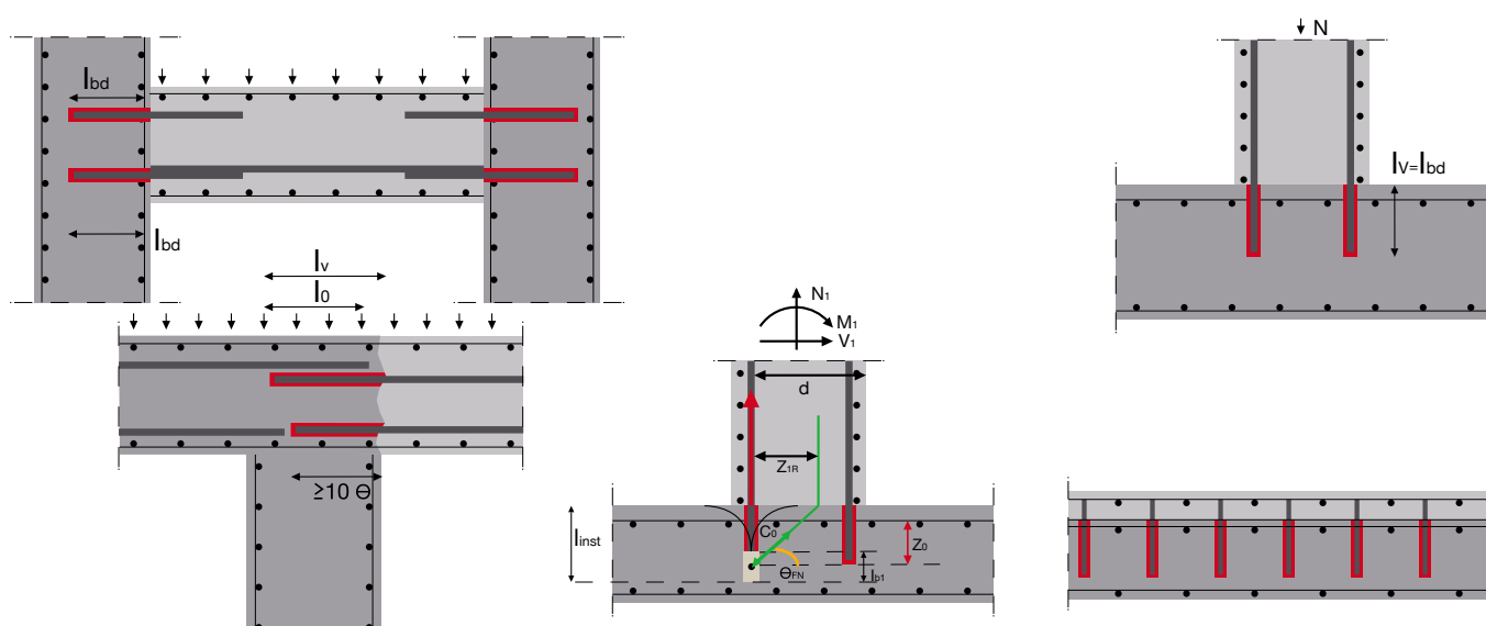
Fig. 3.3: Post-installed rebar applications covered by EC2-1-1 [1] design provisions
