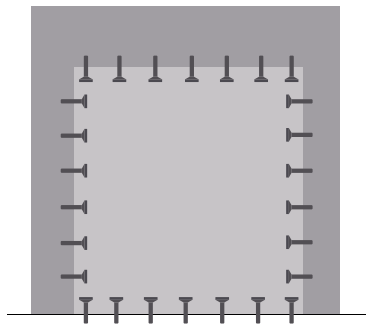
c) Connection of shear walls in RC frame
