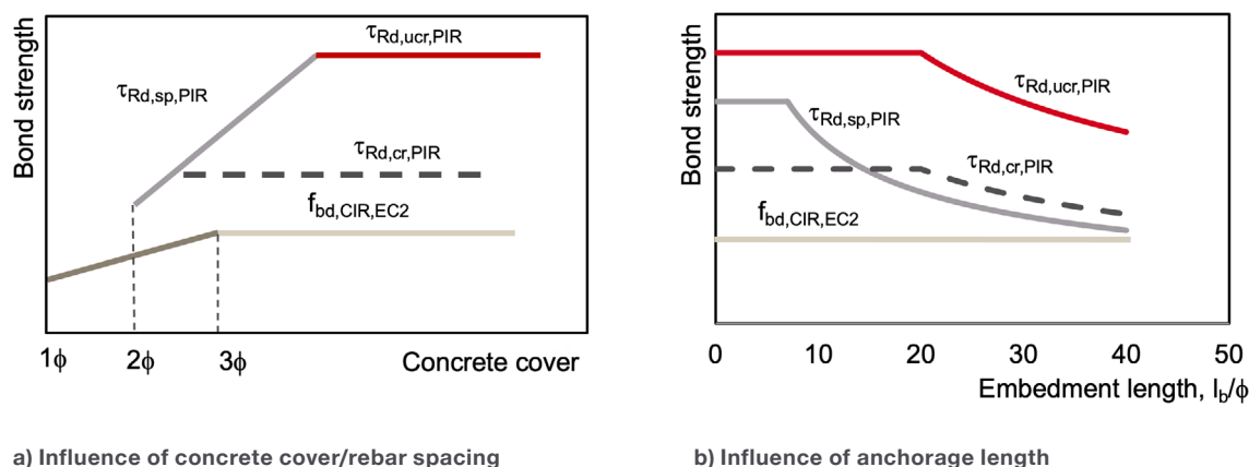
Fig. 3.4: Bond strength performance
