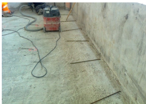
b) Connection of overlay to perimetral walls
