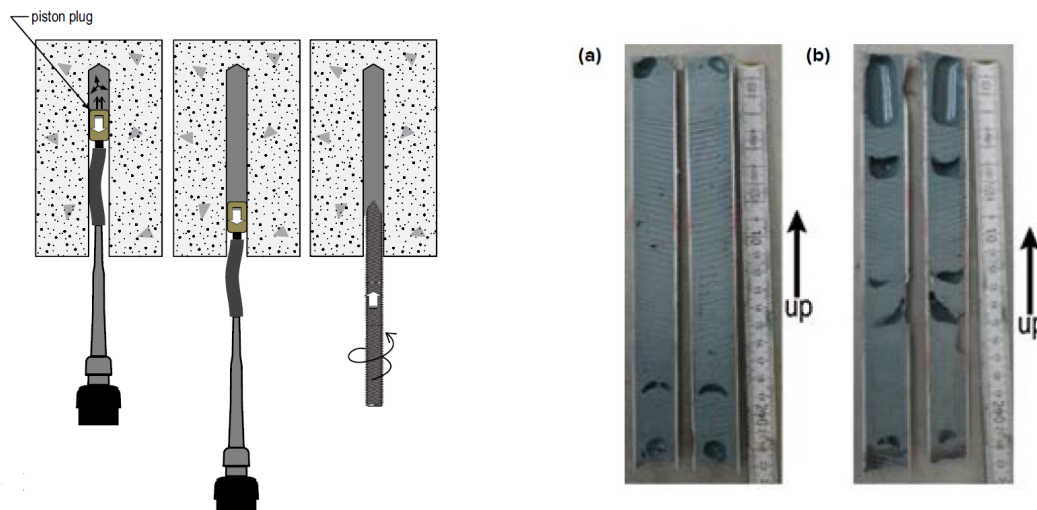
Fig. 9.14: (I) Usage of piston plug for adhesive injection (II) Images showing (a) successful injection of adhesive ( \leq 10\% voids) using piston plug & (b) failed injection of adhesive ( > 10\% voids) [49]
