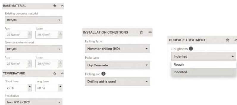
Fig. 8.4: Base material properties and installation conditions
