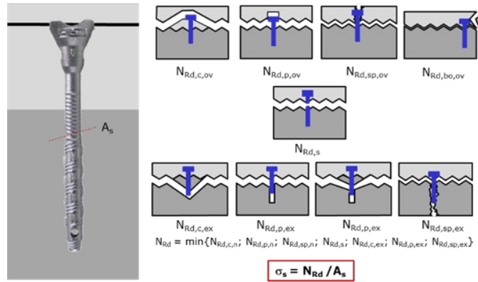
Fig. 7.7: Anchor verifications to be carried out to determine \sigma_s
