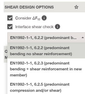
Fig. 8.10: Shear design of interface in PROFIS
