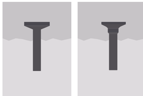
b) Overlay concrete-mechanical interlock (anchor &amp; shaped head)
