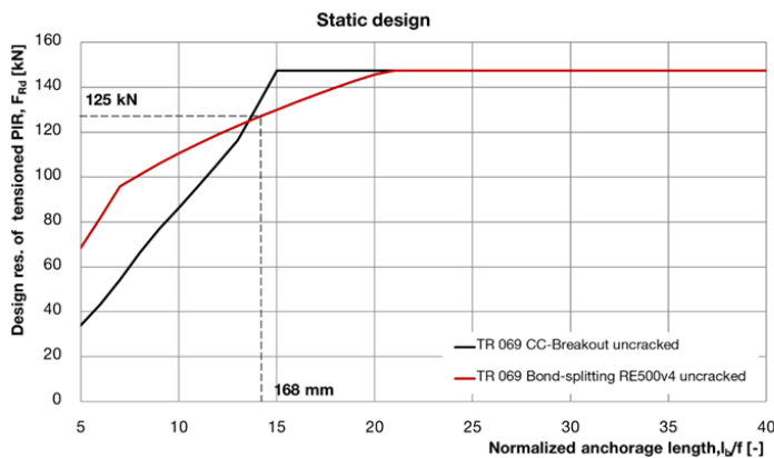
Fig. 6.20: Graphic representation of the required anchorage length for the static load case
