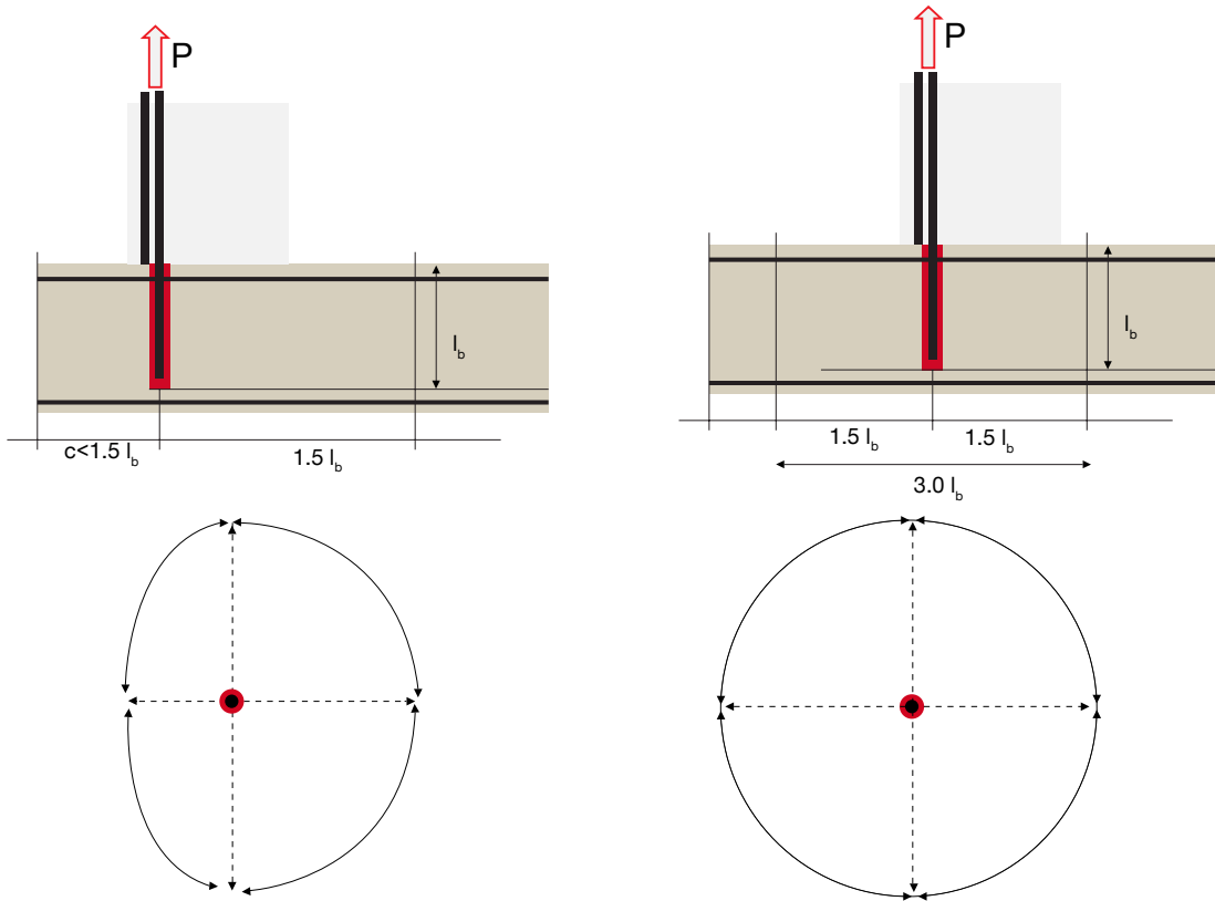
Fig. 6.7: Effect of proximity to concrete edge
