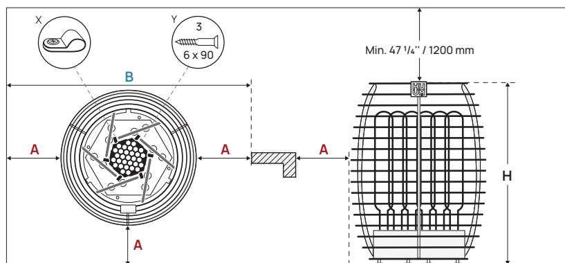
Figure 1 Positioning of the heater
