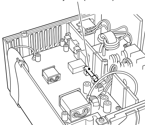
Circuitry fuse (FGB 5 A)
