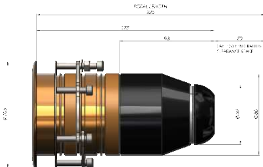
General Dimensions of the Rear Enclosure Assembly
