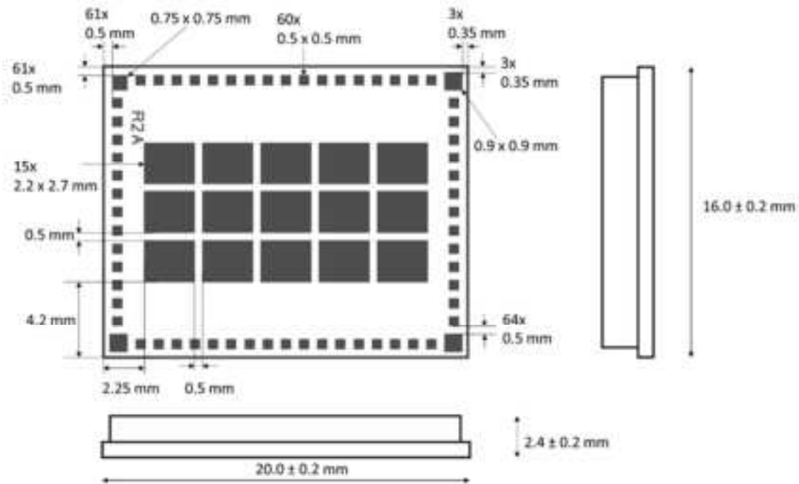
Figure 10. Package dimensions
