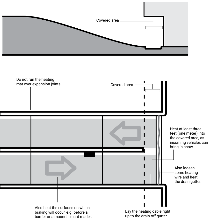
Example of Snow Melting for a Parking Ramp
