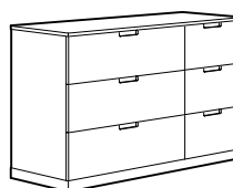
NORDLI 6-drawer dresser* Total size: W47¼×D18½×H29⅞". White 093.841.88 Anthracite 493.841.91
