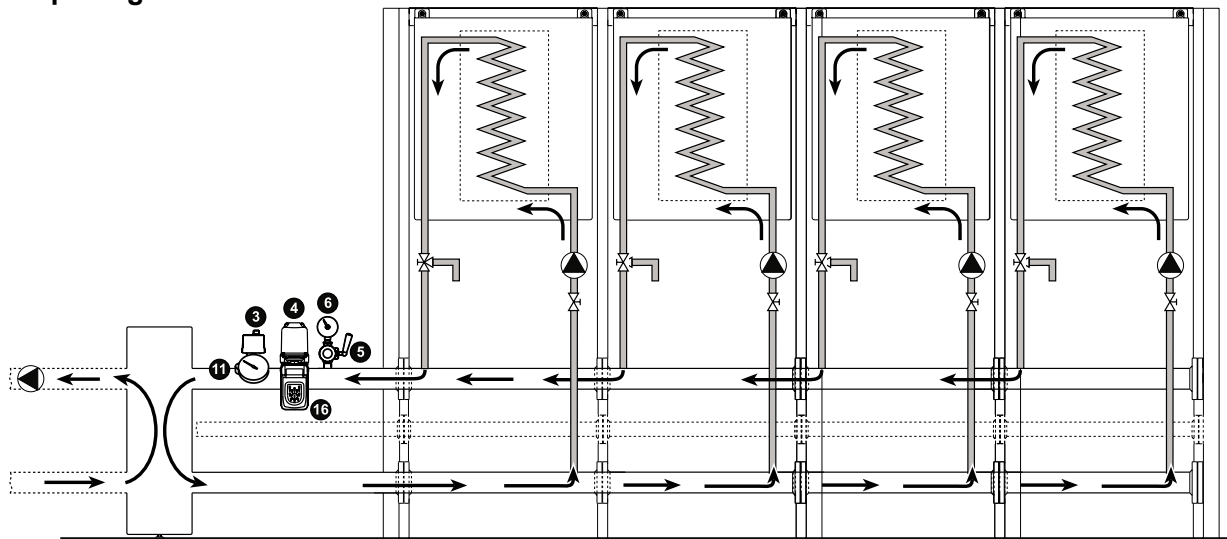
Concept diagram with 4 boilers
