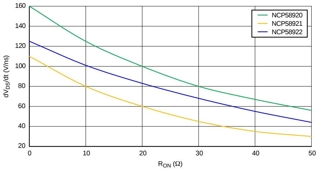
Figure 18. Half-Bridge Power Module Switch-node dv/dt vs. R_{ON} for All Devices in Family
