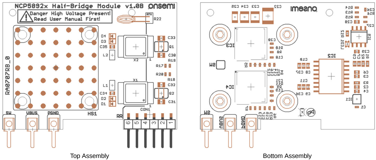
Figure 14. HB Power Module PCB Assembly
