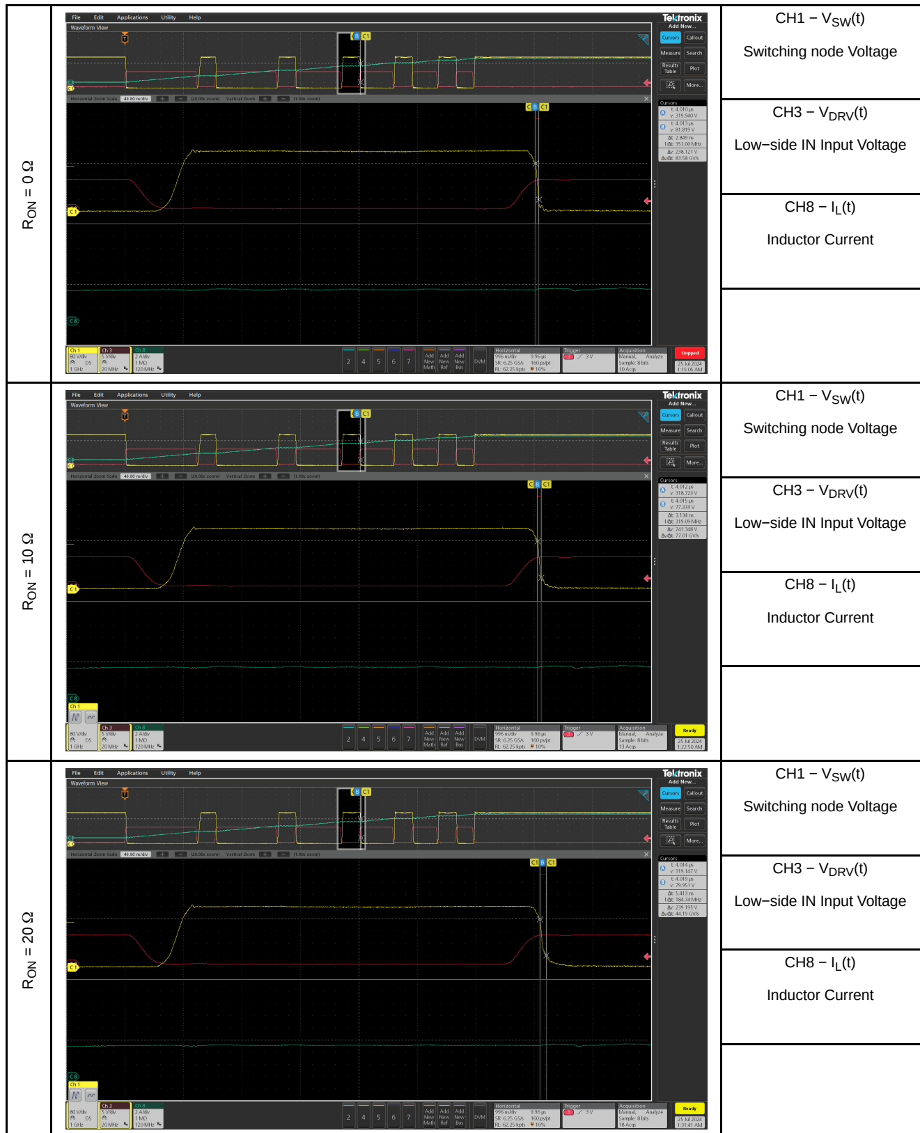
Figure 16. Half-Bridge Power Module Waveform vs. Various R_{ON} Resistance 0–20 \Omega (NCP58921)
