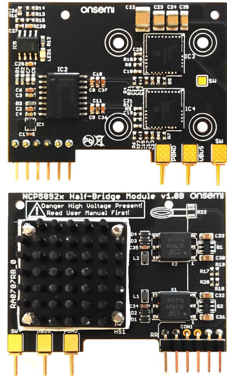
Figure 1. Board Photo
