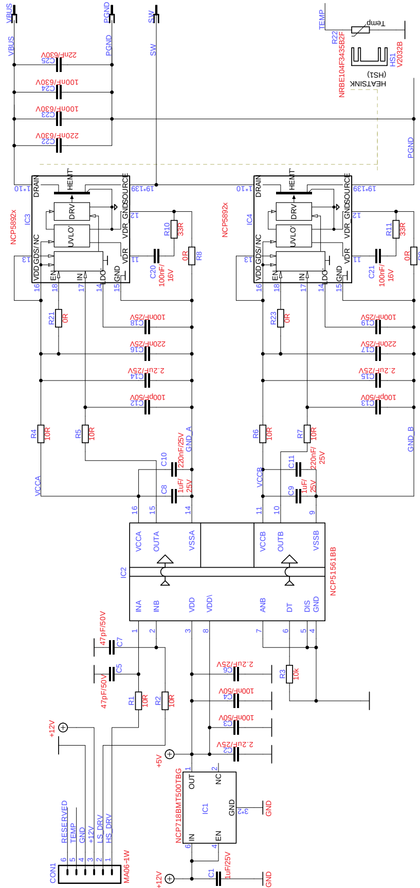
Figure 7. Isolated Driver and Half-bridge Power Stage Schematic Diagram
