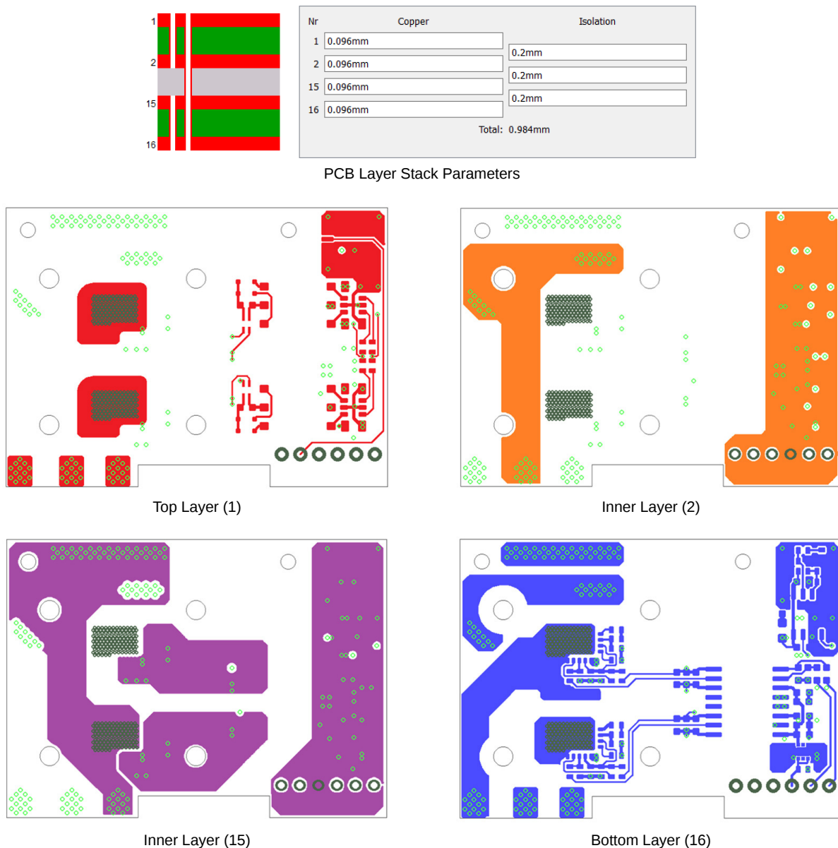
Figure 13. HB Power Module PCB Layout
