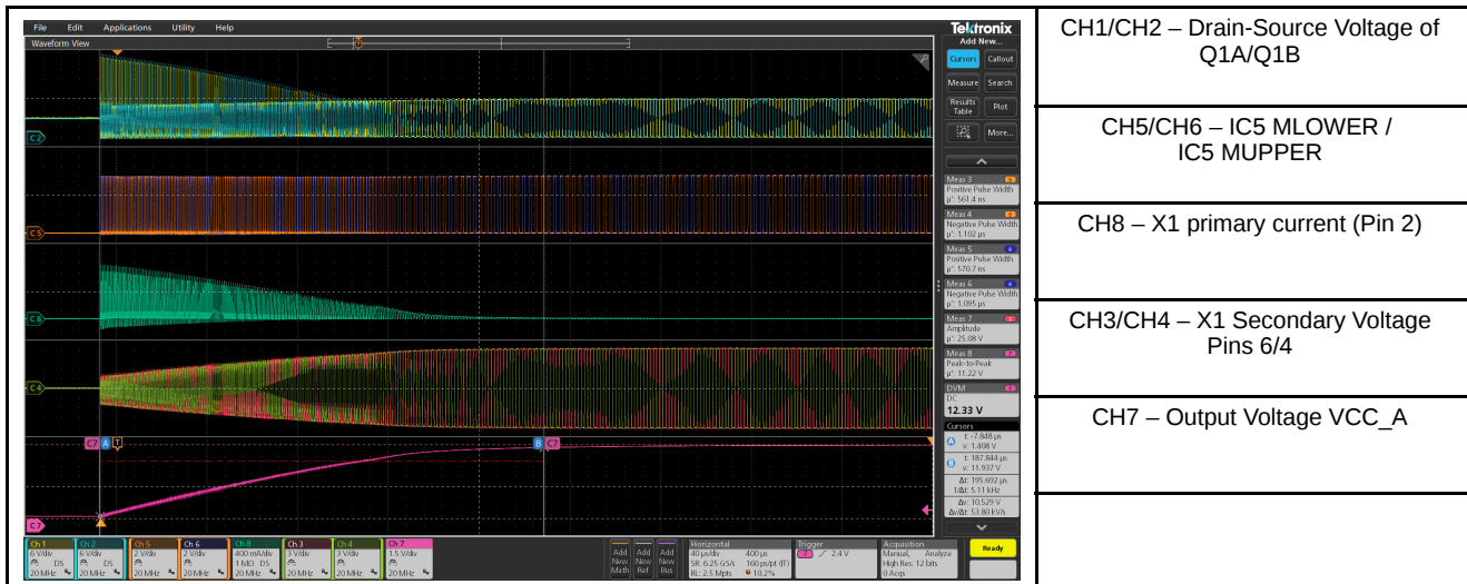
Figure 11. DC-DC Converter Start-up Sequence Waveforms
