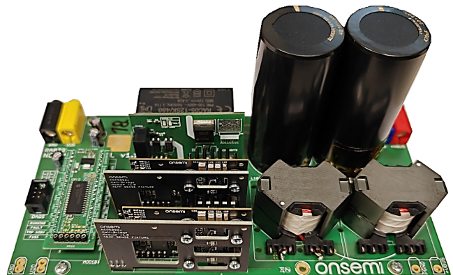
Figure 22. Half-Bridge Power Module Application Examples
