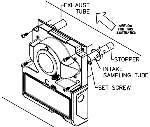
FIGURE 2. DH-100 MOUNTING
