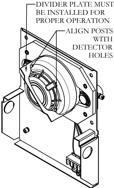
FIGURE 9. DH-100-A COVER REMOVED
