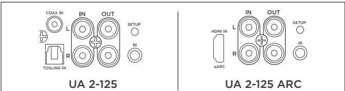
Figure 2: Source Connections
