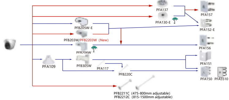
Camera Adapter Wall Mount Ceiling Mount Junction Box Pole/Corner Mount
