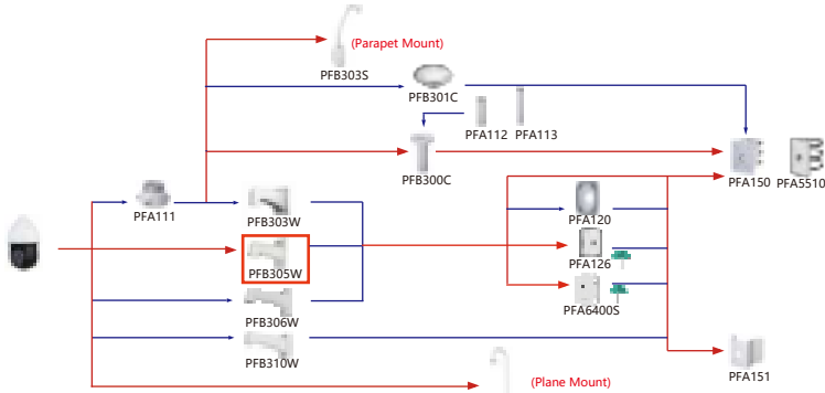
Camera Adapter Wall Mount Ceiling Mount Junction Box Pole/Corner Mount
