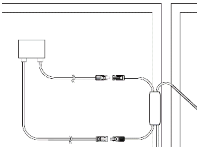
Figure 4.3 Connecting PEFS-PL80P-11 and solar module
