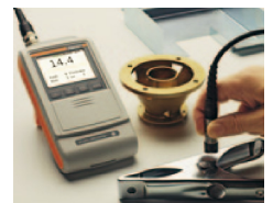
DUALSCOPE® FMP40 using probe FD13H
