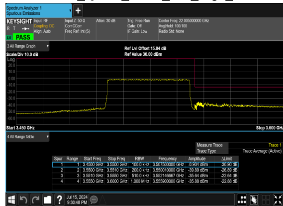
N77(50M)_DFT-s- OFDM_QPSK_Outer_Full_High_CH
