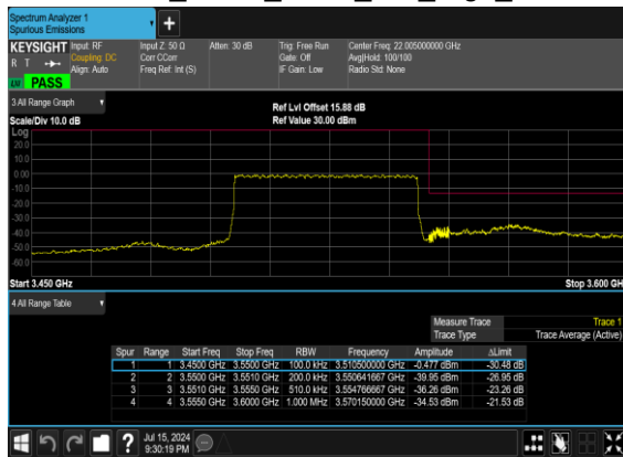
N77(50M)_DFT-s- OFDM_BPSK_Outer_Full_High_CH
