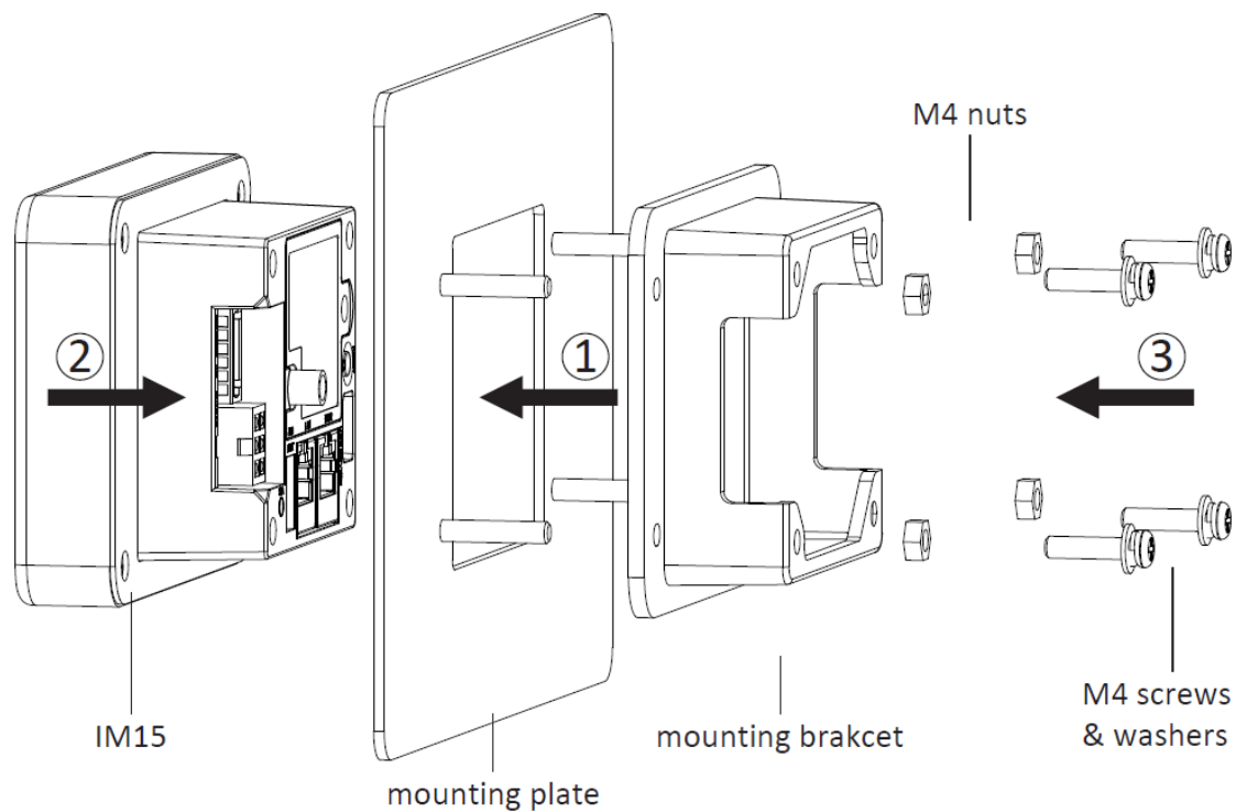
Figure 6: device installation
