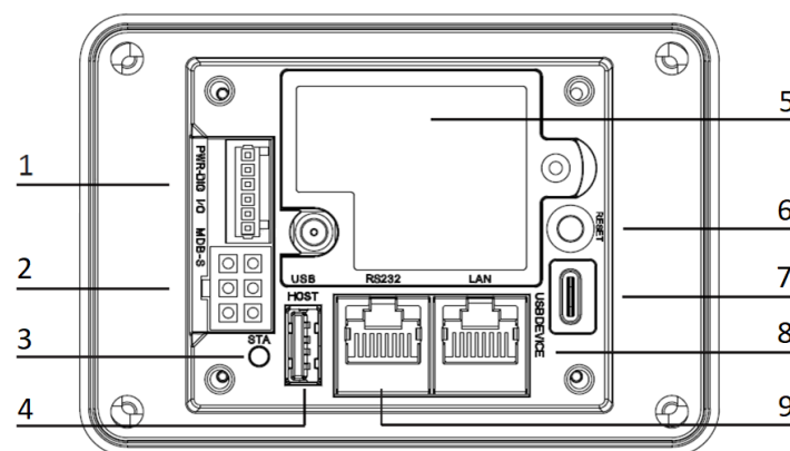
Figure 2: back view
