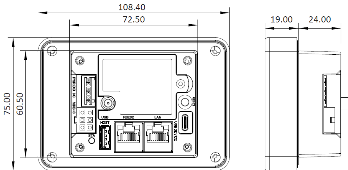
Figure 5: device dimensions (mm)
