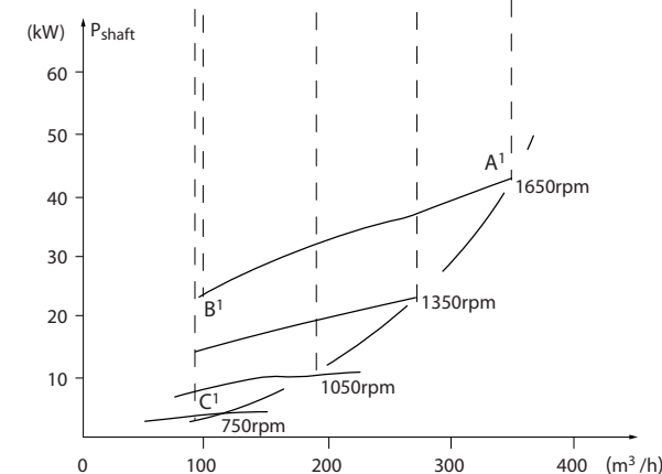
Illustration 4.10 Pump Performance
