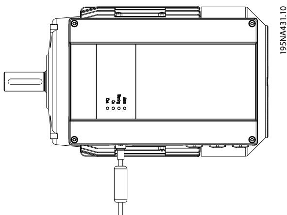
Illustration 3.3 Remote Mounting Kit Connections
