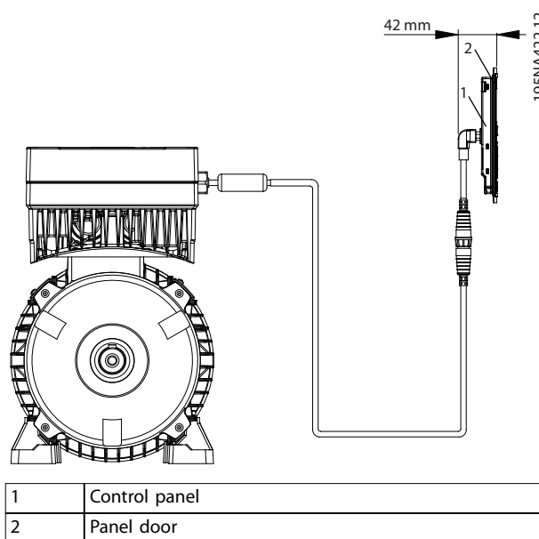
Illustration 3.5 LCP Remote Mounting
