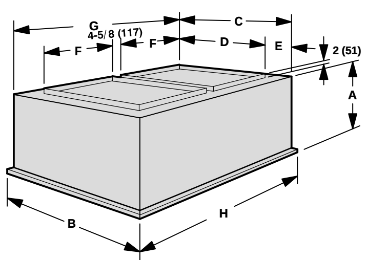
FD11-185 & FD11-275 FLUSH CEILING DIFFUSER
