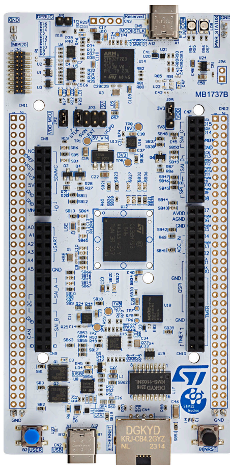
Figure 1. NUCLEO-H7S3L8 top view
