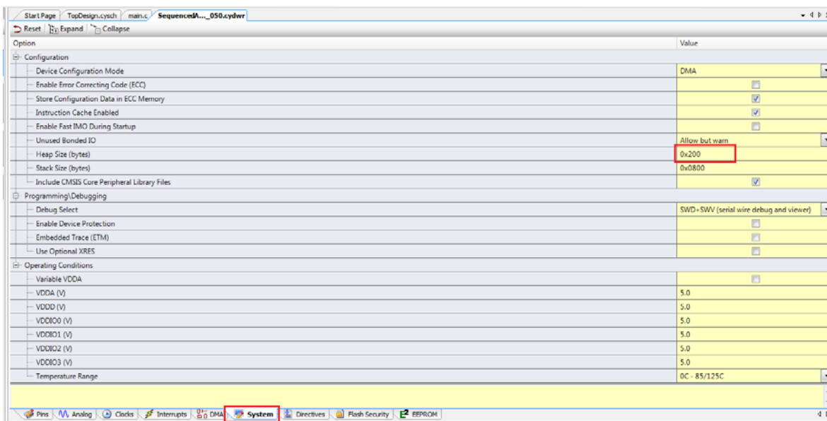
Figure 5-2. System Tab
