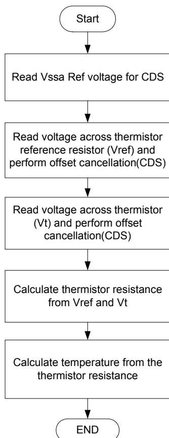
Figure 5-9. Thermistor Flowchart
