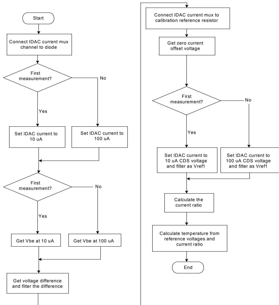
Figure 5-11. Diode Flowchart
