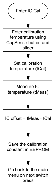
Figure 5-14. IC Calibration
