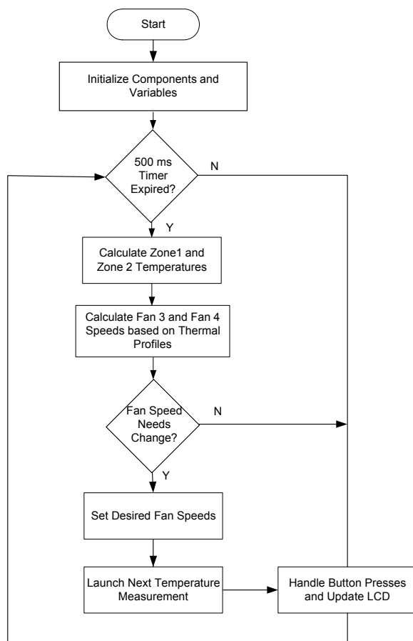
Figure 5-42. Thermal Manager Flowchart
