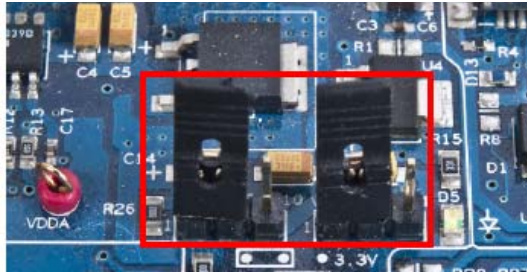
Figure 5-24. CY8CKIT-030 PSoC 3 DVK Power Jumpers
