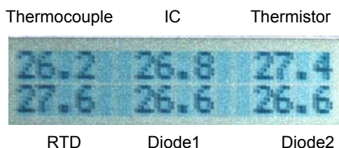
Figure 5-4. Simultaneous Temperature Display for All Six Sensors
