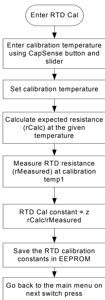
Figure 5-12. RTD Calibration
