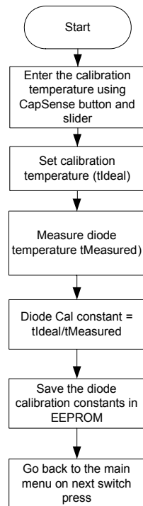
Figure 5-13. Diode Calibration
