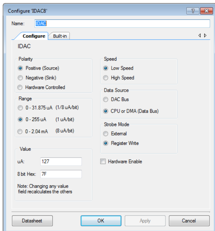
Figure 5-41. IDAC Configuration
