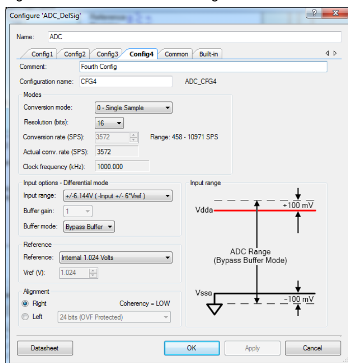
Figure 5-19. \pm 6.144 V ADC Configuration
