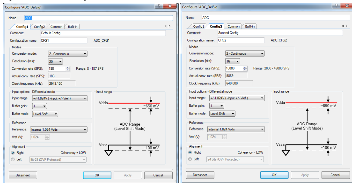
Figure 5-6. ADC Configuration
