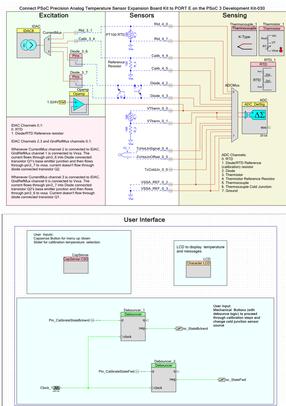
Figure 5-5. PSoC Creator Top Design
