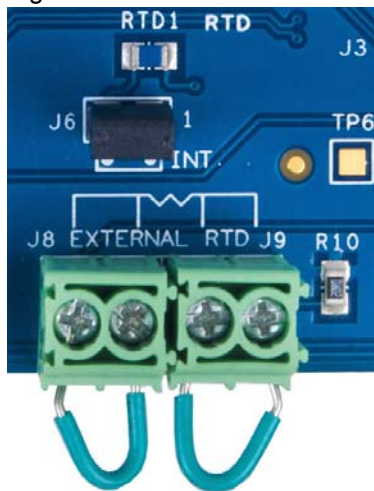
Figure 3-7. RTD
