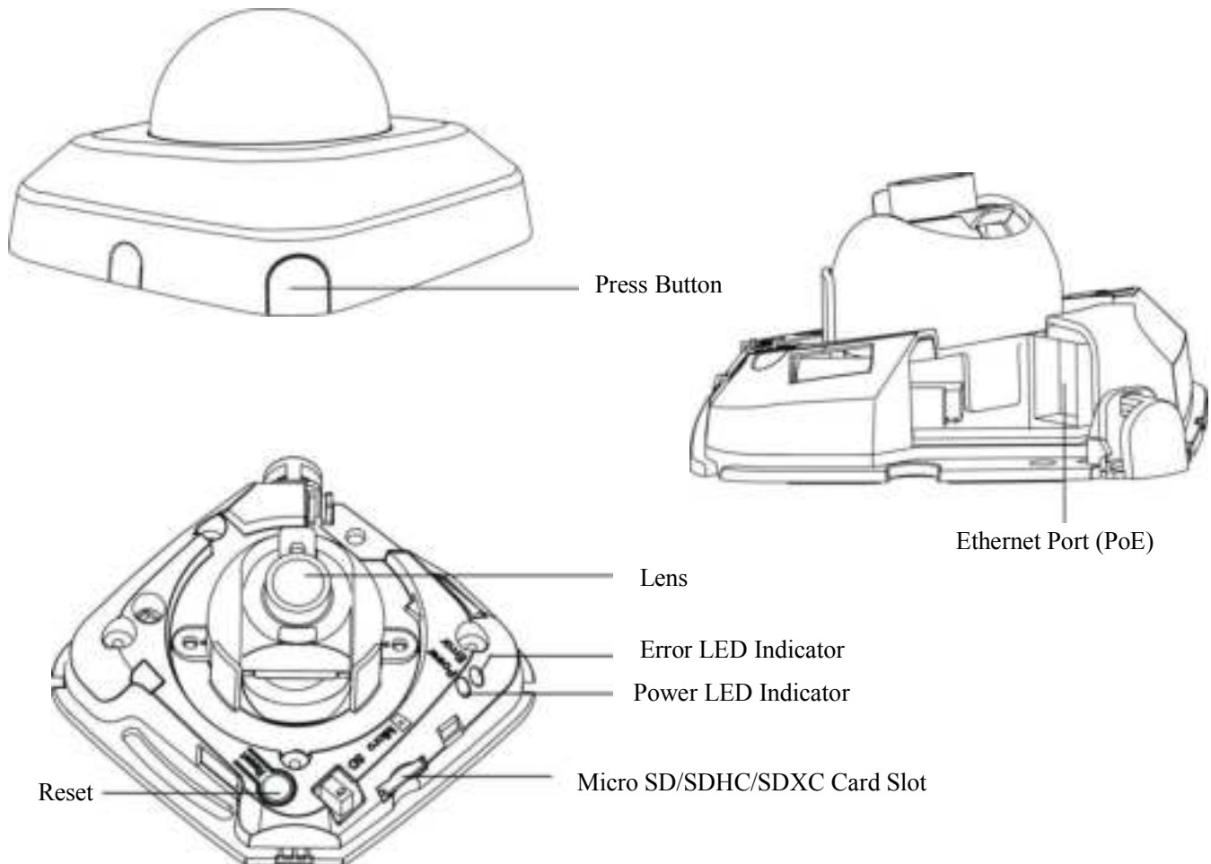
Figure 1-3-1 Mini Dome Network Camera
