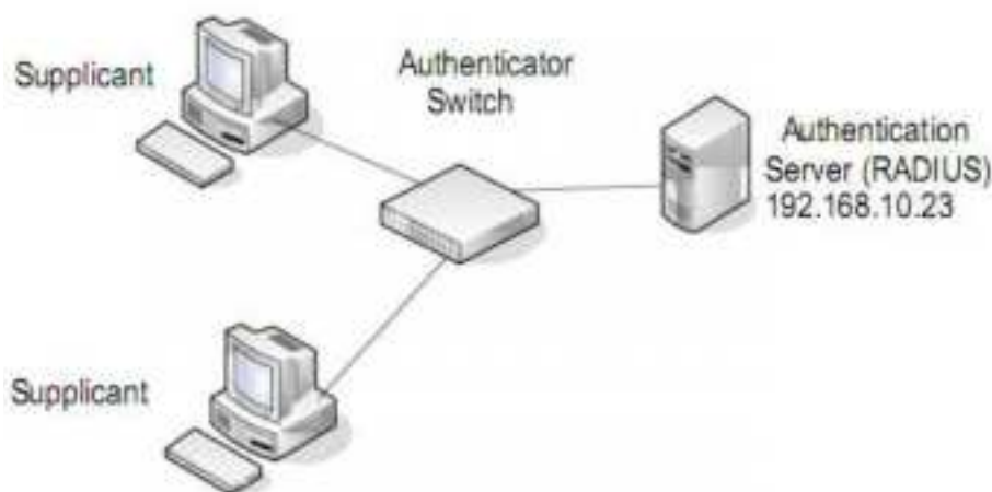
Figure 1. 802.1X authentication roles
