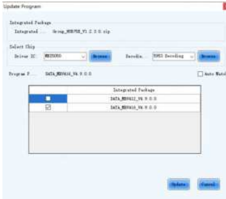
Fig4-16
