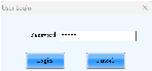
Fig 4-4 User Login
