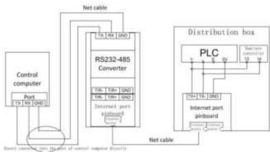
Fig 2-26 Distribution Box PLC Connection Diagram
