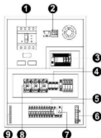
Fig 2-25 Internal Structure of Distribution Box
