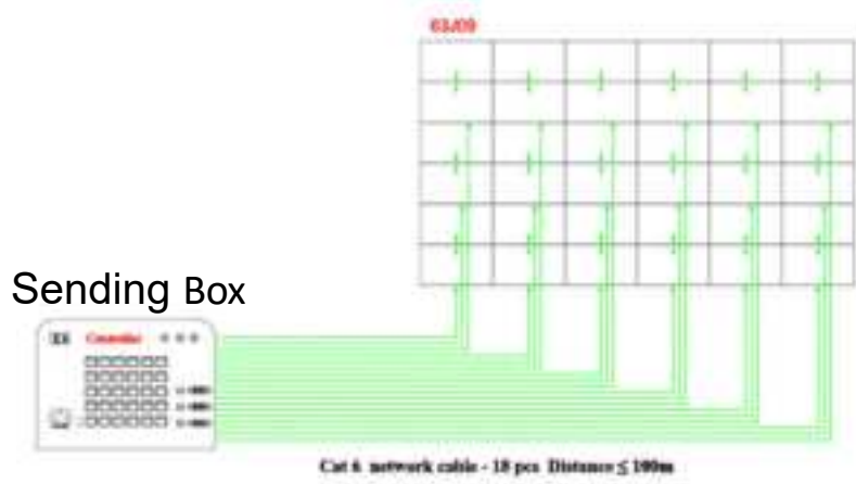
Fig 2-21 Signal Cable Connection Diagram of P0.9
