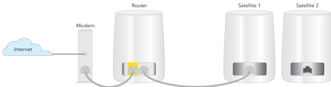
Figure 4. Star topology: Satellite connected to the router's Ethernet port
