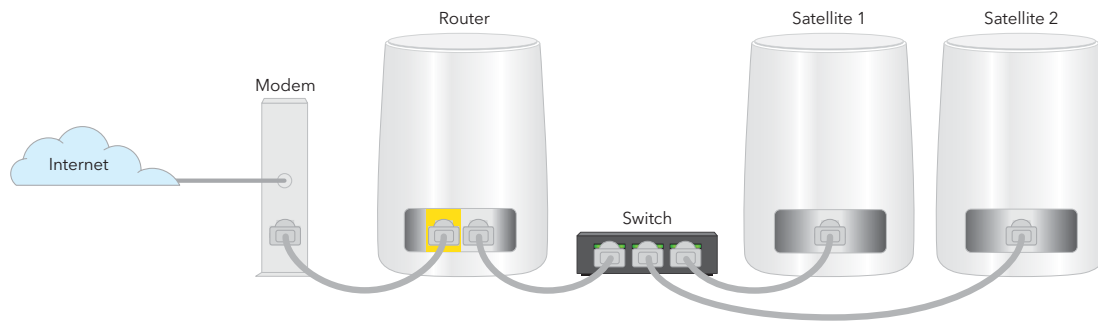
Figure 6. Ethernet backhaul connection using a switch
