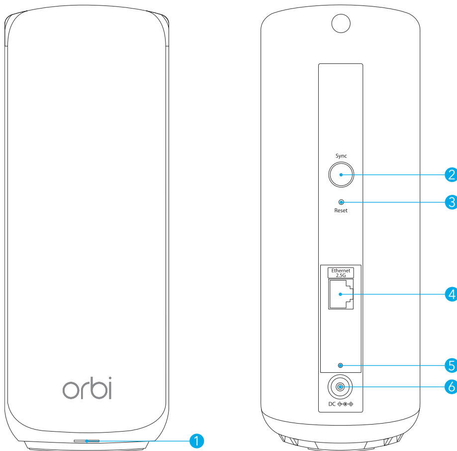
Figure 2. Orbi satellite front (left figure) and back (right figure) views
