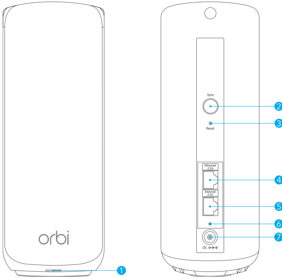
Figure 1. Orbi router front (left figure) and back (right figure) views
