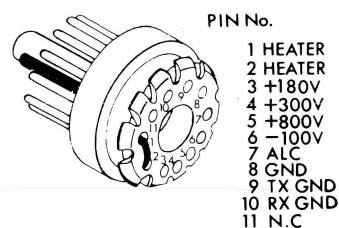
ACC plug
